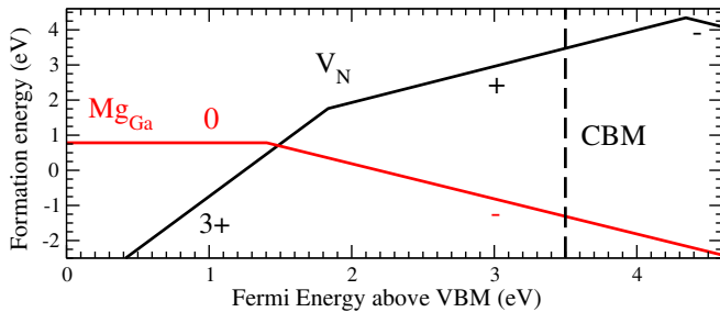
FIG. 2 (color online). Formation energy of V_N (black line) and \text{Mg}_{\text{Ga}} [light gray (red) line] as a function of Fermi energy above the VBM. Anion-rich conditions are assumed. The position of the conduction band minimum (CBM) is indicated by the broken line. For each value of Fermi energy, only the most stable defect charge state is shown, with a change in slope indicating a change in charge state.
