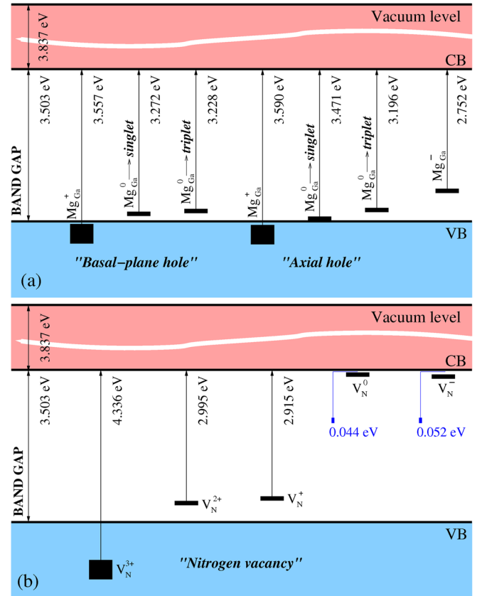
FIG. 3 (color online). Calculated vertical ionization levels of (a) \text{Mg}_{\text{Ga}} and (b) V_N in the relevant charge states, shown relative to the valence band (VB), conduction band (CB), and vacuum level. In (a) the two hole configuration cases, consisting of localization on a N either in the basal plane or along the c axis, are shown. For the neutral state, ionization to either singlet or triplet states is included. The large black boxes indicate resonance states in the VB.
