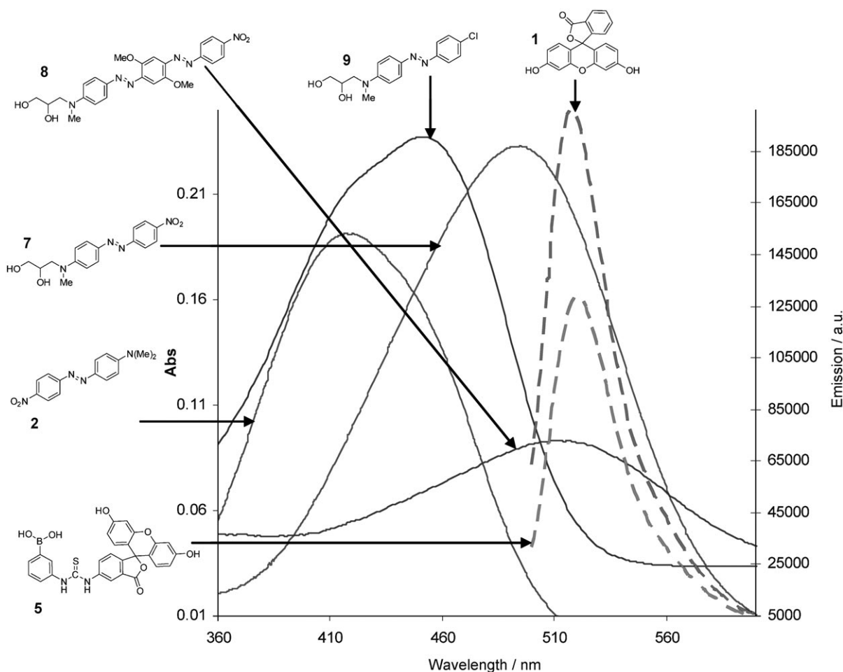
Figure 2. Absorbance (continuous lines) spectra of 2 , 7 , 8 , and 9 and emission (dotted lines) spectra of 1 and 5 ( \lambda_{\text{ex}} = 490 \text{ nm} ).
