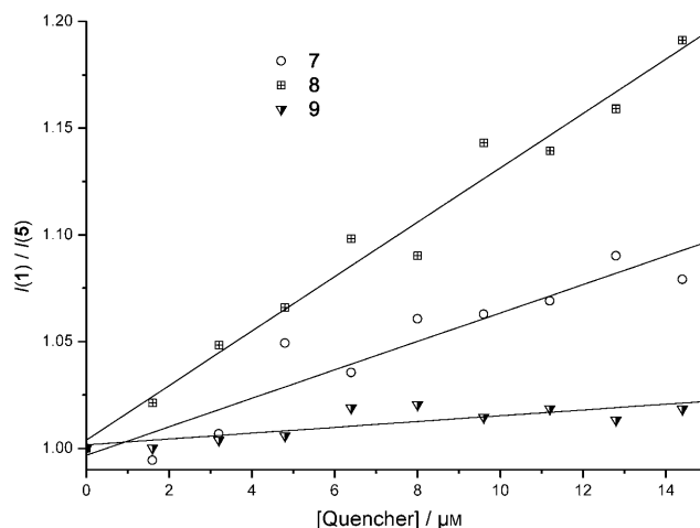
Figure 5. The enhancement in quenching as a result of the presence of a boronic acid in the fluorophore ( I_0/I for 5 )/( I_0/I for 1 ) (represented as I(1)/I(5) ), at 0.0135 \mu\text{M} , for the addition of diol appended quenchers 7 , 8 , and 9 .
