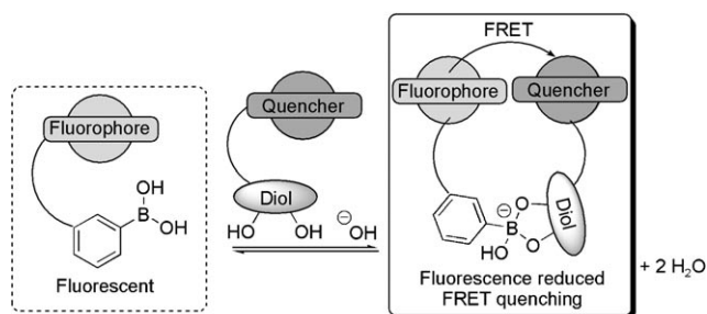
Scheme 2. Schematic representation of boronate ester formation resulting in an enhanced (static) FRET quenching.
