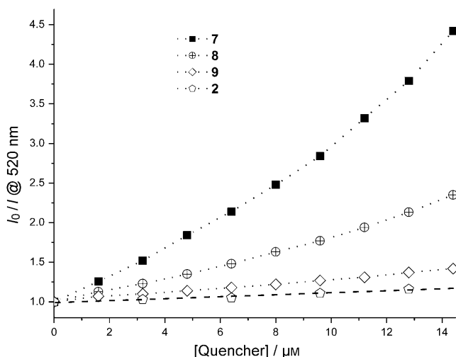
Figure 4. Comparison of relative quenching action observed on 5 ( 0.0135 \mu\text{M} ) ( I_0/I ) upon addition of non-diol appended 2 and diol bearing units 7 , 8 , and 9 at 520 nm ( \lambda_{\text{ex}} = 490 nm).
