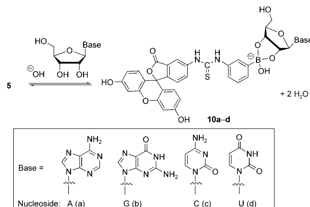
Scheme 6. Formation of 10 a–d upon the addition of nucleosides adenosine A (a), guanosine G (b), cytidine C (c), and uridine U (d) to 5 .
