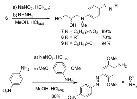
Scheme 5. Synthesis of diol appended quenchers 7 , 8 , and 9 and preparation of intermediate to 8 ( R^1-NH_2 ).
