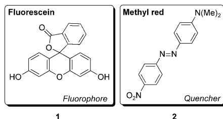
Figure 1. Structures of fluorescein 1 and methyl red 2 .
