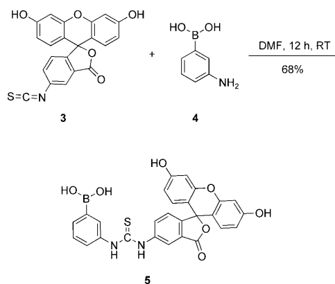
Scheme 3. Preparation of fluorescein boronic acid 5 .
