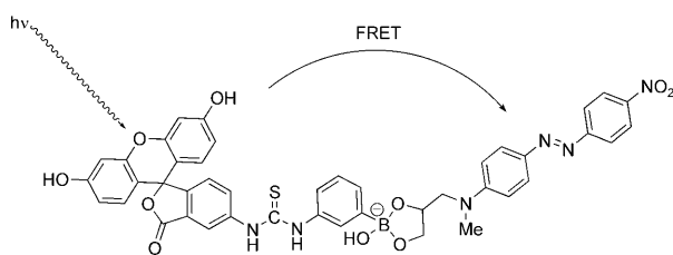
Figure 3. Proposed structure and FRET quenching mechanism of a boronate ester formed upon reaction of 5 with 7 .
