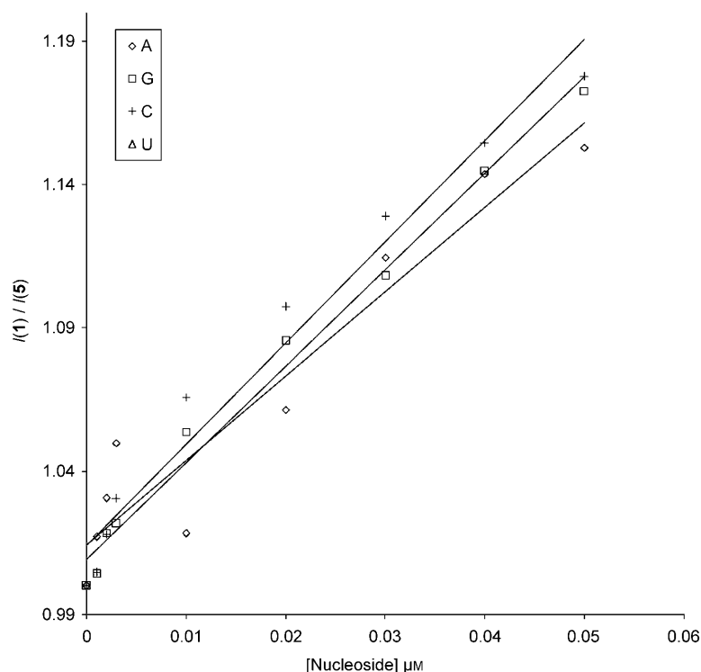
Figure 7. Plot ratiometrically comparing quenching ability of nucleosides on boronic acid appended quencher 5 as a percentage enhancement over that with fluorescein 1 .
