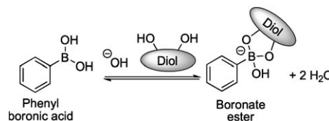
Scheme 1. Generic phenylboronate ester formation.
