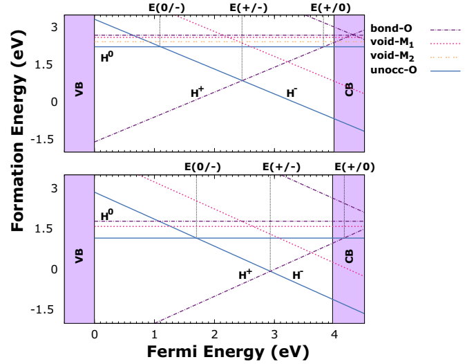
FIG. 6. Formation energy of the different hydrogen configurations as a function of the Fermi-level position. The range of E_F corresponds to the bulk theoretical band gap with E_F = 0 aligned at the valence-band maximum. The formation energies of the different geometrical configurations are represented by different line types and colors. The upper plot represents the results obtained by employing the PBE exchange-correlation functional, where the f electrons were treated as corelike states. The lower plot represents the results obtained from DFT+ U with the f electrons treated as valence states. The thermodynamic charge-transition (electrical) levels are marked by the vertical lines.
