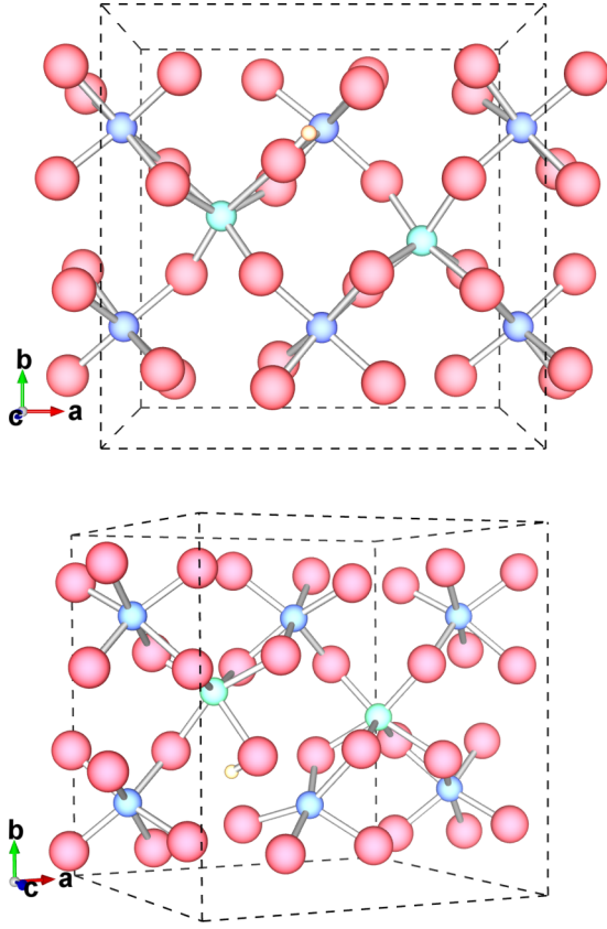
FIG. 5. DFT+ U bond-O configurations of the H impurity for the H^0 (top) and H^- (bottom) charge states. The stable configuration for the H^+ system is similar to the H^- state. The presented structures are the representative lowest-energy bond-O configurations.
