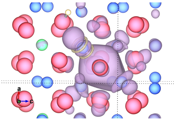
FIG. 11. DFT + U isosurfaces of the electron charge densities for the neutral state of the representative, lowest energy, bond-O configuration. The atoms are represented by their ionic radius, where O is depicted in red, Lu in blue/green, and hydrogen in yellow. The purple color of the isosurface refers to positive values and the yellow to negative values.
