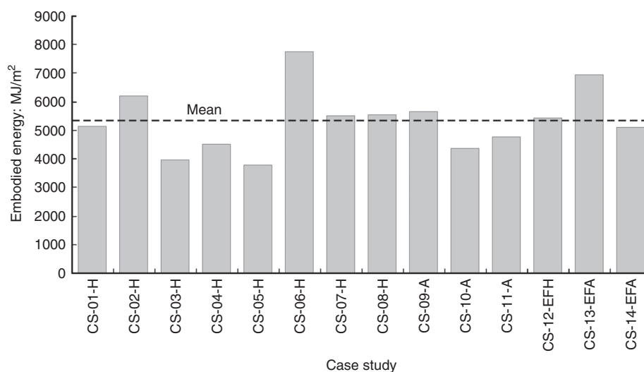
Fig. 6. Embodied energy of 14 case studies (Table 3)
