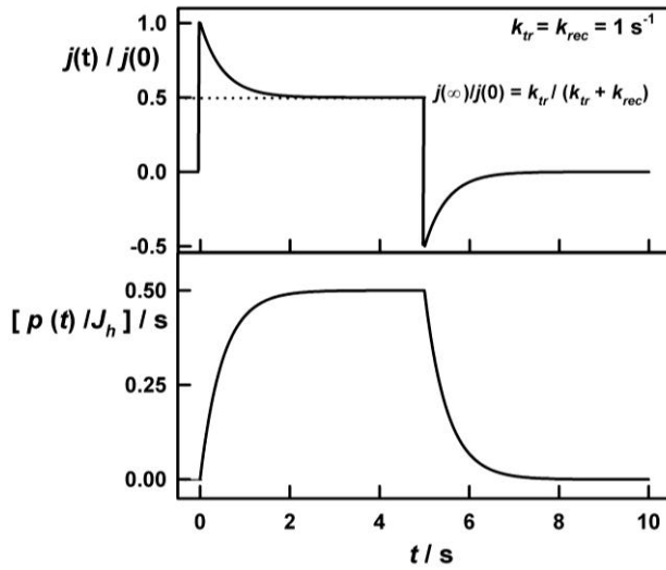
Figure 8. The upper plot shows a normalized photocurrent transient calculated for k_{tr} = k_{rec} = 1 \text{ s}^{-1} . Note that the steady state photocurrent j(\infty) is determined by the competition between charge transfer and recombination, and the decay time constant is determined by (k_{tr} + k_{rec})^{-1} . Analysis of experimental transients allows the values of k_{tr} and k_{rec} to be determined. The lower plot shows the corresponding build up and decay of the surface hole concentration p(t) normalized by dividing by the hole flux J_h into the surface.
