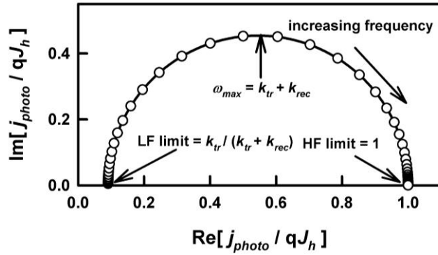
Figure 9. Normalized IMPS response showing high frequency (HF) and low frequency (LF) intercepts and maximum of the semicircle. Calculated for k_{rec} = 10k_{tr} .
