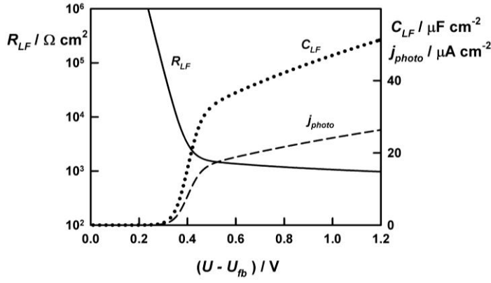
Figure 14. Potential dependence of R_{LF} and C_{LF} calculated from eqn. 14 using values of J_h and k_{rec} calculated using eqn. 9 and eqn. 8 respectively. Other values used in the calculation: k_t = 20 \text{ s}^{-1} , \alpha = 1.5 \times 10^5 \text{ cm}^{-1} , N_d = 10^{19} \text{ cm}^{-3} , \varepsilon = 25 , C_H = 100 \text{ μF cm}^{-2} , \sigma_p = 10^{-16} \text{ cm}^2 , v_{th} = 10^5 \text{ cm s}^{-1} , I_0 = 2 \times 10^{15} \text{ cm}^{-2} \text{ s}^{-1} .
