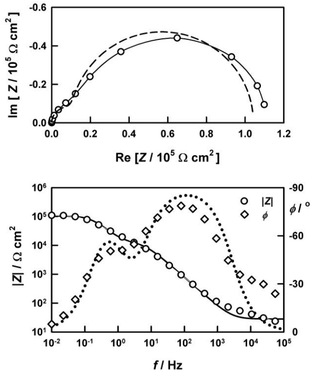
Figure 13. Typical experimental PEIS response for a thin film hematite photoanode. Electrolyte 1. NaOH. Potential 0.1 V vs. Ag|AgCl. Illumination 455 nm, ca.1 mW cm -2 .
