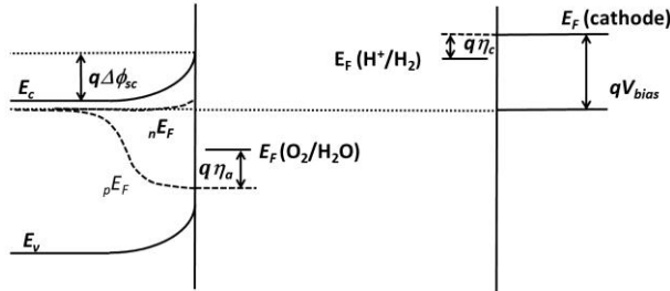
Figure 2. Splitting of the quasi Fermi levels for an illuminated n-type semiconductor such as hematite biased into depletion (band bending = q\Delta\phi_{sc} ). The difference between pE_F and E_F(\text{O}_2/\text{H}_2\text{O}) defines the overpotential \eta_a for the oxygen evolution reaction. In the case shown here, \eta_a is large due the accumulation of holes at the interface as a consequence of sluggish electron transfer kinetics. As shown below, pE_F may be displaced into the valence band if the rate constant for charge transfer is sufficiently slow. In order to achieve water splitting, an additional bias voltage is required to raise the Fermi level of the metal cathode above E_F(\text{H}^+/\text{H}_2) . In the figure, the overpotential for the cathodic reaction, \eta_c is exaggerated for clarity. If catalytic electrodes like platinum are used, the cathodic overpotential will be much smaller.
