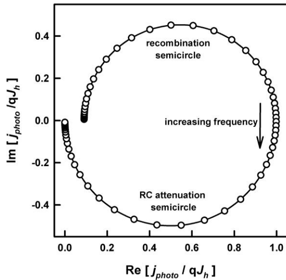
Figure 10. Complete IMPS response including the effects of RC attenuation at high frequencies. Provided that the RC time constant is much shorter than (k_{tr} + k_{rec})^{-1} , the upper semicircle can be used to derive the two rate constants.
