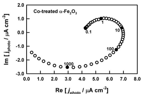
Figure 11. Experimental IMPS response measured for a thin film \alpha\text{-Fe}_2\text{O}_3 electrode in the photocurrent onset region. The electrode was treated with a drop of 10mM cobalt nitrate solution. Electrolyte 1.0 M NaOH. Electrode potential -0.3 V vs. \text{Ag}|\text{AgCl} . Illumination 455 nm, dc photon flux 1.1 \times 10^{17} \text{ cm}^{-2} \text{ s}^{-1} .
