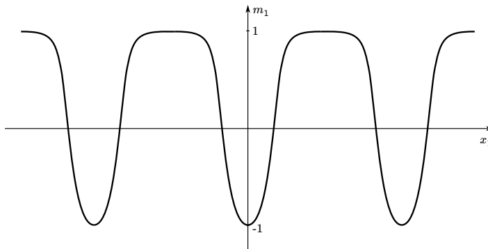
Figure 2: For h = 1 , an array of Néel walls of total winding number 3, represented in terms of m_1 .
