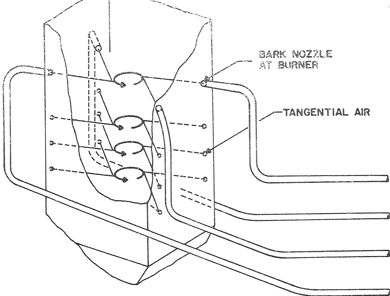
Figure 3-13.—Schematic of a suspension firing system used in large boilers. (Drawing after Fernandes 1976.)
