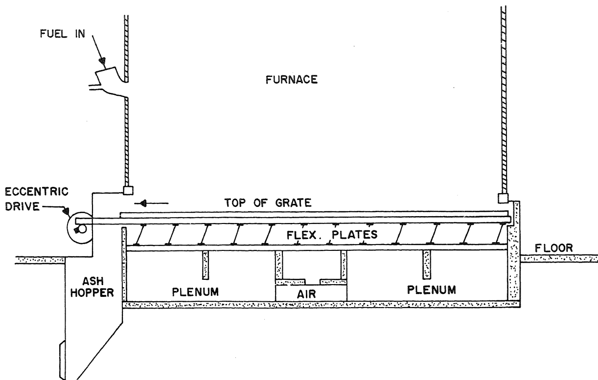
Figure 3-11. — Vibrating grate stoker. (Drawing after Fuller 1976.)
