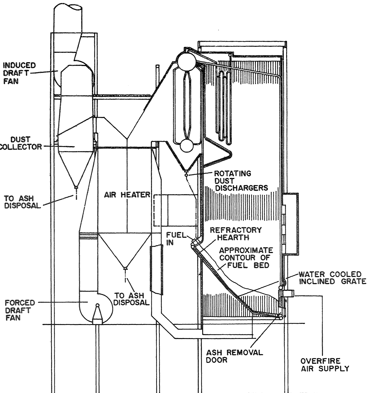
Figure 3-8.—Inclined grate furnace system. (Drawing after Corder 1973.)
