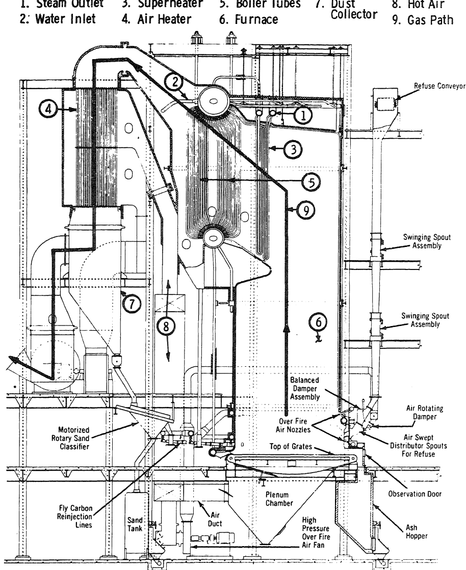
SIDE SECTION
