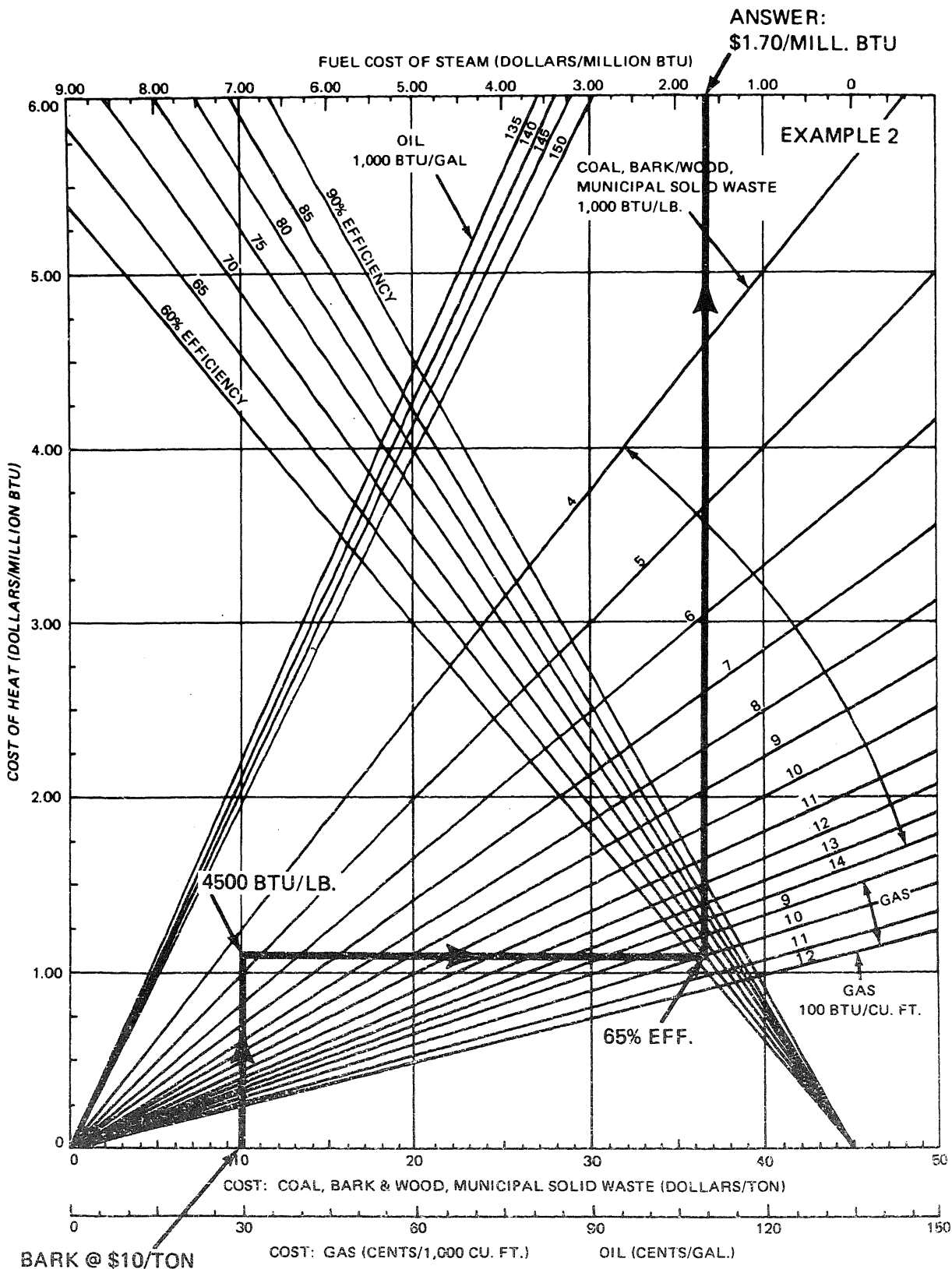
Figure 3-4. --Example of how to use the fuel value comparison graph. (Drawing after Arola 1975.)
