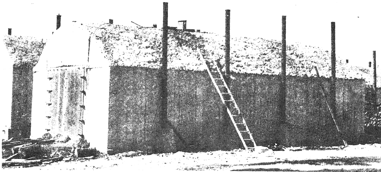
Figure 5-2.—Missouri-type batch kiln. (Photo courtesy of Bob Massengale, Missouri Department of Conservation.)
