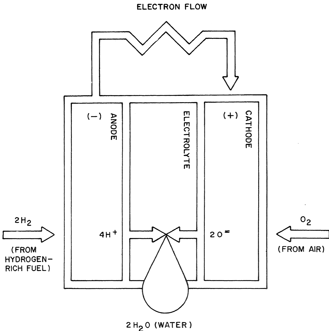
Figure 4-4.— The basic principles of fuel cell operation (Energy Research and Development Administration 1976). The fuel cell consists of an anode, cathode, and electrolyte much as in a battery. Hydrogen rich fuel is fed down the anode side of the cell. Here the hydrogen leaves its electrons giving the anode a negative charge. Air enters the fuel cell on the cathode side. Here oxygen accepts electrons from the cell giving the cathode a positive charge. Electrical power is generated by the flow of electrons from the anode to the cathode. Hydrogen ions formed at the anode and oxygen ions formed at the cathode migrate through the electrolyte to combine and form water. Heat is also liberated in the process. The overall simplified process is shown in equation 4-1. (Drawing from Department of Energy.)
