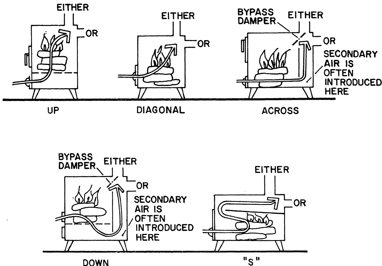
Figure 3-20.—The five basic air flow patterns found in domestic stoves. Stoves with both the across- and down-draft flow patterns usually require a bypass damper to prevent smoke from entering the room when the stove door is opened. (Drawing after Lew 6 )
