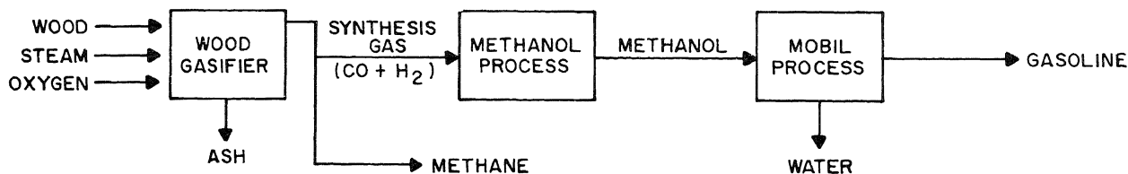
Figure 4-5.—Overall scheme for the production of gasoline from wood. Selling the methane produced in the gasification step instead of reconverting it into synthesis gas would lower the cost of methanol production. (Drawing after Meisel et al. 1976.)
