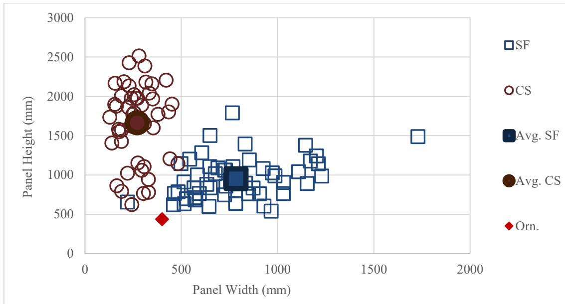
Figure 5. Dimensions of 100 representative sample infill panels. Square Framed (SF), Close Studded (CS), Ornamental (Orn).
