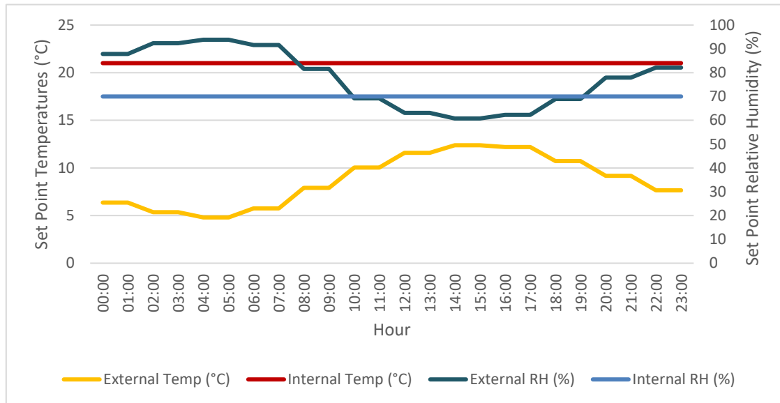
Figure 10. Set points for cyclical conditions for internal and external climate-controlled chambers. twenty-four-hour pattern repeated 14 times over two week period.
