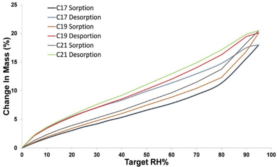
Figure 6. Sorption and desorption isotherms for three samples of oak felled in different centuries.
