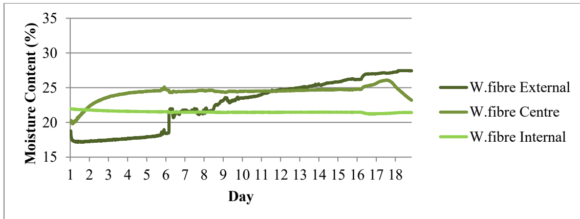
Figure 13. Interstitial moisture content (%) measured in Woodfibre and Woodwool panel from 14/09/2017 to 02/10/2017 under steady state conditions.
