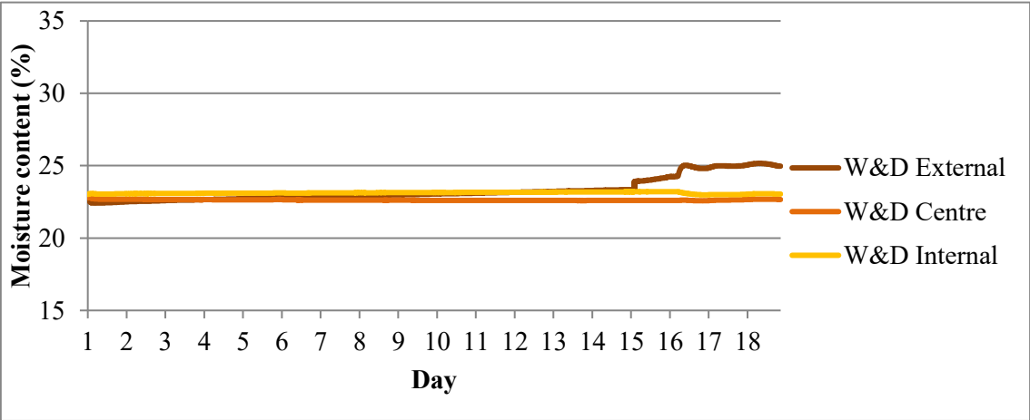
Figure 11. Interstitial moisture content (%) measured in Wattle & Daub (W&D) panel from 14/09/2017 to 02/10/2017 under steady state conditions.
