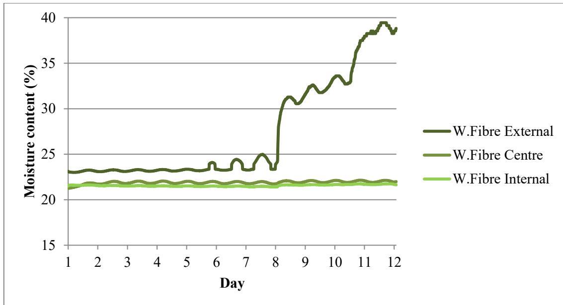
Figure 16. Interstitial moisture content (%) measured in Woodfibre and Woodwool panel from 02/10/2017 to 13/10/2017 under dynamic conditions.
