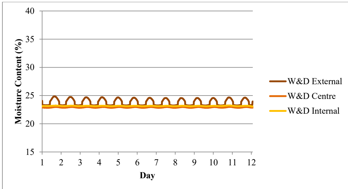
Figure 14. Interstitial moisture content (%) measured in Wattle & Daub (W&D) panel from 02/10/2017 to 13/10/2017 under dynamic conditions.
