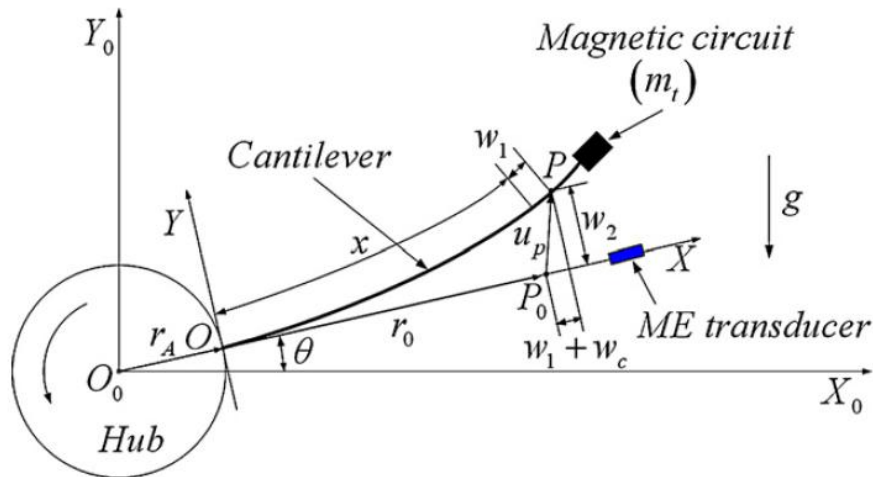
Figure 12. Schematic illustration of frequency-tunable energy harvester [71] with permission from Elsevier.
