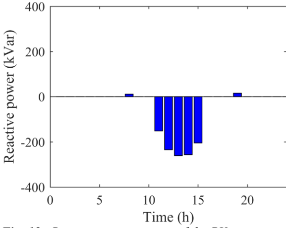
Fig. 12. Reactive output power of the PV inverter at node 18.
