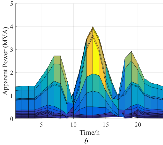
Fig. 10. Branch apparent power profiles in 3-D and its projection on the Time- Apparent power plane. (a). Figure in 3-D (b). Projection on the Time- Apparent power plane
