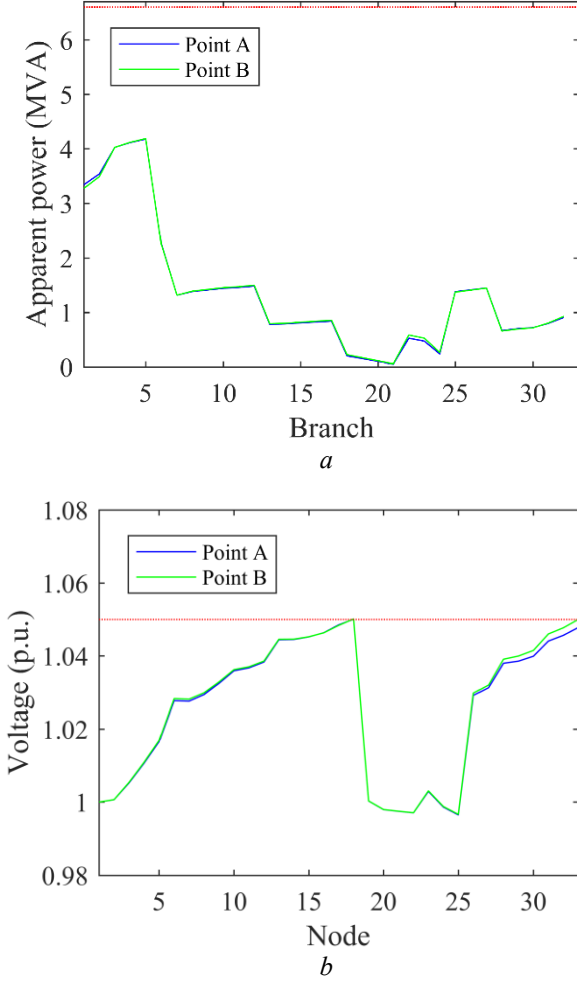
Fig. 9. Branch flow and Node voltage at point A and B (a). Branch flow (b). Node voltage
