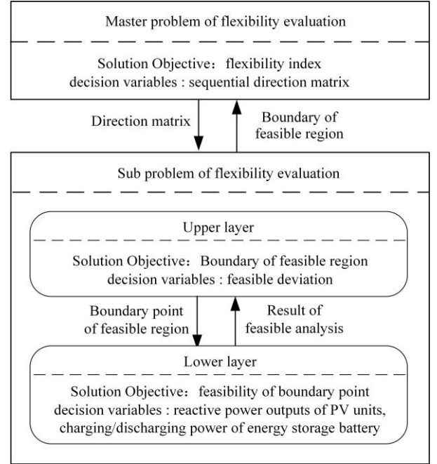
Fig. 2. The proposed approach for flexibility evaluation
