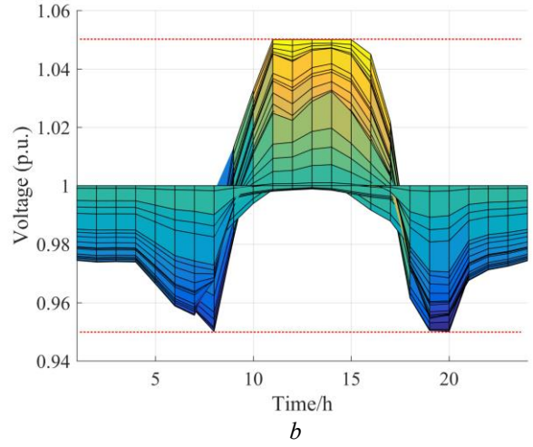
Fig. 11. Voltage profiles in 3-D and its projection on the Time-Voltage plane. (a). Figure in 3-D (b). Projection on the Time-Voltage plane
