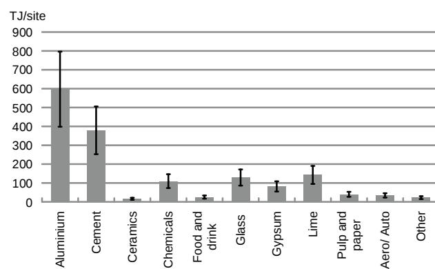
Figure 4 Annual heat recovery per site.
