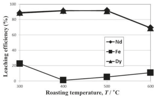
Figure 5. The effect of roasting temperature on the leaching efficiency (Grinding conditions: 550 rpm in rotational speed, 5 cm 3 in water addition, 30 min in grinding time, 15 in stoichiometric molar ratio).
