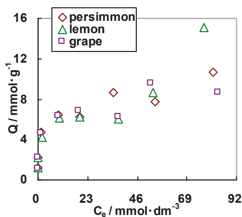
Figure 26. Adsorption isotherms of gold(III) from 1\text{ mol}\cdot\text{dm}^{-3} hydrochloric acid solution on the adsorption gels prepared from peels of persimmon, lemon and grape treated in boiling concentrated sulfuric acid [34] (with permission for reuse from Elsevier B.V.).
