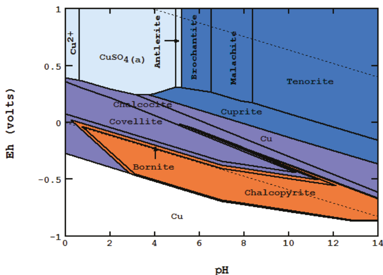
Figure 4. Eh-pH diagram Cu-CO 2 -Fe-S in water. p\text{CO}_2 = 0.1 \text{ atm} , [\text{S}] = 0.01 \text{ M} , [\text{Fe}] = [\text{Cu}] = 0.001 \text{ M} . Species were taken from the LLnL database [11].
