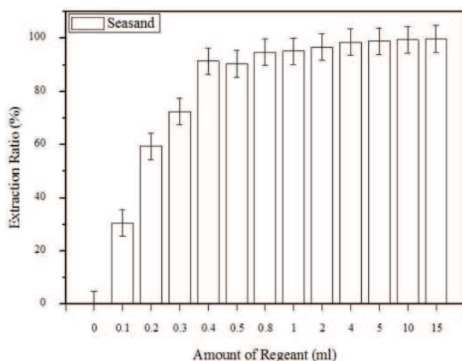
Figure 4. Extracted fraction of uranium as a function of the amount of extraction reagent used (specimen: sea sand with 50 \mu\text{g-U/g} , uncertainty applied: 5%).
