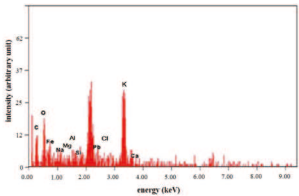
Figure 6. SEM/EDX results from in-house potassium ferrate.
