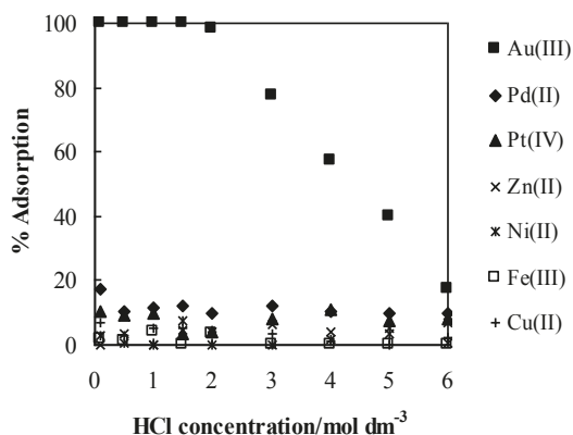
Figure 19. Percentage adsorption of various metal ions on crude PT powder as a function of concentration of hydrochloric acid [33] (with permission for reuse from Elsevier B.V.).
