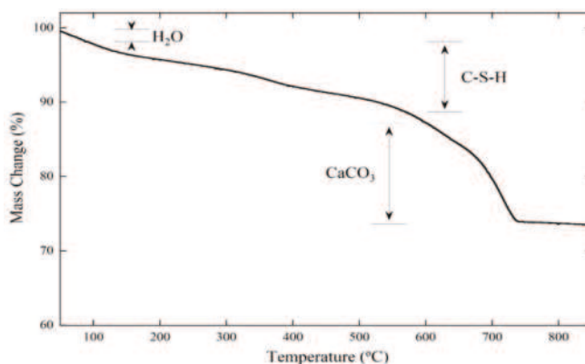
Figure 2. Thermogravimetric analysis (TGA) results of as-received waste slate. “H 2 O”, “C–S–H”, and “CaCO 3 ” indicate the mass change occurred by the decomposition of H 2 O, C–S–H, and CaCO 3 , respectively.
