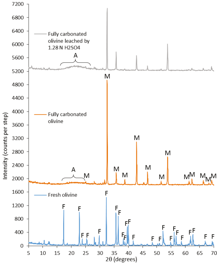
Figure 1. XRD diffractograms of fresh olivine, fully carbonated olivine and fully carbonated olivine after leaching in 1.28 N H 2 SO 4 for 24 h; major mineral peaks are indicated: F = ferroan-forsterite ((Mg,Fe) 2 SiO 4 ); M = magnesite/ferro-magnesite ((Mg 1-x ,Fe x )CO 3 ); A = quasi-amorphous phase.
