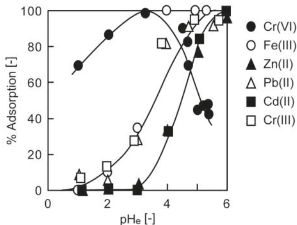
Figure 8. Effect of equilibrium pH on the adsorption of different metal ions on CPW gel [23] (with permission for reuse from Elsevier B.V.).
