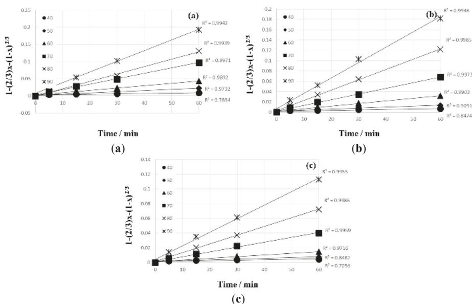
Figure 6. Plot of 1 - 2/3x - (1 - x)^{2/3} vs. T for different temperatures ( [\text{Fe}^{3+}] : (a) 1.0 M; (b) 0.5 M; (c) 0.25 M; 10% pulp density; 400 rpm agitation speed).
