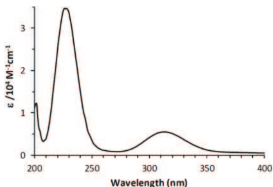
Figure 2. UV-Vis spectrum of \text{HAuCl}_4 in 0.1 M aqueous HCl.
