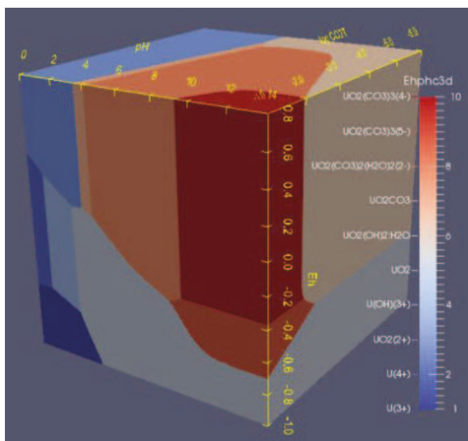
Figure 27. Eh-pH- \log \Sigma CO_2 of uranium where the species are shown by colors. A color bar is inserted to show the corresponding species.
