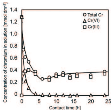
Figure 10. Time variation of the concentrations of chromium(VI) and chromium(III) as well as total chromium in the aqueous solution at pH = 1 during adsorption [23] (with permission for reuse from Elsevier B.V.).
