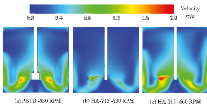
Figure 4. Flow field contours in a stirred tank generated by PBTD and HA-715.
