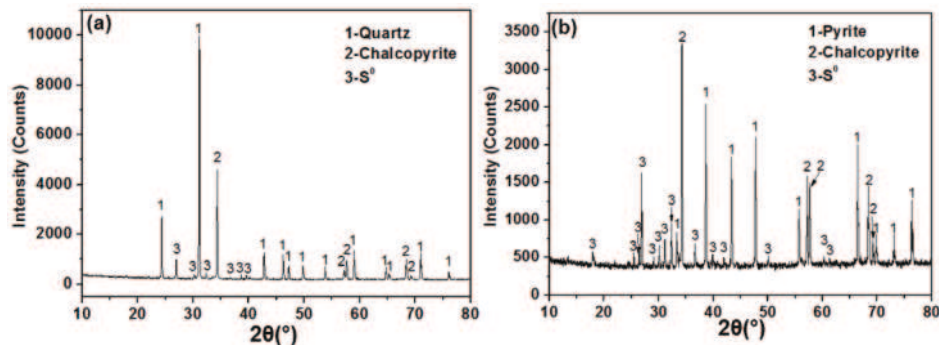
Figure 2. XRD patterns from the chalcopyrite leach residue subjected to 750 mV, 75 °C and pH 1.0: (a) chalcopyrite and quartz; (b) chalcopyrite and pyrite.
