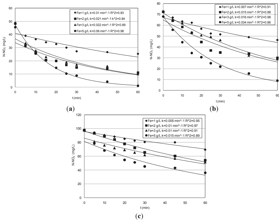
Figure 4. Trends of nitrate concentrations detected during the tests conducted at uncontrolled pH: (a) N_i = 50 \text{ mg/L} ; (b) 70 \text{ mg/L} ; (c) 95 \text{ mg/L} .
