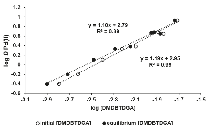
Figure 5. Dependence of the Pd(II) log D values on the log of the initial and equilibrium DMDBTDGA concentrations ( 9.4 \times 10^{-4} M Pd(II) in 4.5 M HCl; 1.6 \times 10^{-3} to 2.0 \times 10^{-2} M DMDBTDGA in toluene; A/O = 1, room temperature, 900–1000 rpm). Standard deviations: \pm 5\% .
