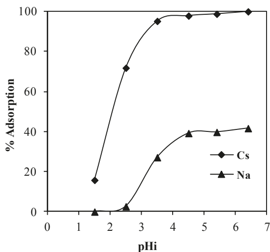
Figure 5. Percentage adsorption of cesium(I) and sodium(I) ions on crosslinked persimmon tannin (CPT) gel at varying initial pH [17] (with permission for reuse from Elsevier B.V.).
