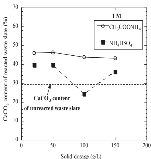
Figure 7. \text{CaCO}_3 content of reacted waste slate samples determined using TGA as a function of the solid dosage with the 1.0 M \text{CH}_3\text{COONH}_4 and \text{NH}_4\text{HSO}_4 solutions.
