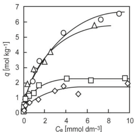
Figure 11. Adsorption isotherms of chromium(VI) on CPW gel [23] (with permission for reuse from Elsevier B.V.). \circ pH 1, \Delta pH 2, \square pH 3, \diamond pH 4.
