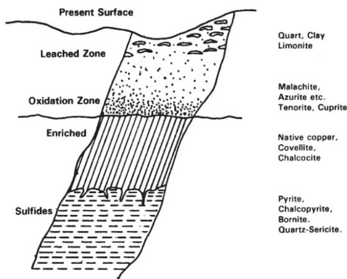
Figure 3. Illustrated copper ore deposit for comparison to the Eh-pH diagram to the right (Dudas et al. [10]).
