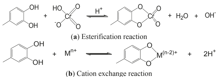
Scheme 2. The binding mechanism of (a) chromium(VI) and (b) other metals to the hydroxyl groups of catechol units on the cross-linked persimmon gel.
