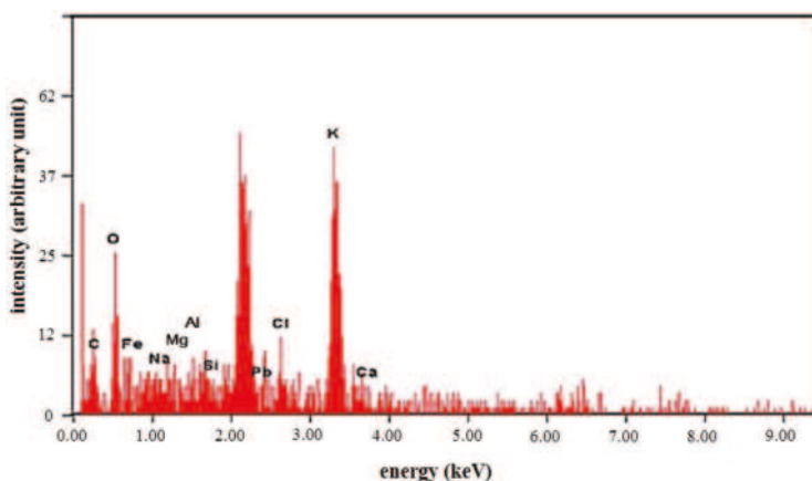
Figure 5. SEM/EDX results from as-purchase potassium ferrate.
