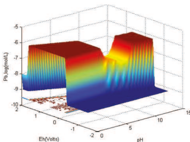
Figure 23. The Eh-pH plus solubility diagram for Pb- \text{CO}_3 -water. The yellow gulch area in the middle is where Pb(II) is likely passivated by \text{CO}_3 .
