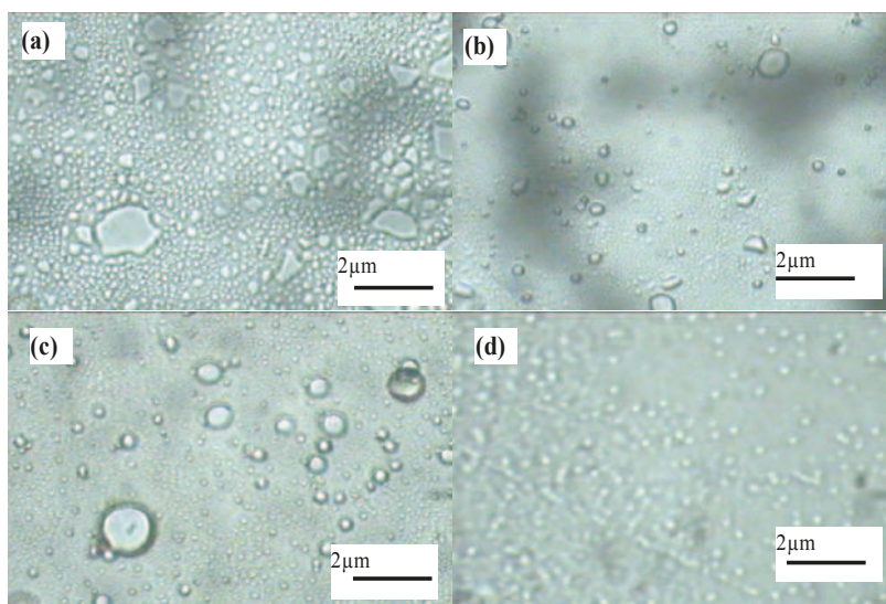
Figure 1. Photographic of ELM droplets formed under different stirring times. (Membrane phase: 6% v/v LIX 7950, 2% v/v 1-dodecanol, 5% v/v Span 80, 1% v/v paraffin, balanced with kerosene; Internal stripping solution: 0.1 mol/L KOH; Volume ratio of the membrane phase to the internal phase: 1:1; Mixing speed: 4500 RPM; Mixing time: (a) 5 min; (b) 15 min; (c) 25 min; (d) 35 min).
