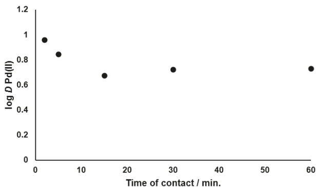
Figure 4. Variation of the log D values of Pd(II) with the contact time ( 9.4 \times 10^{-4} M Pd(II) in 4.5 M HCl; 0.02 M DMDBTDGA in toluene; A/O = 1, room temperature, 900–1000 rpm). Standard deviations: \pm 8\% .
