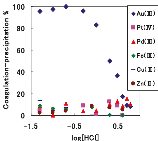
Figure 16. Percentage recovery of various metal ions by means of coagulation using persimmon extract liquor from varying concentration ( \text{mol}\cdot\text{dm}^{-3} ) of hydrochloric acid solution [32] (with permission for reuse from The Society of Chemical Engineers of Japan).
