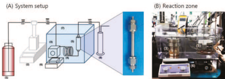
Figure 3. Experiment setup and the reaction zone for uranium extraction from the contaminated sand: (1) \text{CO}_2 cylinder; (2) syringe pump; (3) mixing cell; (4) preheating cell; (5) specimen; (6) mixer; (7) thermostat; and (8) collector.
