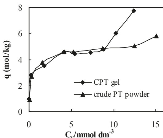
Figure 20. Adsorption isotherms of gold(III) on CPT gel and crude persimmon extract tannin (PT) powder from 0.1 mol·dm -3 hydrochloric acid solution [33] (with permission for reuse from Elsevier B.V.).
