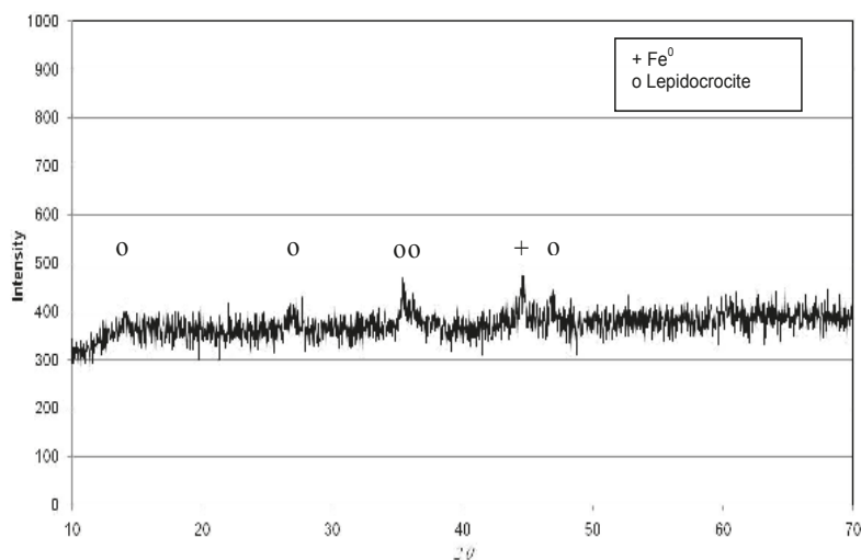
Figure 6. XRD of iron corrosion product after the tests conducted with \text{Fe}^0 = 3 \text{ g/L} , N_i = 50 \text{ mg/L} and uncontrolled pH.
