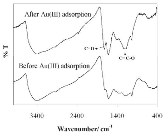
Figure 21. FT-IR spectra of CPT gel before and after the adsorption of gold(III) [33] (with permission for reuse from Elsevier B.V.).
