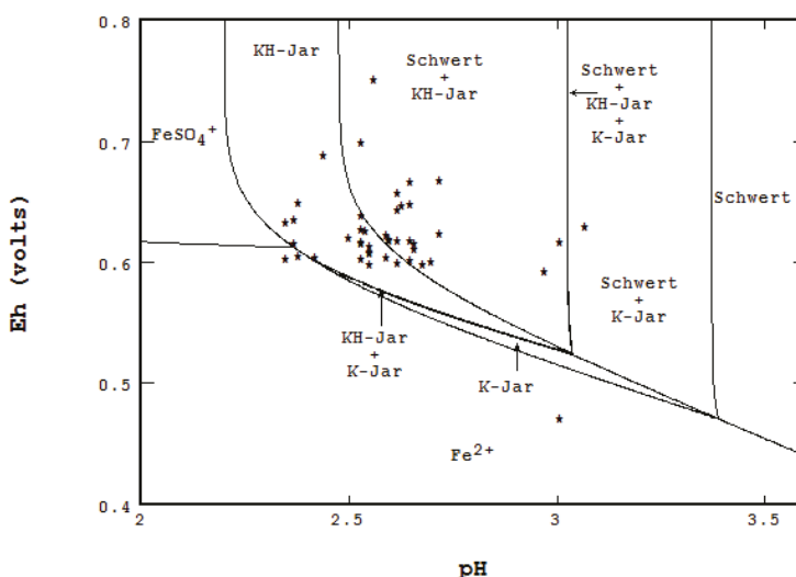
Figure 16. Mass balanced Eh-pH diagram for the Fe-K-S system at 7 °C. This diagram shows the coexistence among schwertmannite, K-jarosite and KH-jarosite. * represents the data analyzed from the sampled water.
