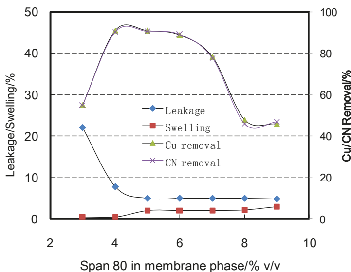
Figure 6. Effect of Span 80 concentration on ELM stability and copper and cyanide removal. (For ELMs formation, membrane phase: 2% v/v 1-dodecanol, 1% v/v liquid paraffin, balanced with kerosene; Internal phase: 0.05 mol/L KOH solution. Volume ratio of the membrane phase to the internal phase: 1:1; Mixing for emulsification: 15 min at 4500 RPM. The external aqueous phase: dilute copper cyanide solution, [Cu]_T = 19.3 mg/L, [CN]_T = 23.6 mg/L, pH 9.5. Mixing of ELMs and the external phase: 15 min at 300 RPM).
