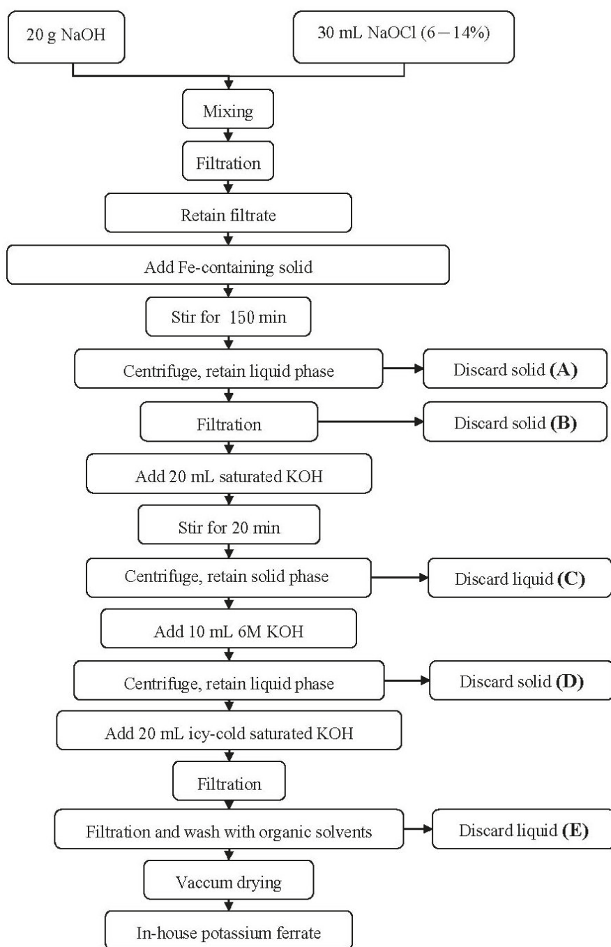
Figure 1. Flowchart for synthesizing in-house potassium ferrate.
