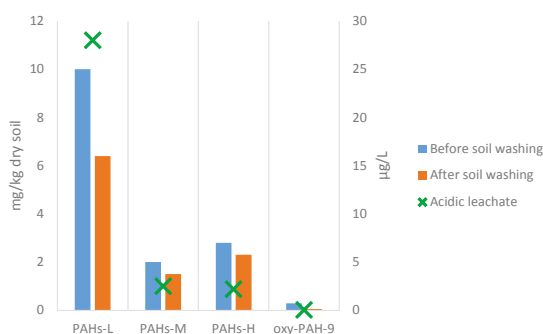
Figure 7. Concentrations of PAHs and oxy-PAHs analyzed in the A1 spiked soil sample before and after acidic washing (mg/kg), and the concentrations in the corresponding acidic leachate (µg/L).
