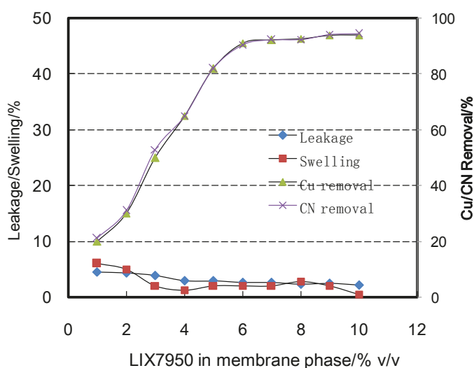
Figure 5. Effect of LIX 7950 concentration on ELM stability and copper and cyanide removal. (For ELMs formation, membrane phase: 2% v/v 1-dodecanol, 5% v/v Span 80, 1% v/v liquid paraffin, balanced with kerosene; Internal phase: 0.05 mol/L KOH solution. Volume ratio of the membrane phase to the internal phase: 1:1; Mixing for emulsification: 15 min at 4500 RPM. The external aqueous phase: dilute copper cyanide solution, [Cu]_T = 19.3 mg/L, [CN]_T = 23.6 mg/L, pH 9.5. Mixing of ELMs and the external phase: 15 min at 300 RPM).
