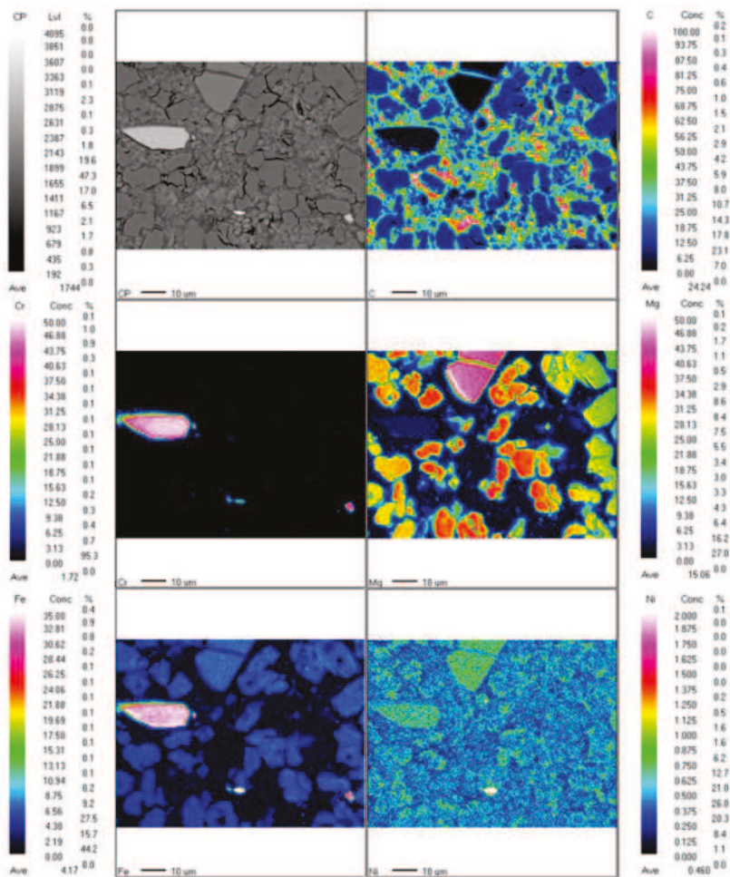
Figure 6. Backscattered scanning electron image and elemental concentration mapping (carbon, chromium, magnesium, iron and nickel) of fully carbonated olivine, captured by EPMA; concentration scale is relative to max/min levels; color gradient in Mg map is due to curvature artifact that occurs at these relatively low magnifications.
