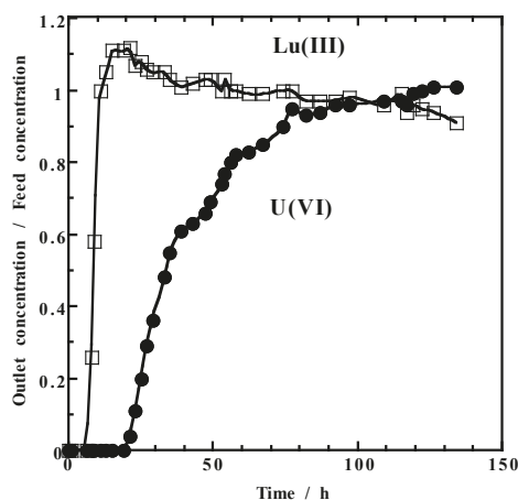
Figure 3. Breakthrough profile of uranium(VI) and lutetium(III) from the column packed with persimmon peel (PP) gel.
