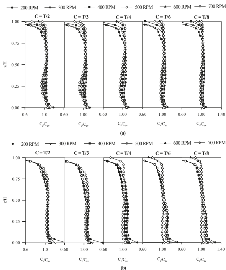
Figure 5. Axial concentration profiles at different stirrer speeds and off-bottom clearance for impeller to tank diameter ratio of (a) 0.5 and (b) 0.33.
