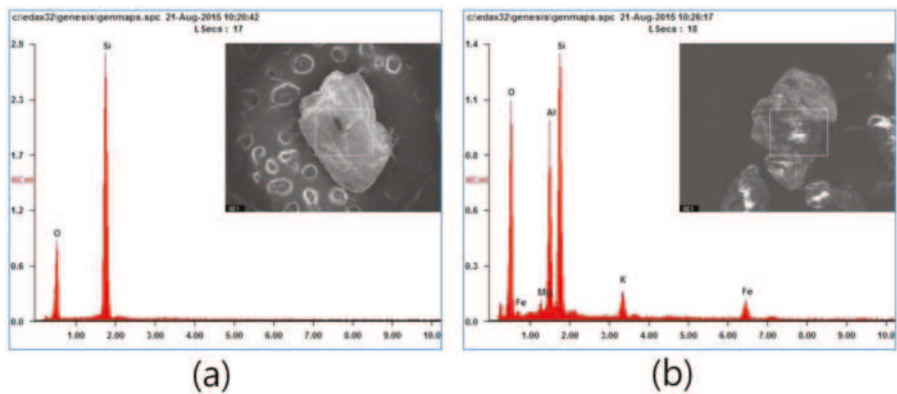
Figure 7. EDX analyses of the sea sand and fine soil sand before the cleaning process (four-year-old samples). (a) Sea sand and (b) fine soil sand.
