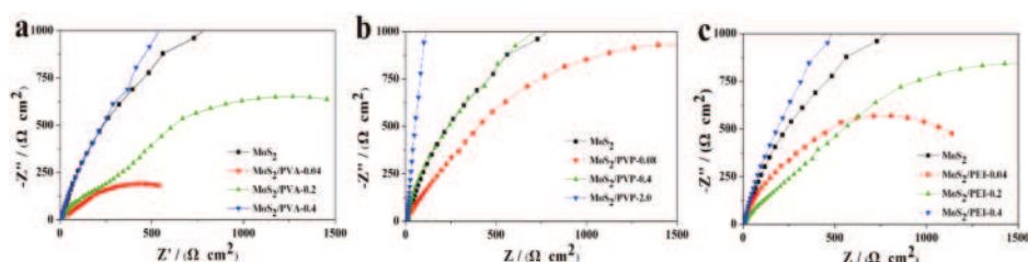
Figure 8. Nyquist plots of MoS 2 -based nanoflower-like composite catalysts: (a) MoS 2 /PVA composite; (b) MoS 2 /PVP composite; (c) MoS 2 /PEI composite.
