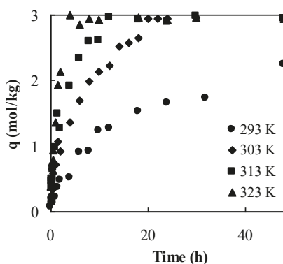
Figure 23. Time variation of the adsorption of gold(III) on CPT gel at different temperatures [33] (with permission for reuse from Elsevier B.V.).
