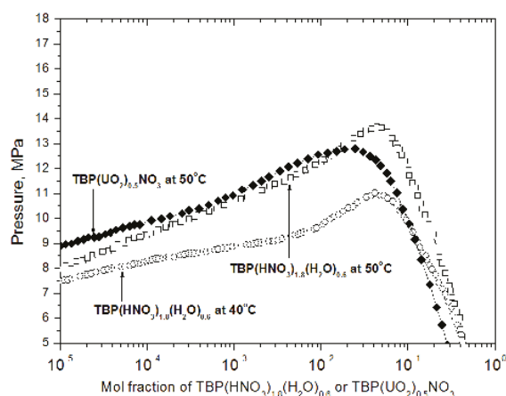
Figure 1. Solubility curves for the transition pressures from two-phase to single-phase \text{TBP} \cdot (\text{UO}_2)_{0.5} \cdot \text{NO}_3 and \text{TBP} \cdot (\text{HNO}_3)_{1.8} \cdot (\text{H}_2\text{O})_{0.6} in supercritical \text{CO}_2 [13].
