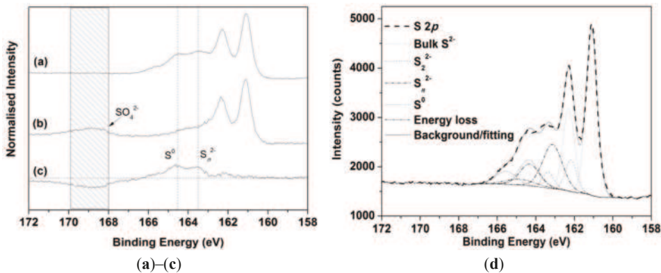
Figure 4. S 2p spectra collected from the chalcopyrite slabs dissolved at 750 mV, 75 °C and pH 1.0 for 30 h: (a) chalcopyrite from galvanic cell; (b) chalcopyrite only; (c) (a) minus (b); (d) fitting of (a).
