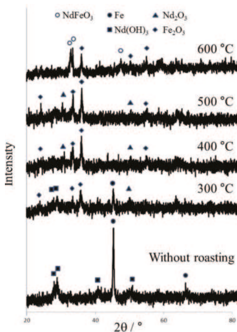
Figure 3. XRD patterns of roasted sample with temperature (Grinding conditions: 15 in stoichiometric molar ratio, 550 rpm in rotational speed, 5 \text{cm}^3 in water addition, 30 min in grinding time).
