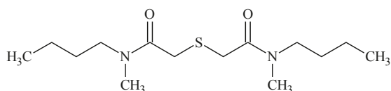
Figure 1. Structure of N,N' -dimethyl- N,N' -dibutylthiodiglycolamide (DMDBTDGA).
