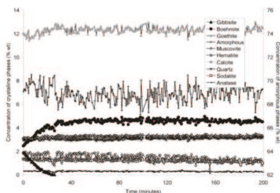
Figure 6. Concentration of crystalline and amorphous phases in bauxite residue slurry in capillary reaction vessels as a function of treatment time at 170 °C, as determined by Rietveld-based quantitative mineral analysis of X-ray diffractograms. Note that amorphous content is plotted on the secondary Y axis and represents contributions from X-ray amorphous minerals in bauxite residue, water in the slurry, and the fused silica capillary.
