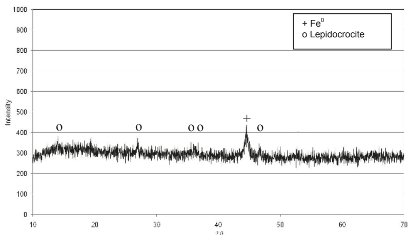
Figure 5. XRD of iron corrosion product after the tests conducted with \text{Fe}^0 = 3 \text{ g/L} , \text{N}_i = 50 \text{ mg/L} and \text{pH} = 3 .
