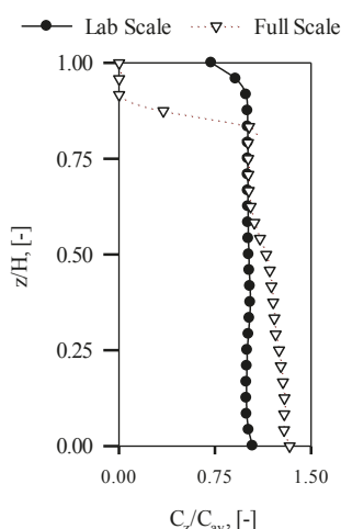
Figure 7. Axial concentration profiles for lab scale ( T = 0.288 \text{ m} ) and full scale ( T = 10 \text{ m} ) stirred tanks with C = T/6 and D_i = T/3 .
