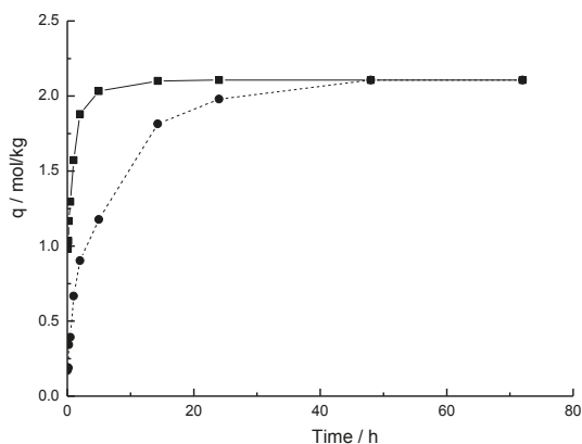
Figure 29. Time variation of the amount of gold(III) on CPW (●)gel and DMA-PW (■)gel from 0.1 \text{ mol} \cdot \text{dm}^{-3} hydrochloric acid solution [36] (with permission for reuse from Elsevier B.V.).
