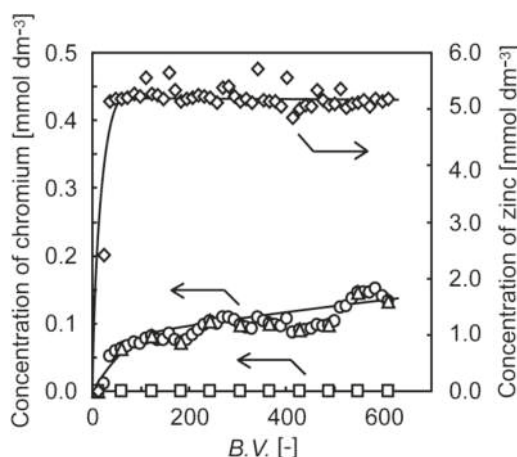
Figure 12. Breakthrough profiles of various chromium and zinc species from the column packed with CPW gel at pH = 1.0 [23] (with permission for reuse from Elsevier B.V.). \circ : Total Cr \Delta : Cr(III) \square : Cr(VI) \diamond : Zn(II).
