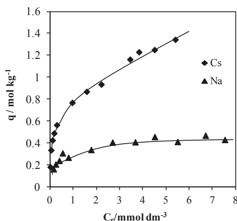
Figure 6. Adsorption isotherms of cesium(I) and sodium(I) ions on CPT gel [17] (with permission for reuse from Elsevier B.V.).
