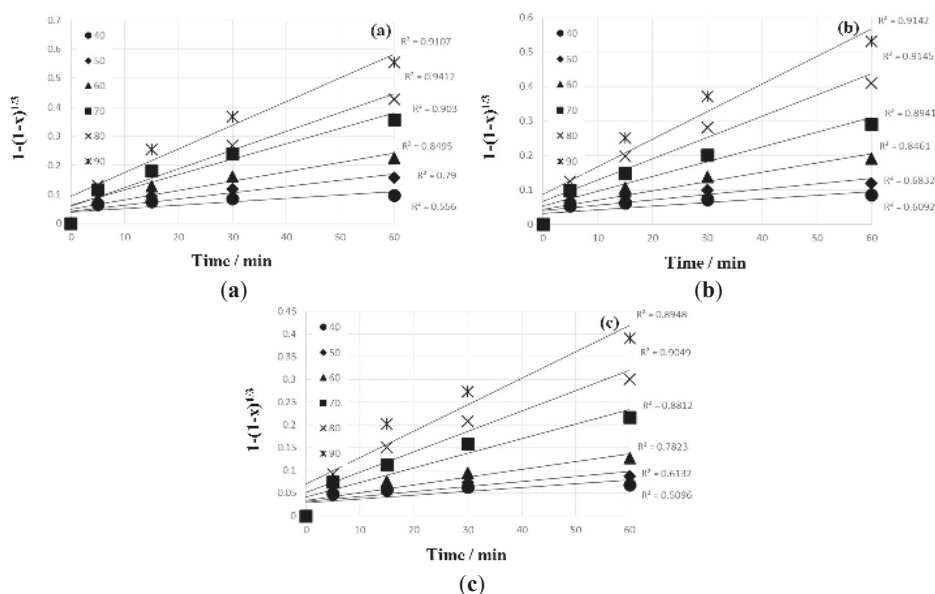
Figure 5. Plot of 1 - (1 - x)^{1/3} vs. T for different temperatures ( [\text{Fe}^{3+}] : (a) 1.0 M; (b) 0.5 M; (c) 0.25 M; 10% pulp density; 400 rpm agitation speed).
