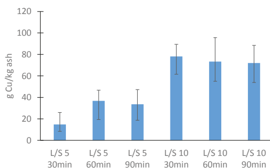
Figure 2. Cu leached from the bark-ash sample A1 with a variation in leaching time (30–90 min) and L/S-ratios (5 and 10). The columns show the average of three replicate tests. The error bars show the maximum and minimum values.
