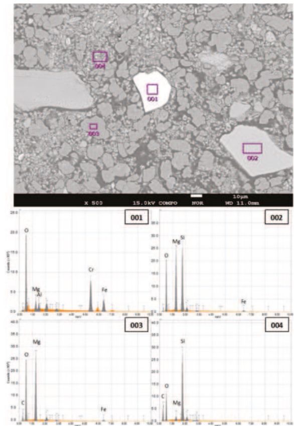
Figure 8. Backscattered scanning electron image of fully carbonated olivine and EPMA scanning of selected areas; mounted sample was coated with platinum and palladium for the analysis.
