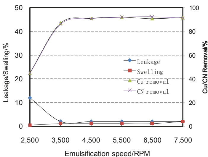
Figure 3. Effect of emulsification speed on ELM stability and copper and cyanide removal. (For ELMs formation, membrane phase: 6% v/v LIX 7950, 2% v/v 1-dodecanol, 5% v/v Span 80, 1% v/v liquid paraffin, balanced with kerosene; Internal phase: 0.05 mol/L KOH; Volume ratio of membrane to internal phases: 1:1; Mixing time: 15 min. The external aqueous phase: dilute copper cyanide solution, [Cu]_T = 19.3 mg/L, [CN]_T = 23.6 mg/L, pH 9.5. Mixing of ELMs and the external phase: 15 min at 300 RPM).
