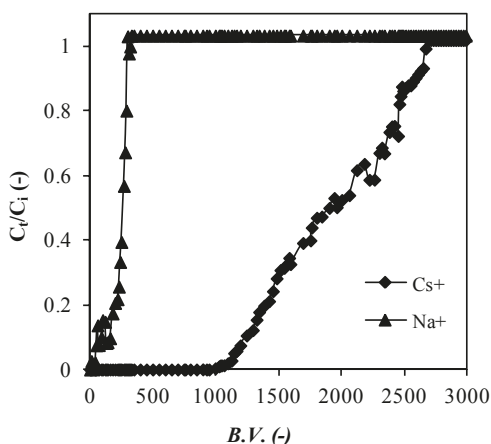
Figure 7. Breakthrough profiles of cesium(I) and sodium(I) ions from the column packed with CPT gel [17] (with permission for reuse from Elsevier B.V.).
