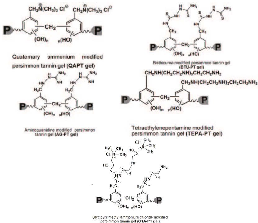
Scheme 4. Chemical structures of the gels prepared from persimmon tannin extract powder via chemical modification immobilizing functional groups of quaternary ammonium (QA), bithiourea (BTU), aminoguanidine (AG), tetraethylenepentamine (TEPA) and glycidyltrimethyl ammonium (GTA) where P stands for persimmon tannin moiety.
