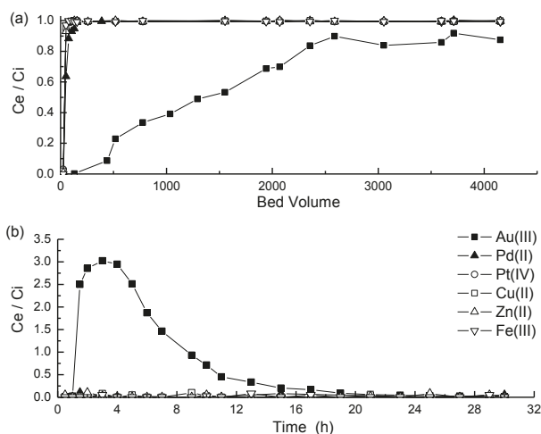
Figure 30. (a) Breakthrough profiles of various metal ions contained in the sample solution of the actual effluent of the precious metals industry from the first column packed with CPW gel; (b) Elution profiles of various metal ions from the first column using aqueous mixture of 0.1 \text{ mol}\cdot\text{dm}^{-3} thiourea in 1 \text{ mol}\cdot\text{dm}^{-3} hydrochloric acid solution [36] (with permission for reuse from Elsevier B.V.).
