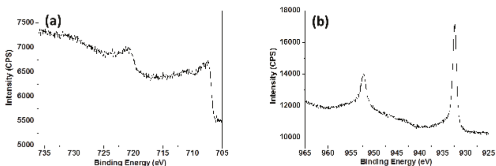
Figure 6. XPS spectra collected from the chalcopryrite surface in contact with pyrite (galvanic cell) leached for 30 h at 750 mV, 75 °C and pH 1.0: (a) Fe 2p; (b) Cu 2p.
