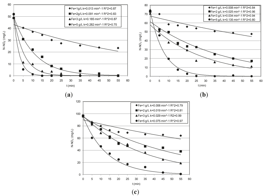
Figure 1. Trends of nitrate concentrations detected during the tests conducted at pH = 3: (a) N_i = 50 \text{ mg/L} ; (b) 70 \text{ mg/L} ; (c) 95 \text{ mg/L} .
