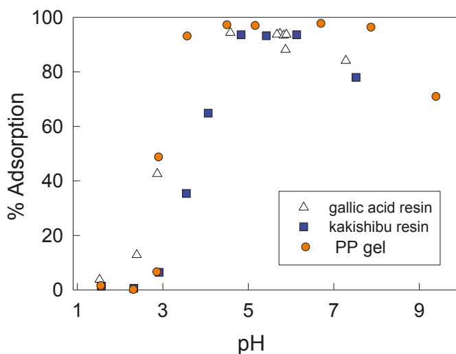
Figure 1. Percentage adsorption of uranium(VI) at varying equilibrium pH on PP gel, gallic acid resin and kakishibu resin.
