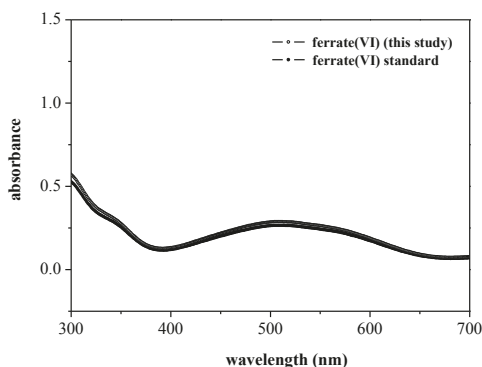
Figure 4. UV-Vis absorbance spectra of in-house and Sigma-Aldrich potassium ferrates at a concentration of 2.88 \times 10^{-4} M.
