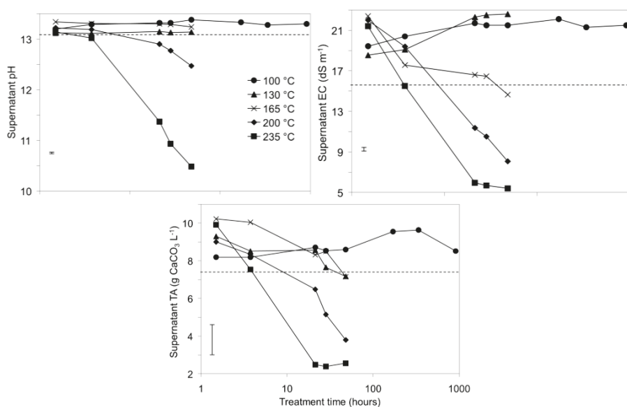
Figure 1. pH, EC, and total alkalinity (TA) of supernatants from bauxite residue during pressure vessel treatments at various temperatures. Dashed lines indicate t = 0 values. Note that treatment time (X axis) is graphed on a logarithmic scale. Error bars indicate 95% confidence interval for the mean of the 100 °C treatment at 909 h.
