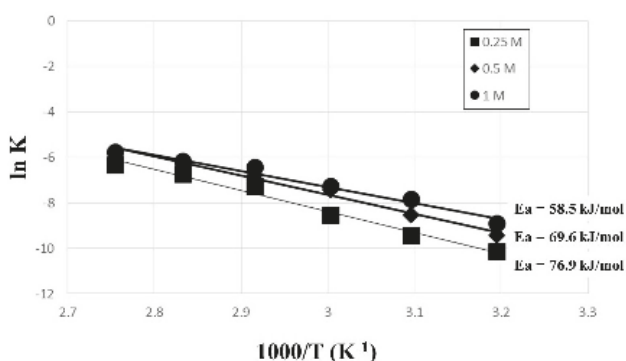
Figure 7. Arrhenius plots. (1 kmol m -3 HCl; 0.25 kmol m -3 –1 kmol m -3 Fe 3+ ; 400 rpm agitation speed; 10% pulp density; 40 °C–90 °C temperature).
