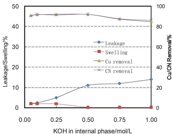
Figure 4. Effect of KOH on ELM stability and copper and cyanide removal. (For ELMs formation, membrane phase: 6% v/v LIX 7950, 2% v/v 1-dodecanol, 5% v/v Span 80, 1% v/v liquid paraffin, balanced with kerosene; Volume ratio of membrane to internal phases: 1:1; Mixing for emulsification: 15 min at 4500 RPM. The external aqueous phase: dilute copper cyanide solution, [Cu]_T = 19.3 mg/L, [CN]_T = 23.6 mg/L, pH 9.5. Mixing of ELMs and the external phase: 15 min at 300 RPM).
