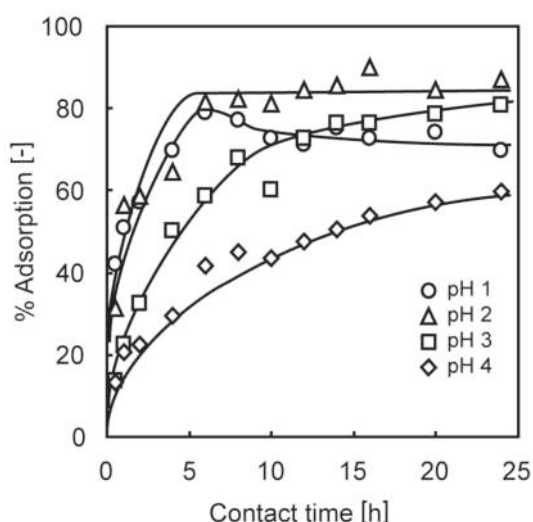
Figure 9. Effect of contact time on the adsorption of total chromium on cross-linked persimmon waste (CPW) gel from chromium(VI) solution at different pH values [23] (with permission for reuse from Elsevier B.V.).
