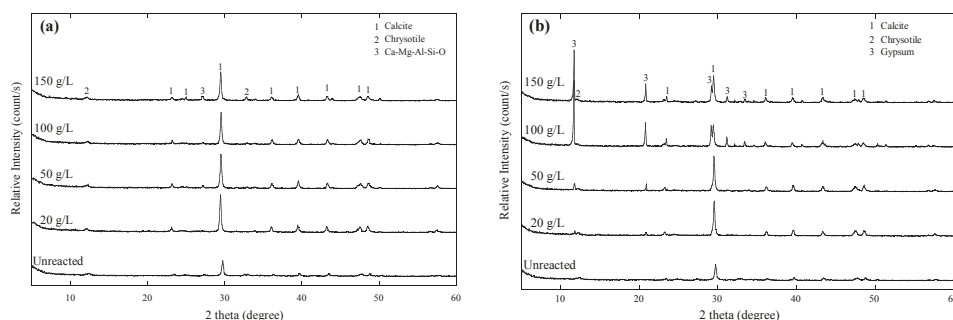
Figure 8. X-ray diffraction (XRD) patterns of unreacted waste slate (Unreacted) and reacted waste slate samples obtained from carbonation tests using (a) 1 M \text{CH}_3\text{COONH}_4 and (b) 1 M \text{NH}_4\text{HSO}_4 solutions at various solid dosages (20, 50, 100, and 150 g/L).
