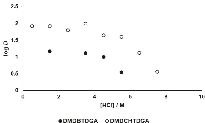
Figure 3. Variation of the log D values of Pd(II) with the HCl concentration by DMDBTDGA and DMDCHTDGA ( 9.4 \times 10^{-4} M Pd(II) in 0.5 M to 7.5 M HCl; 0.02 M DMDBTDGA or DMDCHTDGA* in toluene; A/O = 1, room temperature, 900–1000 rpm, 30 min). Standard deviations: \pm 5\% (*: data collected from [20]).
