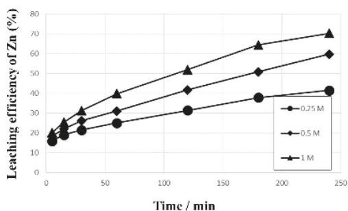
Figure 3. The effects of \text{Fe}^{3+} concentration on the leaching efficiency of Zn at 1 \text{ kmol}\cdot\text{m}^{-3} HCl, 10% pulp density, 50^\circ\text{C} , and 400 rpm.
