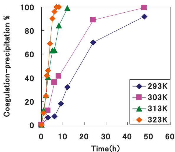
Figure 17. Percentage recovery of gold(III) by means of coagulation using persimmon extract liquor from 0.1 \text{ mol} \cdot \text{dm}^{-3} hydrochloric acid solution at varying temperatures [32] (with permission for reuse from The Society of Chemical Engineers of Japan).
