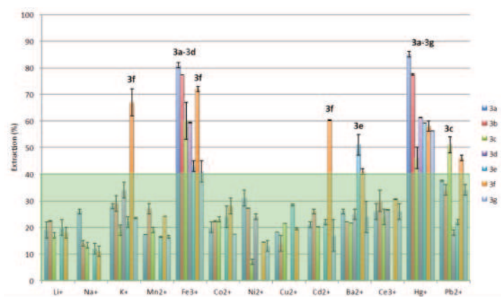
Figure 4. Extraction efficiencies of metal cations by the triazolic piperazine polymers 3a–3g (polymers extracting at levels \geq 50\% are indicated).
