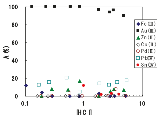
Figure 25. Percentage adsorption of some metal ions on PP gel from varying concentration ( \text{mol}\cdot\text{dm}^{-3} ) of hydrochloric acid [34] (with permission for reuse from Elsevier B.V.).
