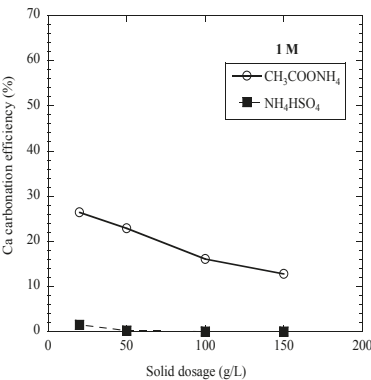
Figure 6. Ca carbonation efficiencies as a function of the solid dosage with the 1.0 M CH 3 COONH 4 and 1.0 M NH 4 HSO 4 solutions for waste slate samples.
