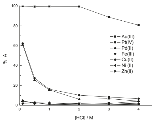
Figure 28. Percentage adsorption of various metal ions on DMA-PW gel from varying concentration ( \text{mol} \cdot \text{dm}^{-3} ) of hydrochloric acid solution [36] (with permission for reuse from Elsevier B.V.).
