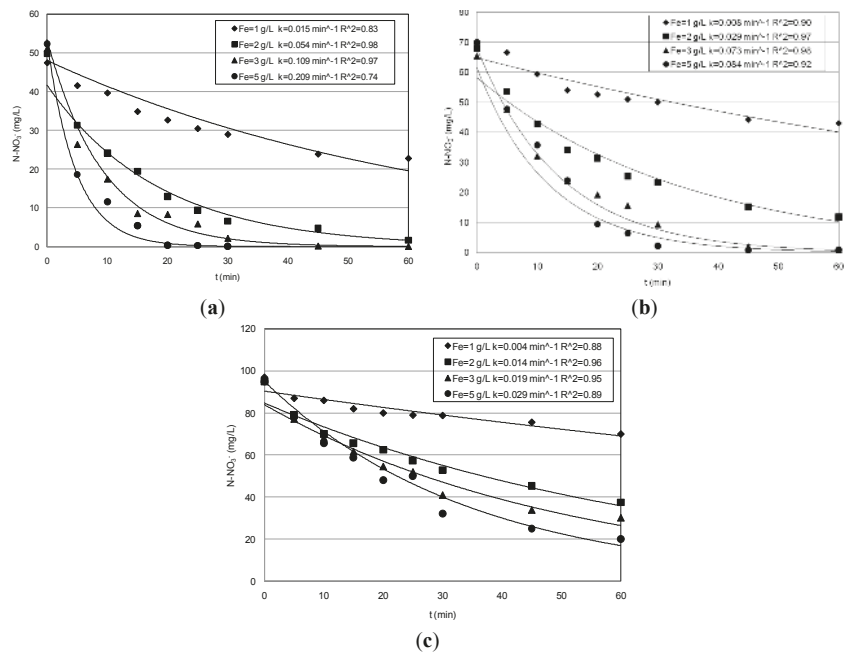
Figure 2. Trends of nitrate concentrations detected during the tests conducted at pH = 5: (a) N_i = 50 \text{ mg/L} ; (b) 70 \text{ mg/L} ; (c) 95 \text{ mg/L} .
