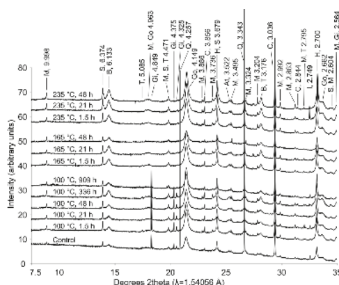
Figure 7. X-ray diffraction patterns from bauxite residue before and after hydrothermal treatment. Treatment time and temperature are indicated for each pattern. Peaks between 7.5°–35° 2 \theta are labeled with d-spacings (Å) and abbreviations for minerals as follows: M—muscovite; S—sodalite; B—boehmite; T—tricalcium aluminate; Go—goethite; Gi—gibbsite; Q—quartz; C—calcite; H—hematite; At—natase; I—ilmenite.
