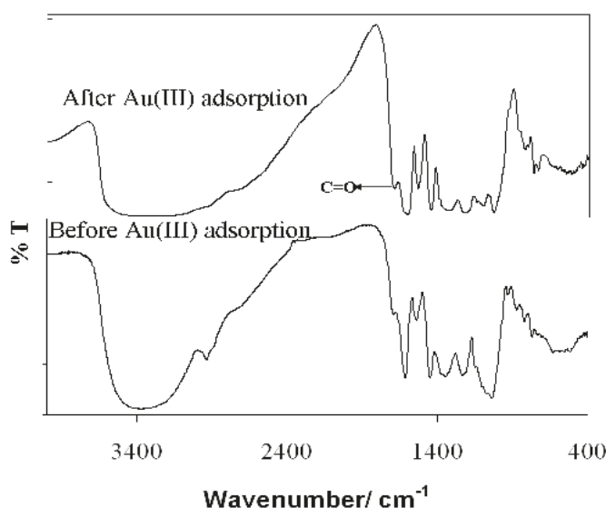
Figure 22. FT-IR spectra of crude PT powder before and after the adsorption of gold(III) [33] (with permission for reuse from Elsevier B.V.).
