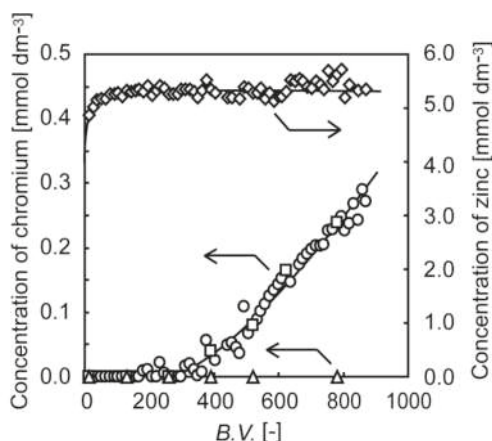
Figure 13. Breakthrough profiles of various chromium and zinc species from the column packed with CPW gel at pH = 4.0 [23] (with permission for reuse from Elsevier B.V.). ○: Total Cr △: Cr(III) □: Cr(VI) ◇: Zn(II).
