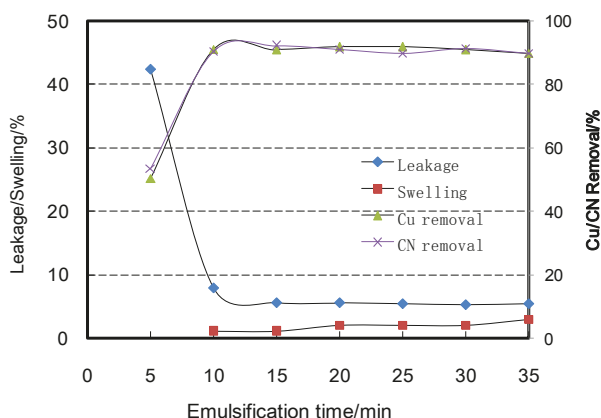
Figure 2. Effect of emulsification time on ELM stability and copper and cyanide removal. (For ELMs formation, membrane phase: 6% v/v LIX 7950, 2% v/v 1-dodecanol, 5% v/v Span 80, 1% v/v liquid paraffin, balanced with kerosene; Internal solution: 0.05 mol/L KOH; Volume ratio of membrane to internal phases: 1:1; Mixing speed: 4500 RPM. The external aqueous phase: dilute copper cyanide solution, [\text{Cu}]_{\text{T}} = 19.3 \text{ mg/L} , [\text{CN}]_{\text{T}} = 23.6 \text{ mg/L} , pH 9.5. Mixing of ELMs and the external solution: 15 min at 300 RPM).
