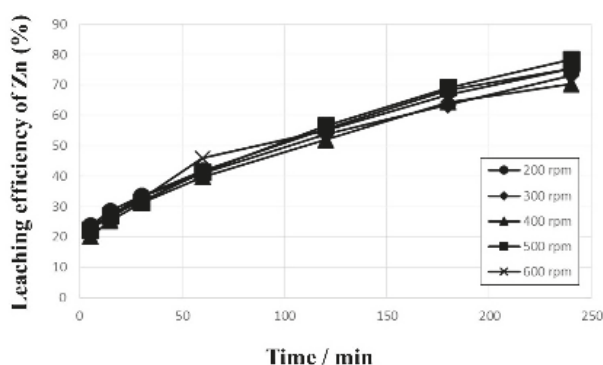
Figure 2. The effects of agitation speed on the leaching efficiency of Zn at 1 \text{ kmol}\cdot\text{m}^{-3} HCl with 1 \text{ kmol}\cdot\text{m}^{-3} \text{Fe}^{3+} , 10% pulp density, and 50^\circ\text{C} .
