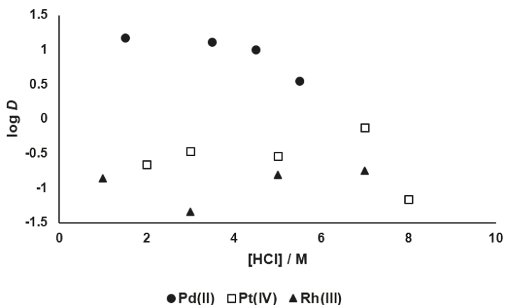
Figure 2. Variation of the \log D values of Pd(II), Pt(IV), and Rh(III) with the HCl concentration ( 9.4 \times 10^{-4} M Pd(II), 5.1 \times 10^{-4} M Pt(IV), or 9.7 \times 10^{-4} M Rh(III) in 1.0 M to 8.0 M HCl; 0.02 M DMDBTDGA in toluene; A/O = 1, room temperature, 900–1000 rpm, 30 min). Standard deviations: \pm 5\% .
