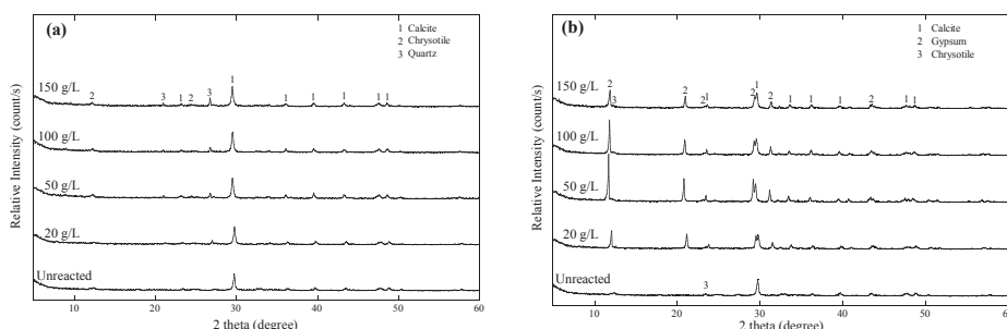
Figure 5. X-ray diffraction (XRD) patterns of as-received waste slate (Unreacted) and reacted waste slate samples obtained from leaching tests using the (a) 1 M \text{CH}_3\text{COONH}_4 and (b) 1 M \text{NH}_4\text{HSO}_4 solutions at various solid dosages (20, 50, 100, and 150 g/L).
