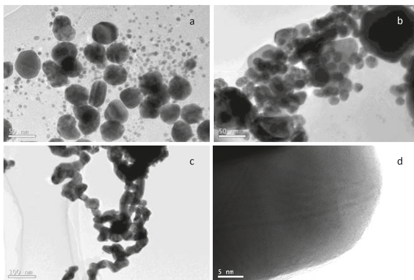
Figure 4. Effect of gold ions concentration. TEM images of gold nanoparticles obtained at pH 10 using different HAuCl 4 concentrations: (a) 100; (b) 250; and (c) 500 mg/L; (d) detail of nanostructure of the gold nanowires.
