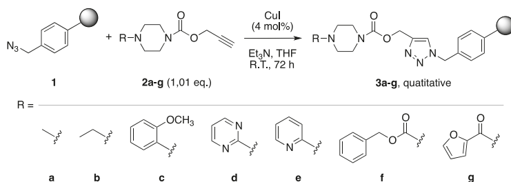
Figure 2. Synthesis of the polymers by CuAAC procedure.
