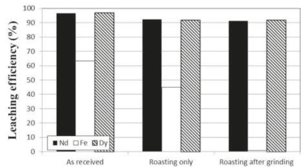
Figure 6. The comparison of leaching efficiencies using samples as as-received, only roasted, and roasted after being ground.
