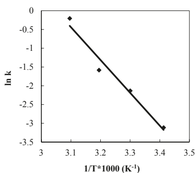
Figure 24. Arrhenius plots for the pseudo-first-order rate constants for CPT gel where the straight line is expressed by the linear equation, Y = -8.57x + 26.7 , with the correlation factor ( R^2 ) = 0.9671 [33] (with permission for reuse from Elsevier B.V.).
