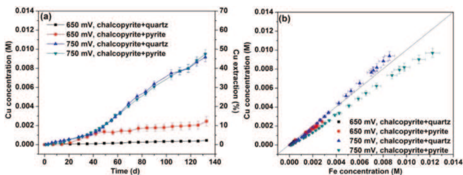
Figure 1. Leach data resulting from the flow-through experiments conducted at 75 °C, pH 1.0, 650 mV and 750 mV: (a) Cu concentration and % extraction versus time; (b) Cu concentration against Fe concentration.
