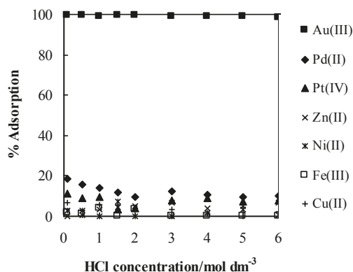
Figure 18. Percentage adsorption of various metal ions on CPT gel as a function of concentration of hydrochloric acid [33] (with permission for reuse from Elsevier B.V.).
