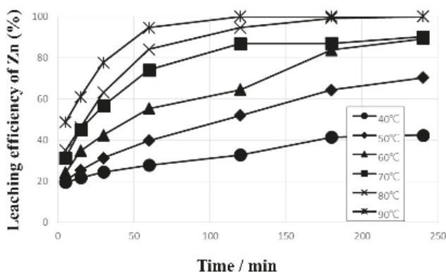
Figure 4. The effects of temperature on the leaching efficiency of Zn at 1 kmol·m −3 HCl with 1 kmol·m −3 Fe 3+ , 10% pulp density, and 400 rpm.
