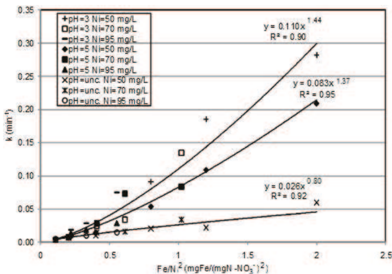
Figure 7. Trends of the k constant vs. the \text{Fe}/N_i^2 ratio.
