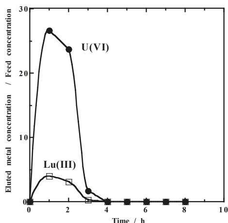
Figure 4. Elution profiles of uranium(VI) and lutetium(III) from the PP gel packed column after breakthrough using 1 mol·dm −3 hydrochloric acid solution.
