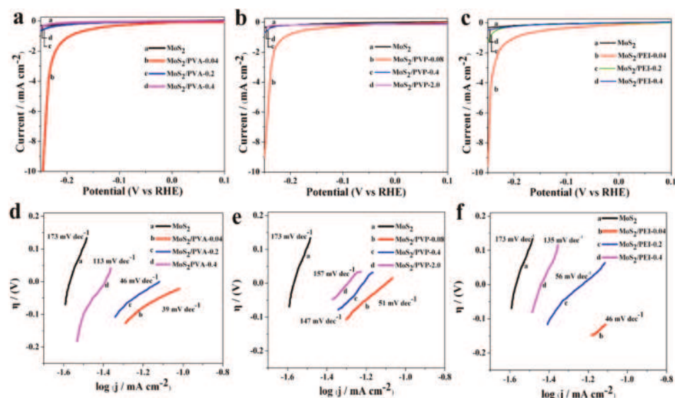
Figure 7. Polarization curves (a–c) and corresponding Tafel plots (d–f) of the MoS 2 /PVA, MoS 2 /PVP, MoS 2 /PEI composites.
