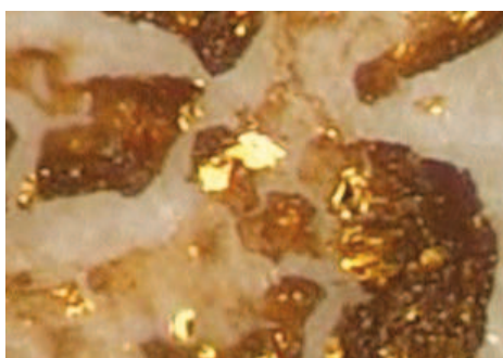
Figure 15. Image of the filter cake of the precipitate generated by the addition of persimmon extract liquor into the gold(III) solution observed by optical microscope ( \times 800 ).
