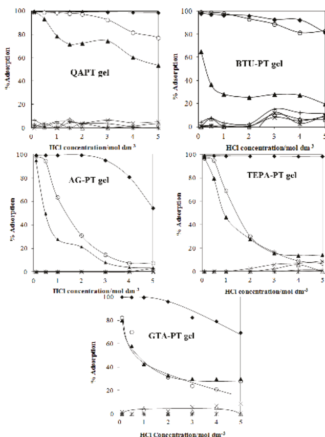
Figure 32. Percentage adsorption of various metal ions on some chemically modified PT gel from varying concentration of hydrochloric acid. ◆ Au(III), ○ Pd(II), ▲ Pt(IV), □ Cu(II), × Zn(II), △ Ni(II), * Fe(III).
