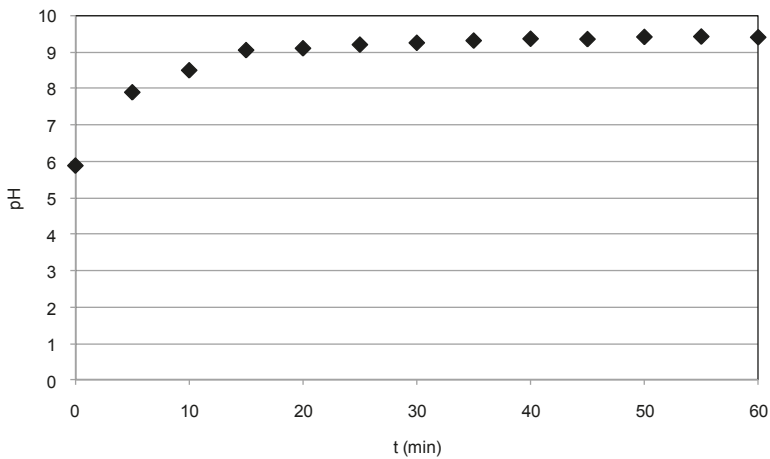
Figure 3. pH trend during the test conducted with \text{Fe}^0 = 3 \text{ g/L} , N_i = 50 \text{ mg/L} and uncontrolled pH.
