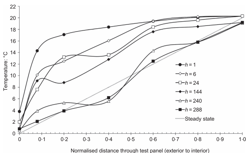
Figure 1. Temperature change in 300 mm hemp-lime wall after a sudden temperature drop
