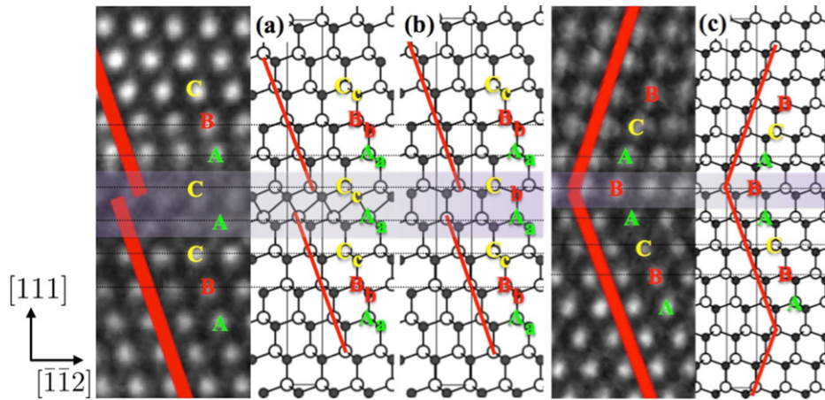
Figure 3. Structural analysis of HRTEM images (from Figure 2) and atomistic modelling for (a) polytype and (b) tetrahedral intrinsic stacking faults (11 atomic layers) and (c) twin boundary (13 atomic layers). The white and black atoms refer to Cd and Te, respectively. The purple shaded region indicates the stacking fault location; the horizontal dotted lines represent the matching of the Cd atomic layers in the model and HRTEM structures. Upper- and lower-case letters represent Cd and Te, respectively, where the perfect fcc crystal follows AaBbCc.
