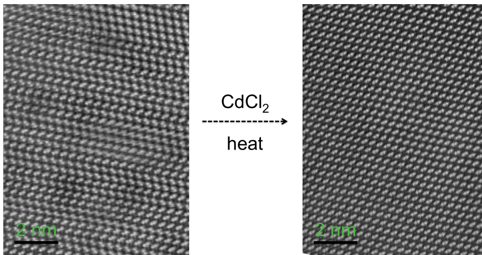
Figure 2. High-resolution TEM image of CdTe before (left) and after (right) annealing treatment. An atomistic model for the stacking faults observed is given in Figure 3.
