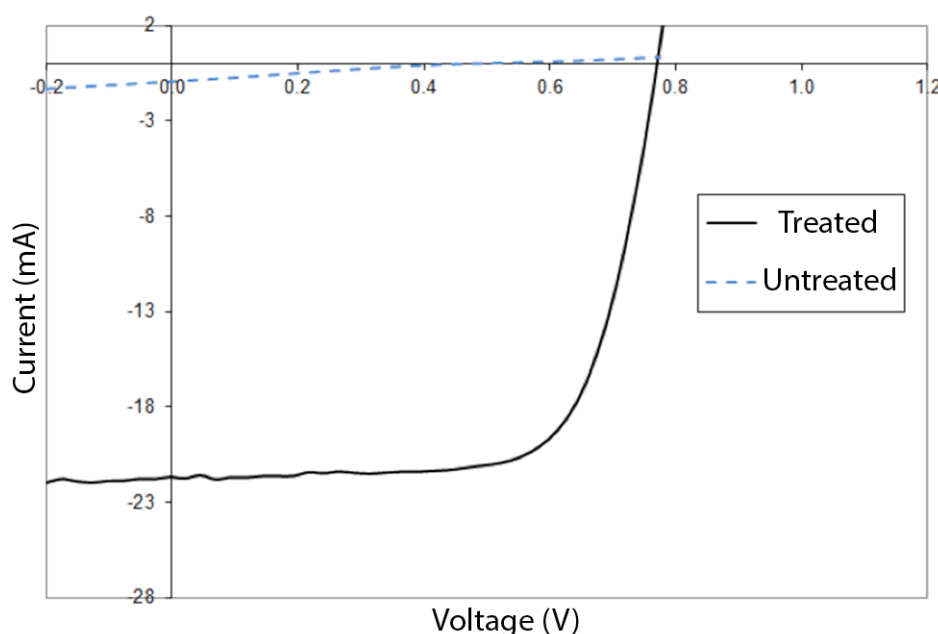
Figure 1. Current-voltage characteristics of an untreated thin-film CdTe photovoltaic cell compared with a cadmium chloride treated device.
