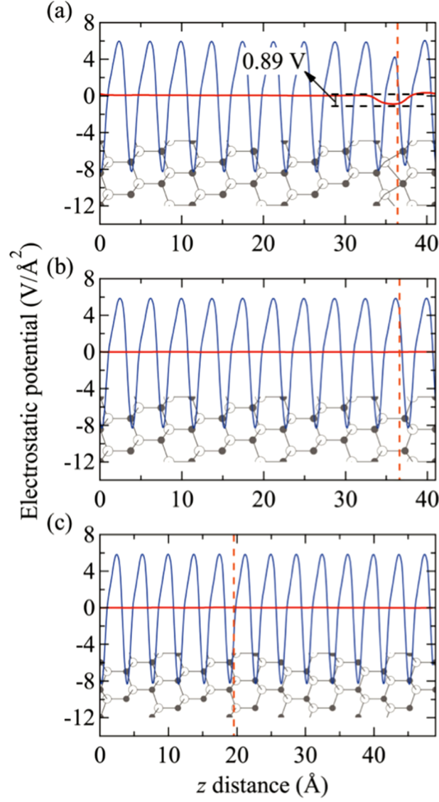
Figure 4. Calculated electrostatic potential of intrinsic stacking faults with (a) polytype, (b) tetrahedral and (c) twin boundary systems. The blue solid, red solid and orange dotted lines represent the planar averaged electrostatic potential, macroscopic averaged electrostatic potential and location of SF, respectively. Simultaneously, the supercells of each SF system are shown in below of graph with Cd (white empty ball) and Te (black solid ball).
