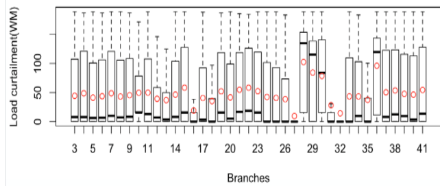
Fig. 7. The loss load due to branch outage
