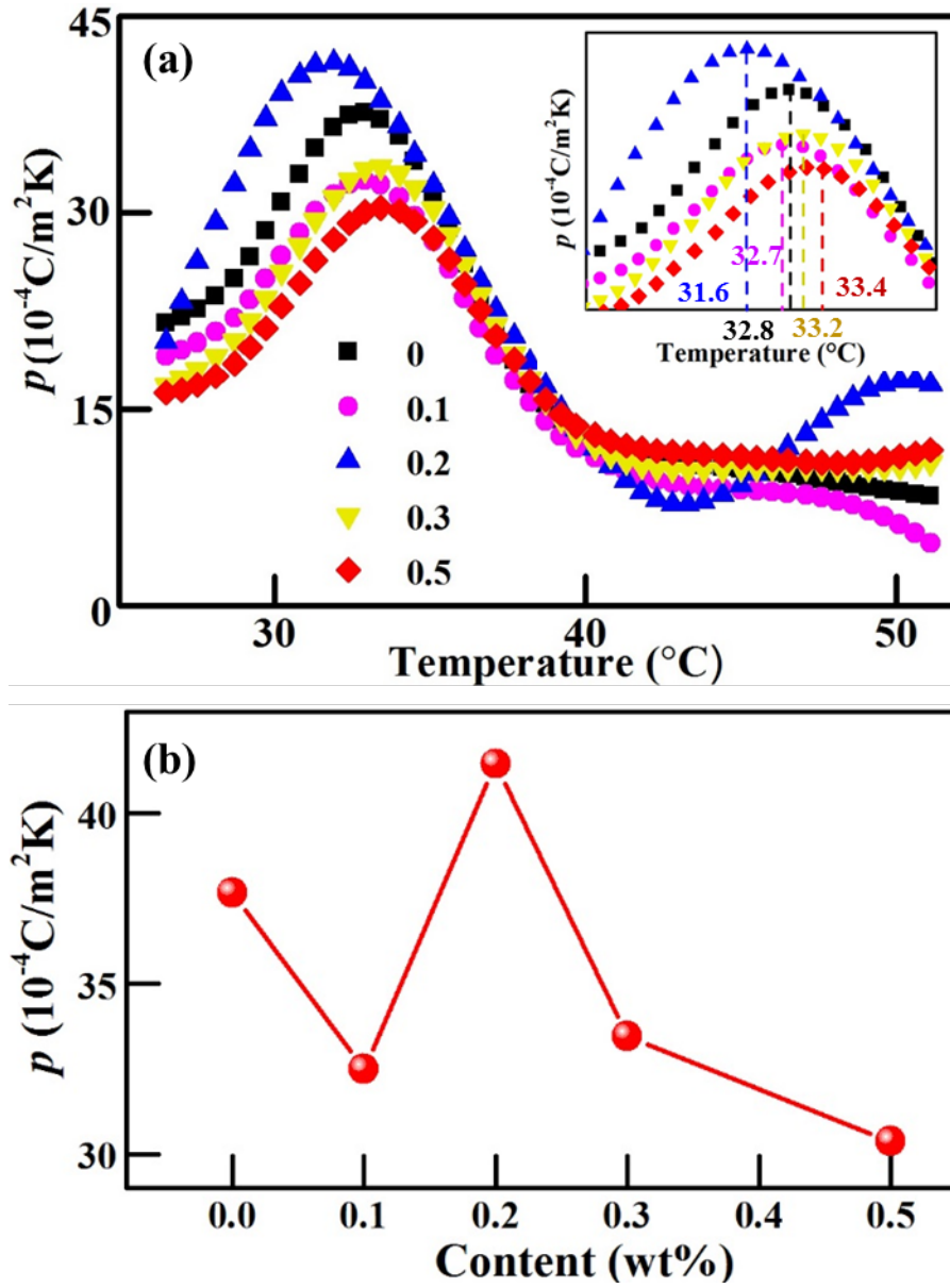
Fig. 6. (a) Temperature-dependent pyroelectric coefficient of the PMN-PMS-PZT:AlN samples with various AlN contents: 0, 0.1, 0.2, 0.3, 0.5 wt.%. (b) Values of the pyroelectric coefficient ( p ) for the corresponding samples.
