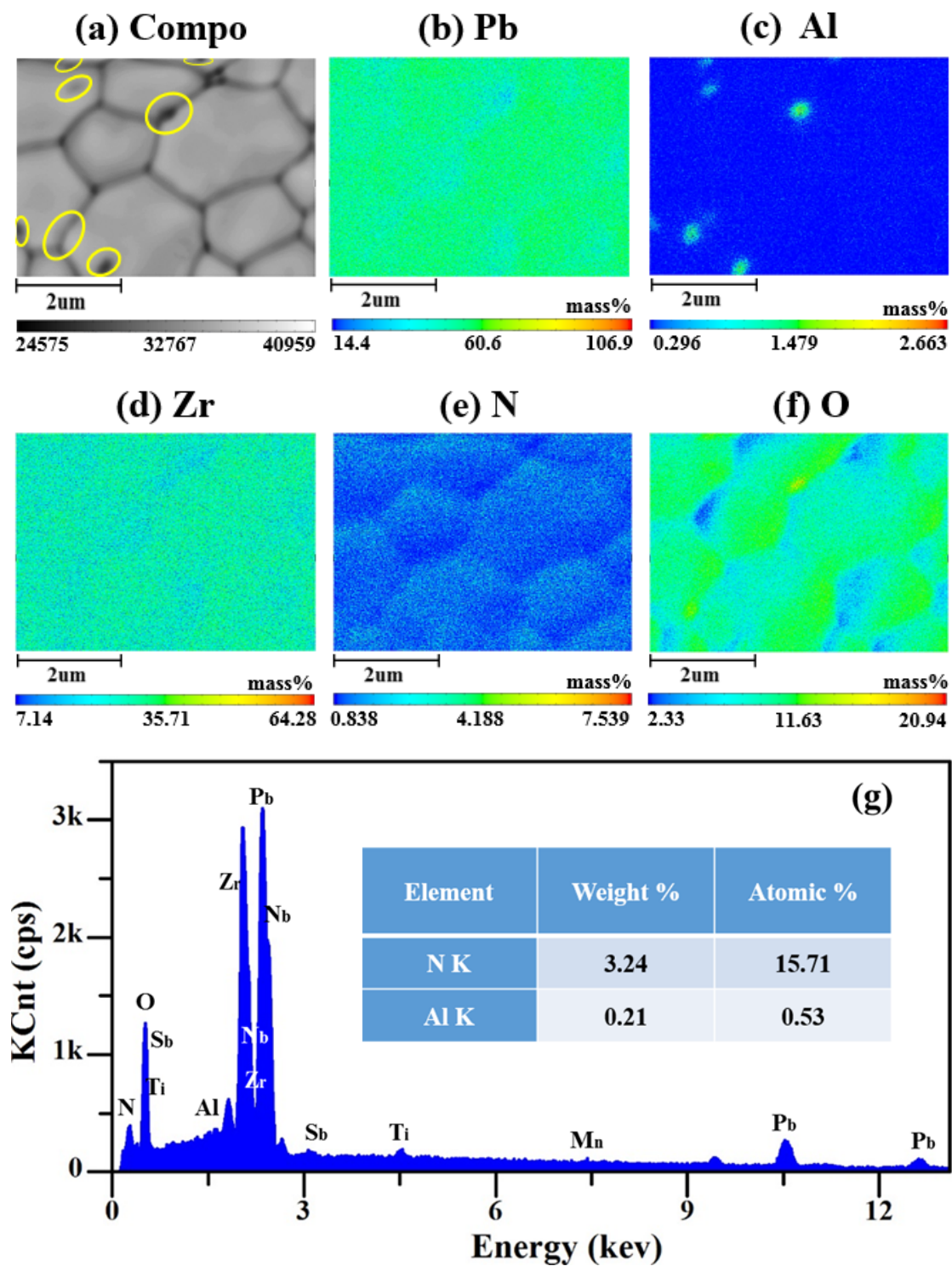
Fig. 3. Elemental analysis of the PMN-PMS-PZT: 0.2AlN sample. (a) SEM image of microstructure. Elemental distribution of (b) Pb, (c) Al, (d) Zr, (e) N, and (f) O. (g) The energy-dispersive spectrum of the PMN-PMS-PZT: 0.2AlN sample.
