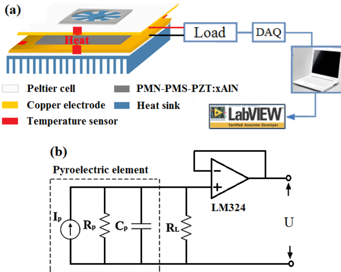
Fig. 8. (a) Schematic of measurement setup and (b) circuit for pyroelectric energy harvesting.
