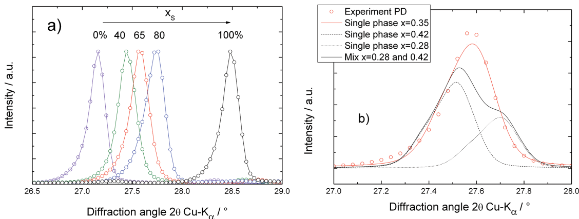
Figure 11. XRD patterns of CZTSSe/Mo thin films with focus on (112) peaks. a) Variable samples with anion ratio x = S/(S+Se) varied from 0 to 100%. b) Full pattern matching results for PD type of sample (i.e., standard sample, red open dots) using a single kesterite phase ( x = 0.35 ) and another fitting example with two mixed phases x = 0.28 / 0.42 with volume fractions of 63%/37%.
