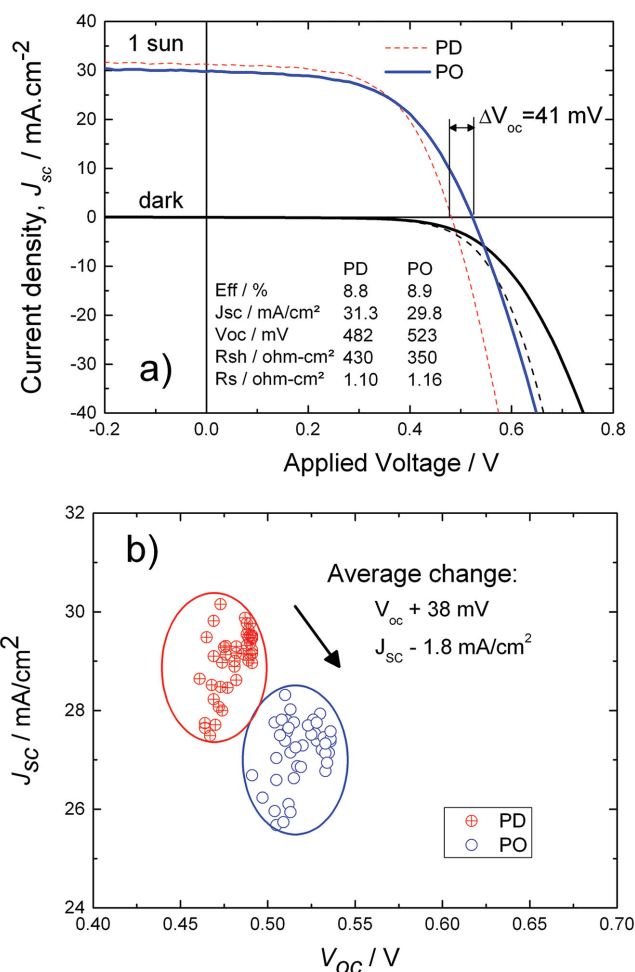
Figure 8. a) Current-Voltage characteristics under 1 sun illumination of PD (partially disordered) and PO (partially ordered) CZTSSe-based photovoltaic devices. b) Set of J_{\text{sc}} - V_{\text{oc}} data points obtained from one batch of solar cells (without ARC).
