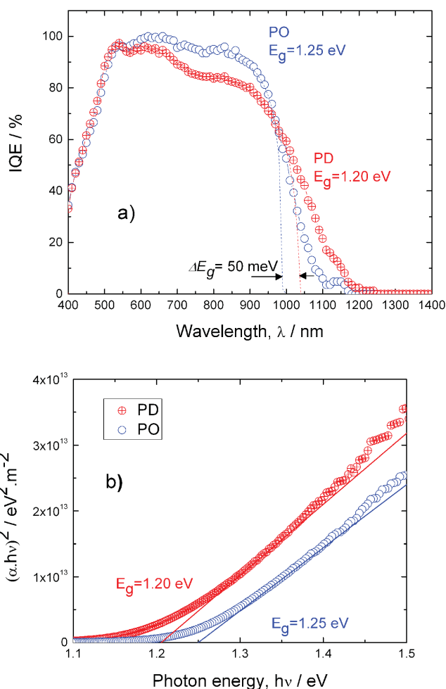
Figure 9. a) Internal quantum efficiency (IQE) spectra of CZTSSe-based photovoltaic devices of PD (red symbols) and PO type (blue symbols). The dotted lines correspond to fitted IQE according to Equation (2) in the range used to extract E_{g-IQE} . b) Linear fit of (\alpha \cdot hv)^2 vs photon energy h\nu , based on the absorption coefficient \alpha measured on lift-off samples from the same batch; used to derive E_{g-abs} (same colors).
