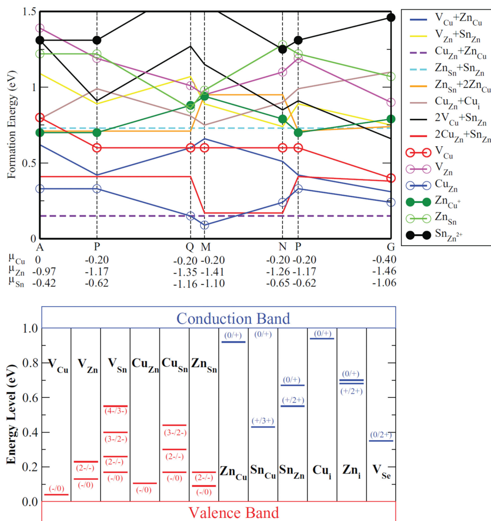
Figure 2. Upper panel: The formation energy of low-energy defects in \text{Cu}_2\text{ZnSnSe}_4 as a function of the chemical potential of the cations. The Fermi energy is assumed to be at the top of the valence band (strong p-type conditions), and all donor defects are fully ionized. Lower panel: The ionization levels of intrinsic defects in the bandgap of \text{Cu}_2\text{ZnSnSe}_4 . The red bars show the acceptor levels and the blue bars show the donor levels, with the initial and final charge states labeled in parentheses. Reproduced with permission. [67] Copyright 2013, Wiley VCH.
