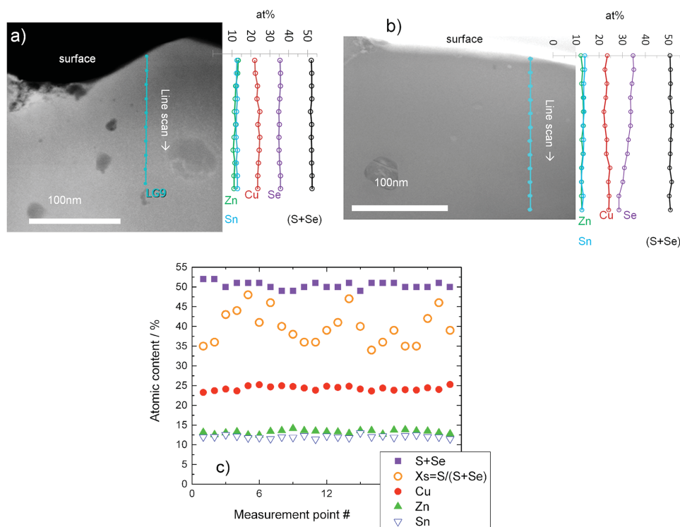
Figure 10. Cross-section STEM-EDX compositional analysis of standard CZTSSe absorber thin films. Line scans in grain with a) uniform and b) non uniform composition. c) Grain-to-grain variation evaluated from 24 data points measured on various grains from a few sections, with 1 data point per grain.
