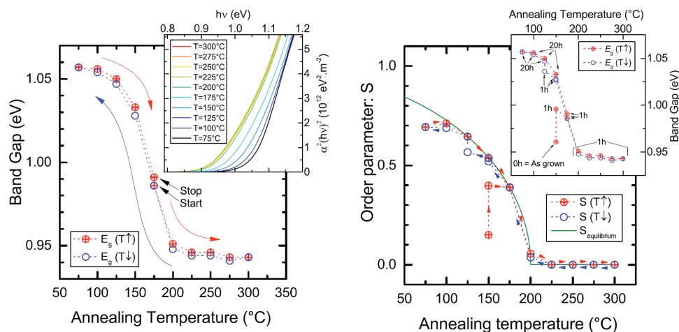
Figure 7. Left panel: Evolution of the CZTSe bandgap with temperature during the annealing/quenching sequence. Inset: Tauc plots for direct bandgap for decreasing temperature. Right panel: calculated evolution of the long-range order parameter during successive annealing. The inset presents the evolution of E_g for the same annealing sequence. Annealing times (dwell times) are shown as labels. Reproduced with permission. [9] Copyright 2014, AIP Publishing LLC.
