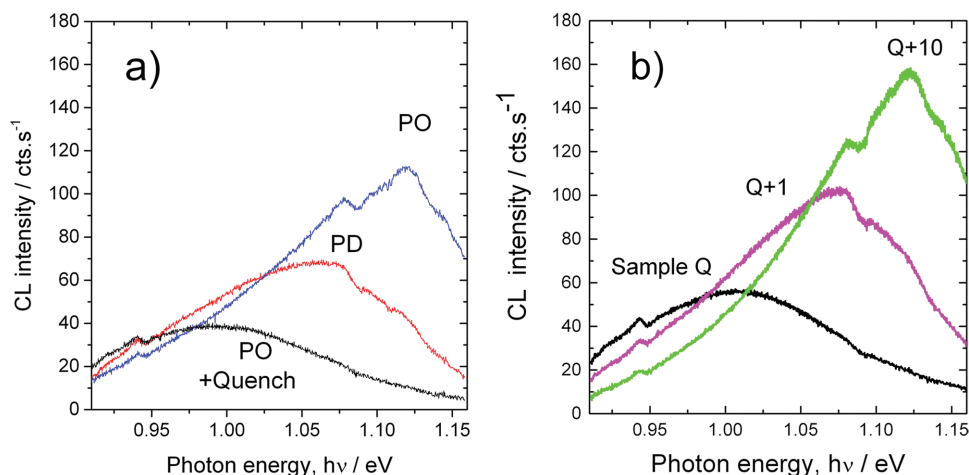
Figure 13. Cathodo-luminescence of CZTSSe layers a) (PO) partially ordered vs (PD) partially disordered samples similar to those used in devices of Figure 8, 9. b) (Q) quenched after a 60 min annealing at 300 °C, (Q+1) quenched and further annealed at 100 °C during 24 hours, and (Q+10) quenched and further annealed at 100 °C during 240 hours.
