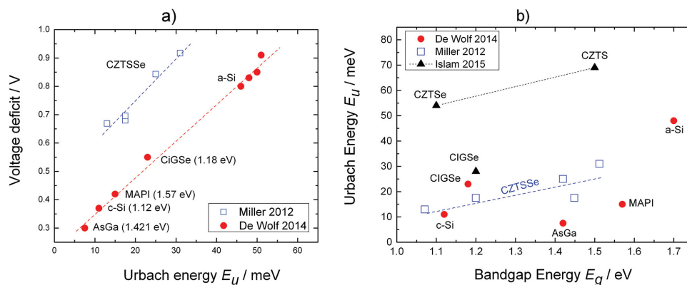
Figure 14. a) Relationship between Urbach energy E_u and lowest reported voltage deficit, for various photovoltaic materials, after De Wolf et al. [76] Data available from Miller et al. [75] and Islam et al. [63] were included.
