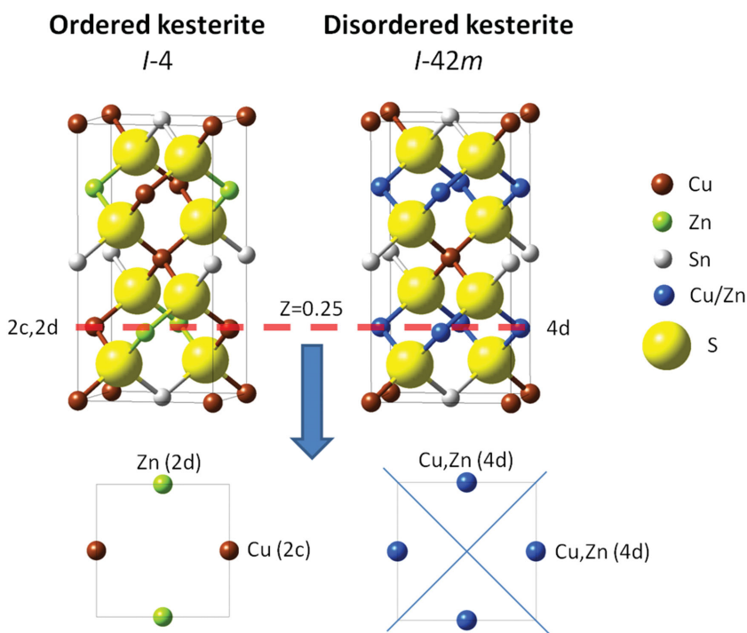
Figure 5. Representations of the ordered ( I-4 ) and disordered ( I-42m ) CZTS kesterite crystal-line structures. A projected view of the z = 0.25 plane is shown at the bottom. Adapted with permission. [71]
