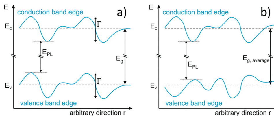
Figure 4. The effect of a) electrostatic potential fluctuations and of b) bandgap fluctuations. In each case radiative transitions at energies below the (average) bandgap are possible. Note that the bandgap in a) is constant and not affected by local charged defects, while band edges in b) can differ depending on e.g., long range composition variations.
