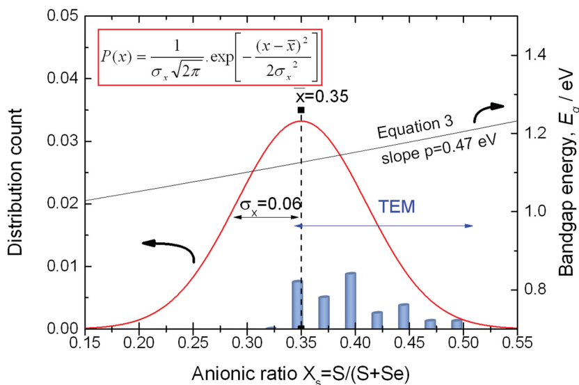
Figure 12. Composition distribution of anion ratio x = S/(S+Se) in our standard CZTSSe films, centered on x = 0.35 as derived from XRD and with standard deviation \sigma_x = 0.06 overestimated, compared with full pattern matching (e.g. Figure 11b). The blue bars are the indicative distribution measured by TEM (Figure 10c). The black line corresponds to a theoretical bandgap calculated using Equation (3), the slope of which ( p = 0.47 eV around x = 0.35 ) is used to derive \sigma_{E_g} = p \cdot \sigma_x .
