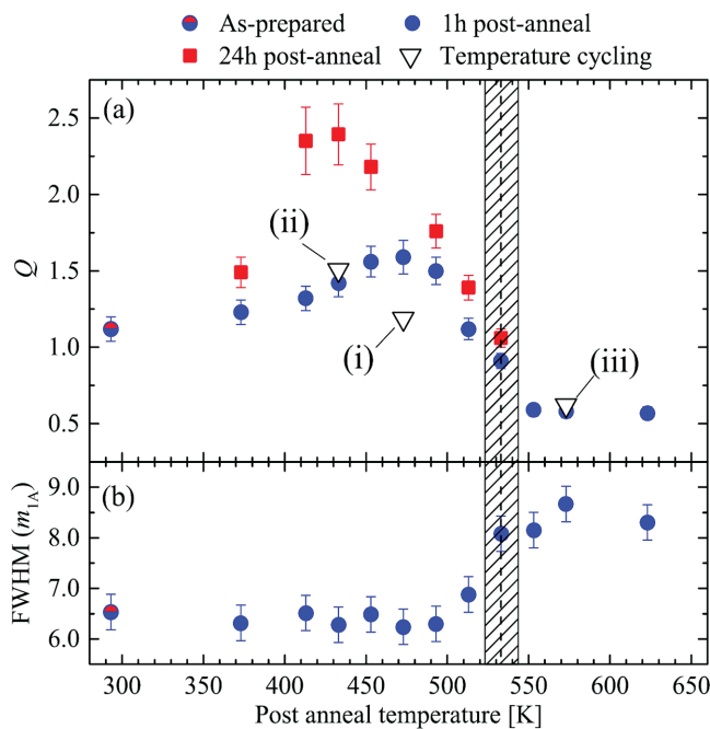
Figure 6. Variation in Q defined as Q = I(m_{2A}) / I(m_{3A}) for initially identical CZTS films post-annealed for different time periods. The triangles show the effect of temperature cycling on a single sample to test the reversibility of changes in Q . The shaded region indicates the probable location of the critical temperature T_c . Reproduced with permission. [8] Copyright 2014, AIP Publishing LLC.
