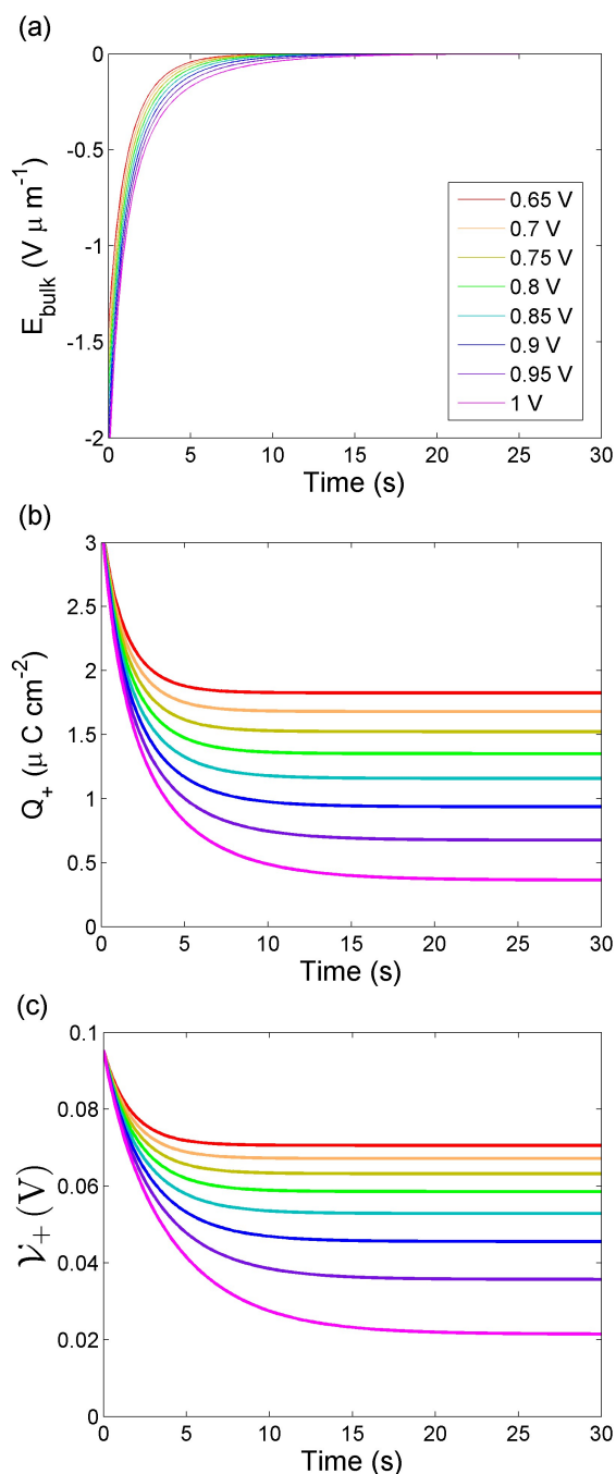
Fig. 6 Simulated (a) electric field E_{\text{bulk}} between the Debye layers; (b) charge per unit area in the Debye layer next to the spiro; and (c) voltage drop V_+ across the same Debye layer.
