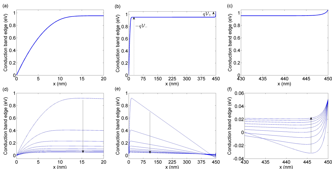
Fig. 4 Conduction band edge (CBE) across the 450 nm thick perovskite layer at 298 K, relative to the CBE immediately next to the titania. The central panels b and e show the entire perovskite layer. The left panels a and d show a close up of the Debye layer next to the titania; the right panels c and f show the Debye layer next to the spiro. Upper panels: CB profile after the cell has been held at 0 V for 30 s, before the voltage jump. Lower panels: Evolution over time of the CB profile for the first 8 s after switching the applied voltage from 0 V to V_{jump}=1 V. The arrow indicates the direction of increasing time; the first line depicts the system immediately after the voltage jump at t=0 s, with successive lines at 1 second intervals.
