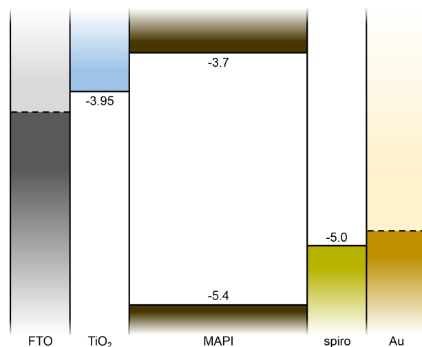
Fig. 1 Band diagram of the device. Band edges for the perovskite and transport layers are represented by solid lines, with energies relative to the vacuum level in eV labelled 56 . Fermi levels for the contacts are depicted by dotted lines – values for these levels were not required by the model and are difficult to measure accurately, so are not given.
