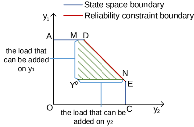
Fig. 4 Available capacity interval
