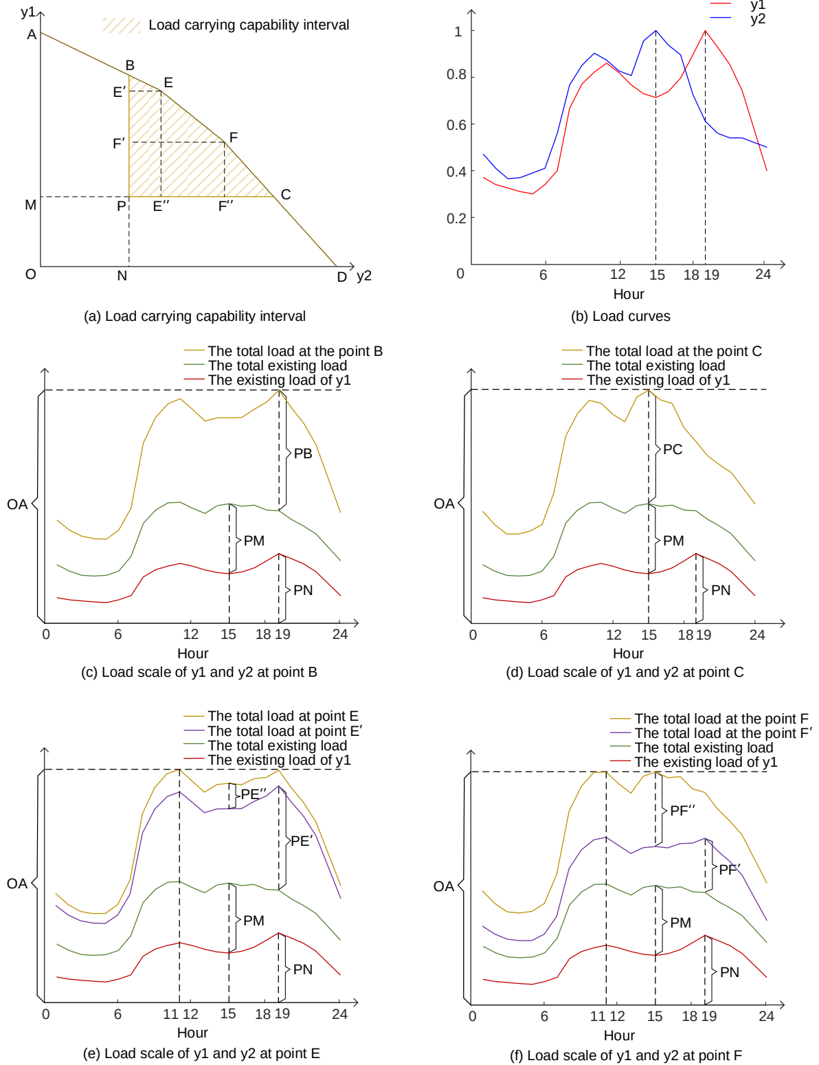
Fig. 5 Load carrying capability interval
