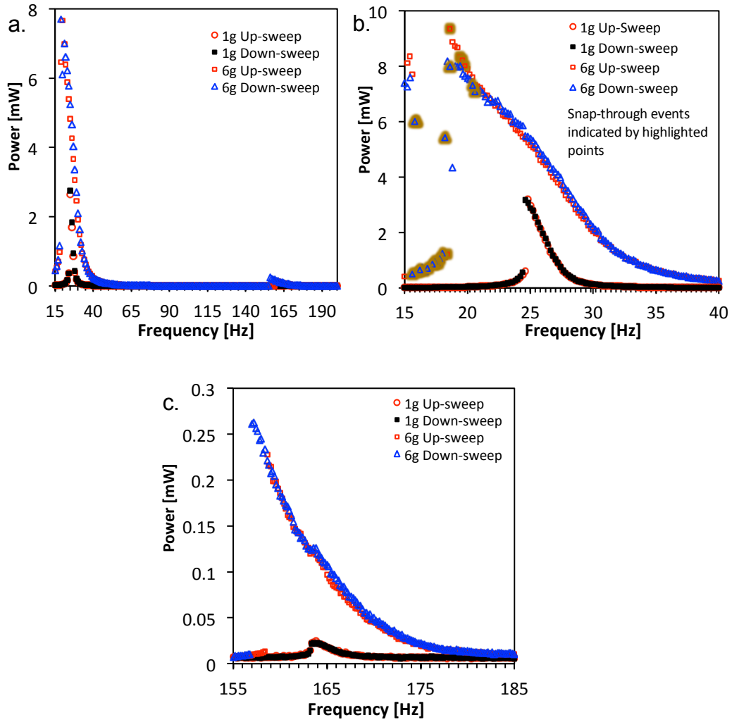
Figure 7. Power versus frequency for 1g and 6g for linear beam (a) frequency range 15-200Hz (b) detailed view of 2 nd mode (c) detailed view of 3 rd mode.
