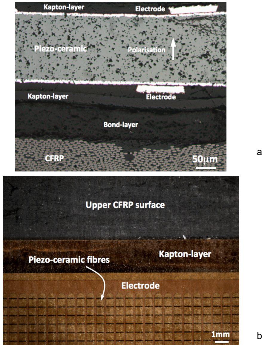
Figure 3. (a) Cross-section of MFC-carbon epoxy laminate (b) top-down view of piezoelectric showing piezoelectric fibres and electrode structure.
