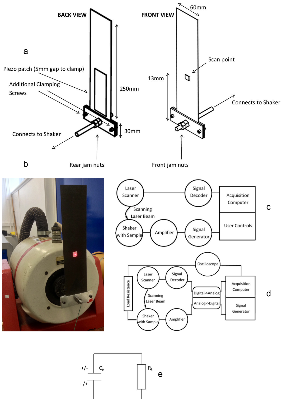
Figure 4. Experimental setup: (a) clamped cantilever beam; (b) cantilever energy harvester on the shaker and reflective tape; (c) schematic of the experimental setup for frequency response function; (d)
