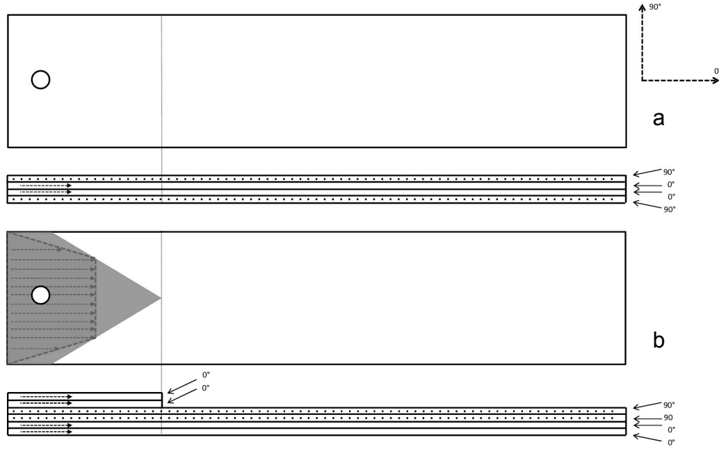
Figure 2. Laminate lay-ups (a) linear [90/0/0/90]_T , (b) bistable [0/0/90/90]_T . The cantilevers were clamped at the left hand side.
