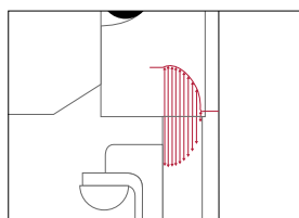
Fig. 1.14b: Opening forces from combined hydrostatic and hydrodynamic pressure distribution
