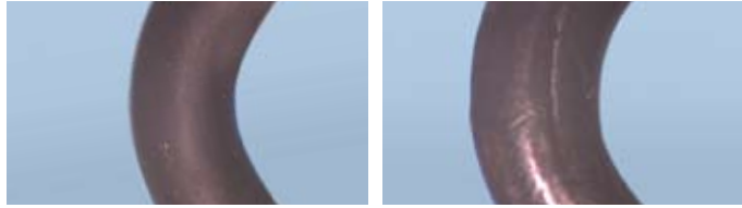
Fig. 5.8: A fresh EPDM O-ring (left) and a swollen EPDM O-ring (right) exposed to water containing mineral oil
