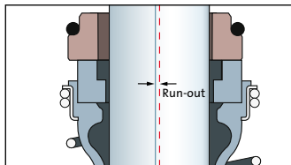
Fig. 5.15: Shaft seal with radial run-out
