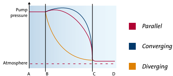
Fig. 1.22: Hydrostatic and hydrodynamic pressure distribution for different sealing gap geometries
