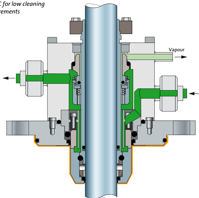
Fig. 2.10: Example of complex sanitary agitator seal subject to the highest sterilisation and cleanability requirements. The barrier fluid (green) can be steam condensate. Surfaces marked with yellow are electro-polished. Secondary seals on medium side have been modified, leaving no gaps
