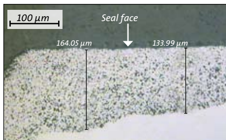
Fig. 5.9: Selective corrosion in cemented tungsten carbide. The metallic binder phase is corroded resulting in reduced wear resistance
