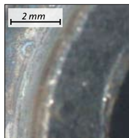
Fig. 5.9: Selective corrosion in cemented tungsten carbide. The metallic binder phase is corroded resulting in reduced wear resistance
