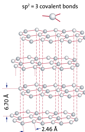
Fig. 3.10: Carbon atoms in the lattice structure of graphite ( sp^2 bonds)
