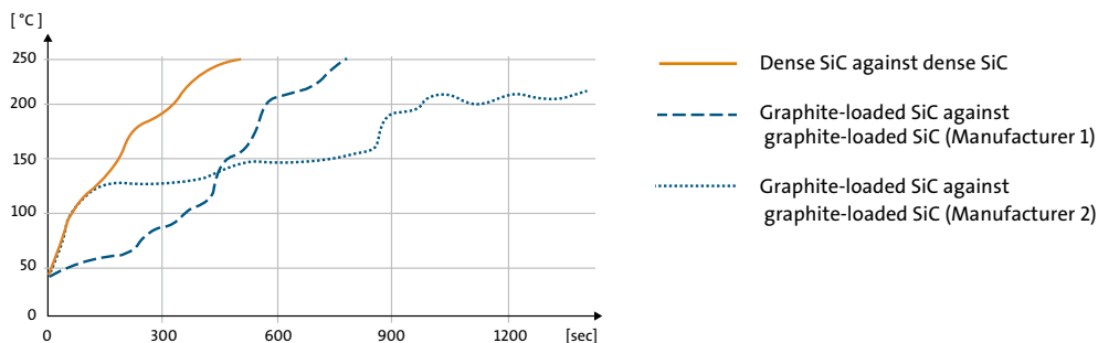
Fig. 3.18: Temperature on seat at dry running of seals with different SiC grades
