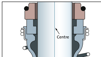
Fig. 5.14: Well-aligned shaft seal
