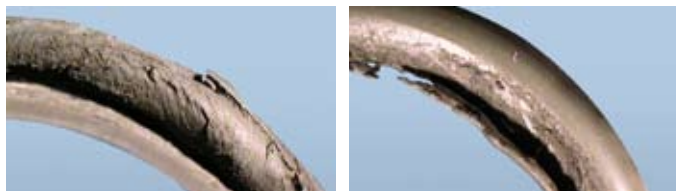
Fig. 5.19: O-rings extruded on account of high pressure
