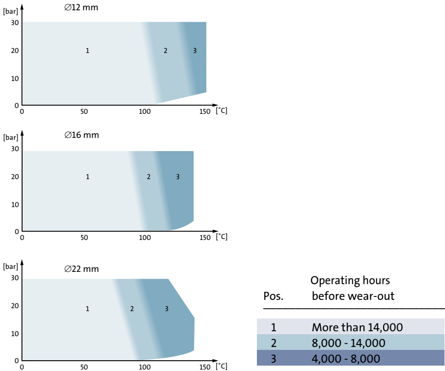
Fig. 3.11: Pressure/temperature diagrams showing operating life of Grundfos type H carbon graphite/WC shaft seals in water at three different shaft diametres
