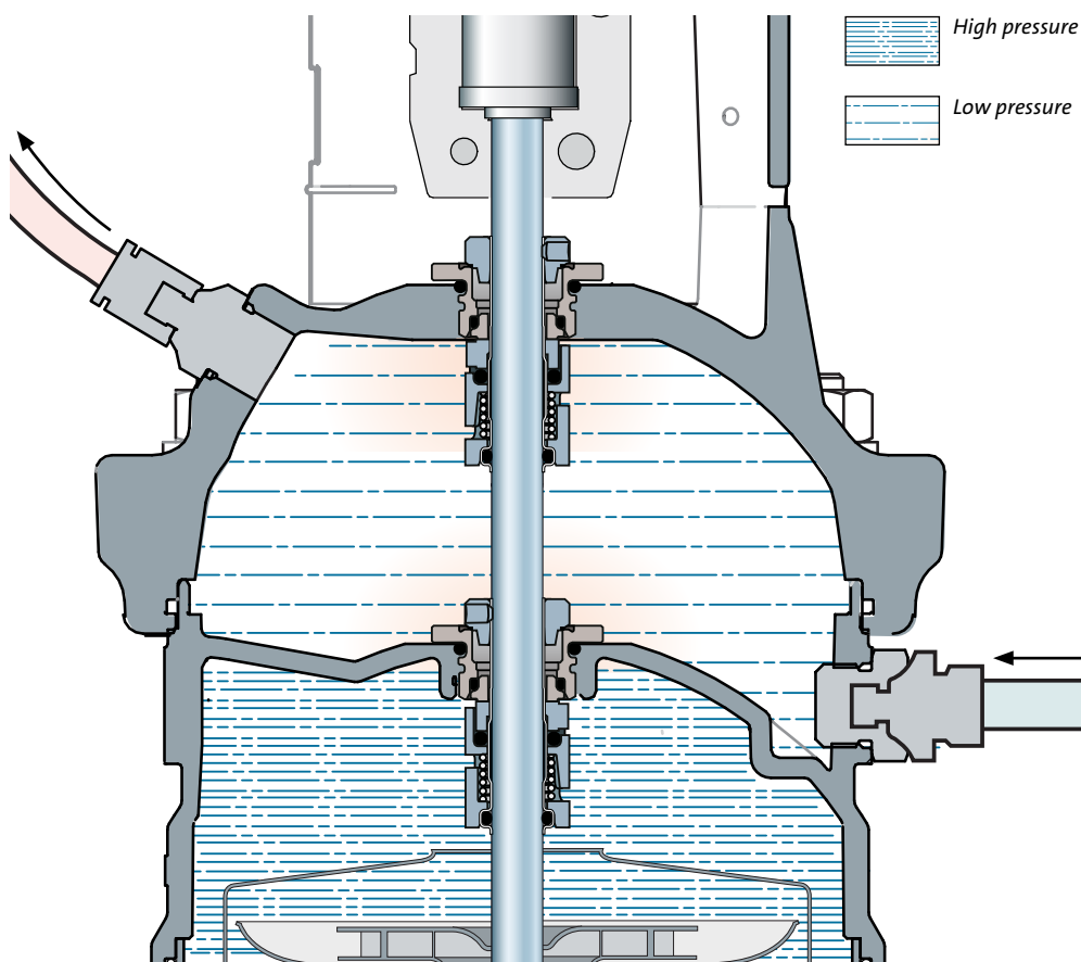
Fig. 2.6: Grundfos CR pump with a tandem seal arrangement
