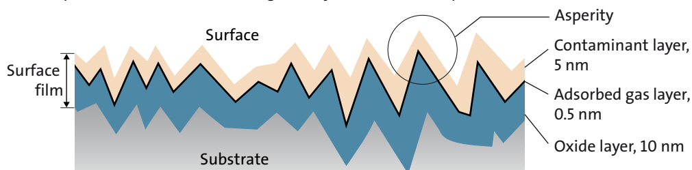
Fig. 4.12: Surface of a material with contaminants
