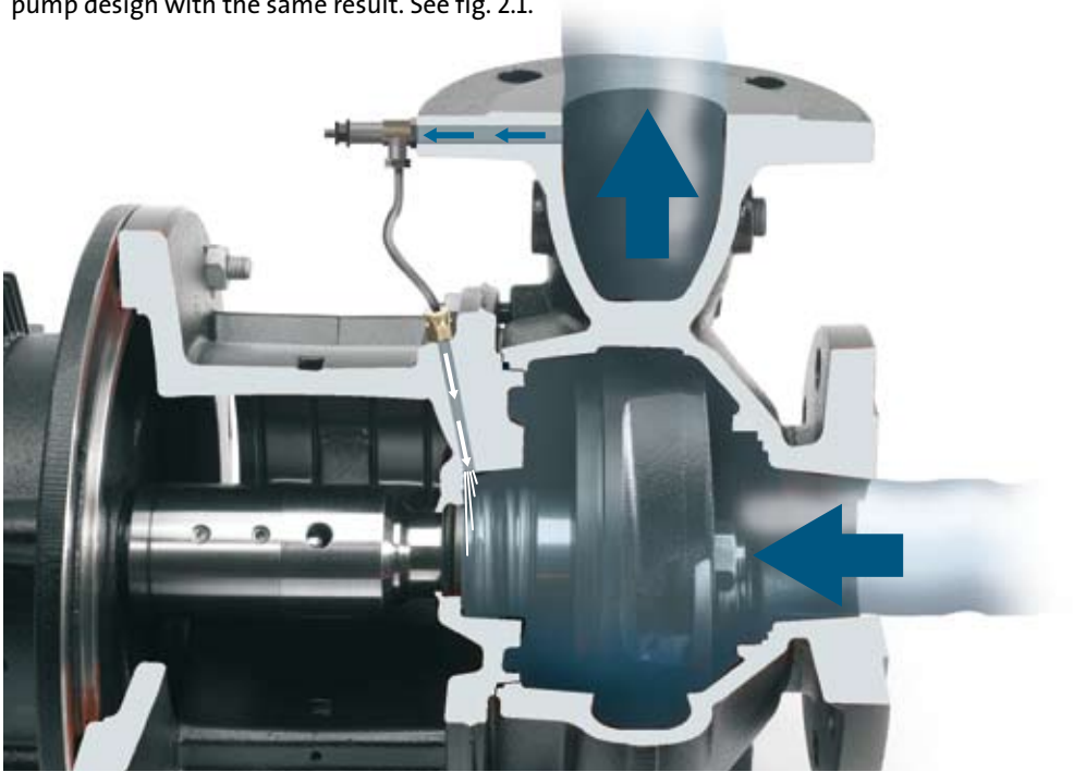
Fig 2.1: Circulation circuit for cooling a single mechanical shaft seal
