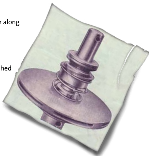
Fig. 1.27: Original illustration of CP pump shaft seal from the "Grundfos pump magazine", 1956
