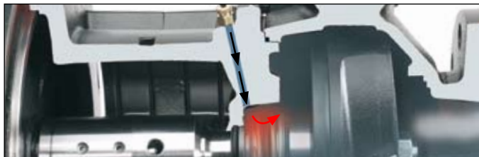
Fig. 5.20: Removal of frictional heat by means of circulating the pumped medium across the shaft seal in the seal chamber
