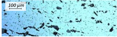
Fig. 3.8: Micrograph showing surface of graphite-loaded silicon carbide
