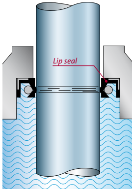
Fig. 1.3: Lip seal
