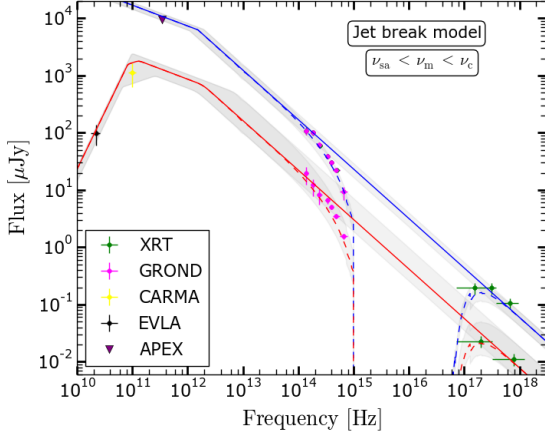
(a) Jet break: \nu_{sa} < \nu_m < \nu_c
