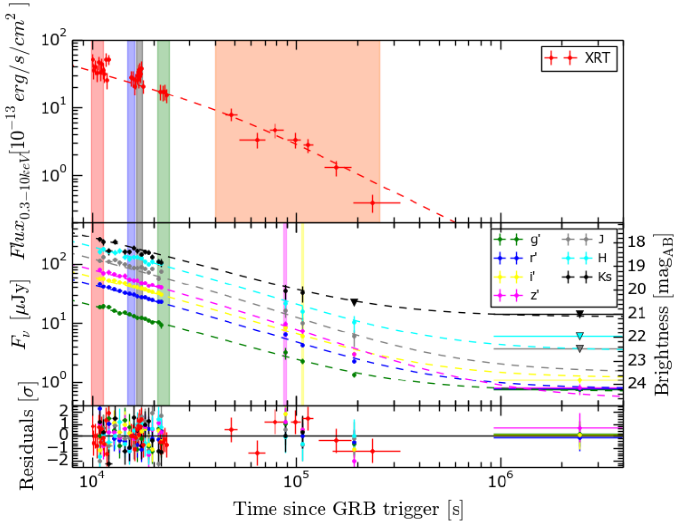
Fig. 2: Light curve of the afterglow of GRB 121024A. Top: XRT light curve from the XRT repository. Bottom: GROND light curve in g'r'i'z'JHK_s . The best fit for the combined light curve (optical/NIR and X-ray data) is a smoothly broken power law with host contribution, shown with dashed lines. The epochs used for the spectral analysis are highlighted with the vertical bars. The break time t_b = 49.8 \pm 5.1 ks.
