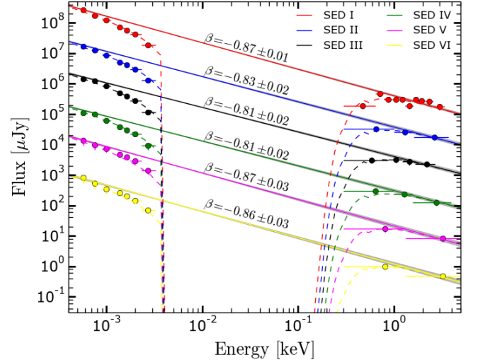
Fig. 3: Spectral energy distribution for the six SEDs highlighted in Fig. 2. SEDs I - IV are from data before the observed break in the light curve. SEDs V and VI are from data taken after the break. The SEDs are scaled with an arbitrary factor for clarity in the plot. The values of \beta written above each line corresponds to the single power-law fit, where the slopes were left free to vary. The single power-law fit with a single tied slope has \beta = 0.86 \pm 0.02 .
