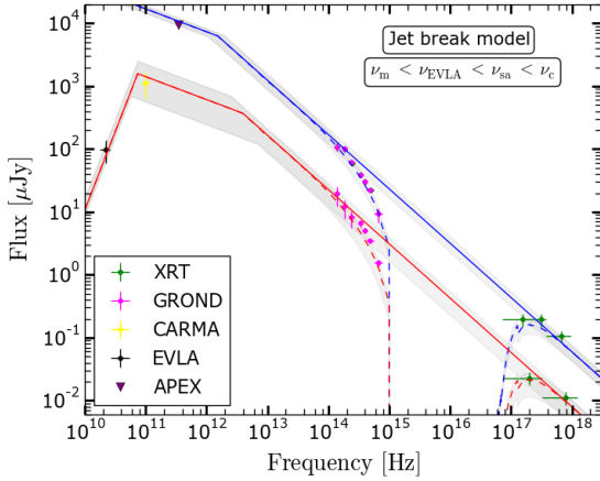
(b) Jet break: \nu_m < \nu_{sa} < \nu_c
