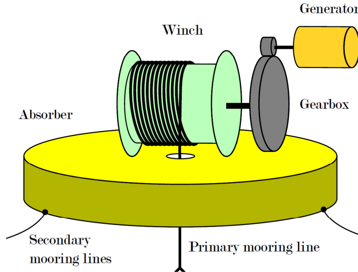
Figure 5: Schematic for Power Take-Off (PTO) system and primary mooring line [37]. Reproduced with permission from the author.
