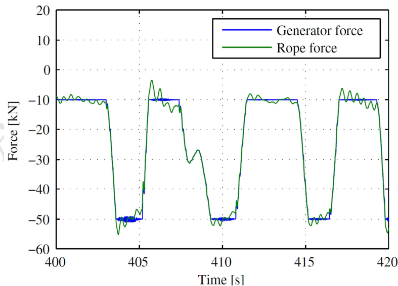
Figure 6: Oscillations encountered in primary moorings due to system dynamics [37]. Reproduced with permission from the author.
