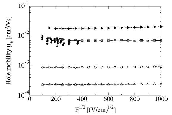
Fig. 4. Poole–Frenkel plot for predicted \mu_h compared to experimental data [26] (•) in an aligned PFO film at T = 300 K and a fixed interchain separation \Delta r = a = 0.65 nm, where F is parallel to x . Predicted \mu_h values are shown for the ordered system devised to maximize \mu_h (filled right triangles); the ordered system with fixed \varphi = 20^\circ (◊), with fixed \varphi = 0^\circ (Δ) and a lateral and torsionally disordered system (■). The lines are to guide the eye. (Taken from [12].)
