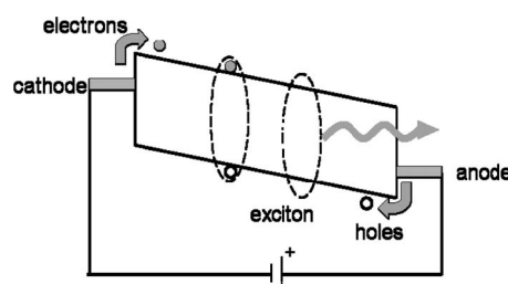
Fig. 2. Schematic diagram of OLED operation.
