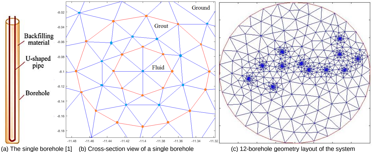
FIGURE 3 The layout and geometry of boreholes
