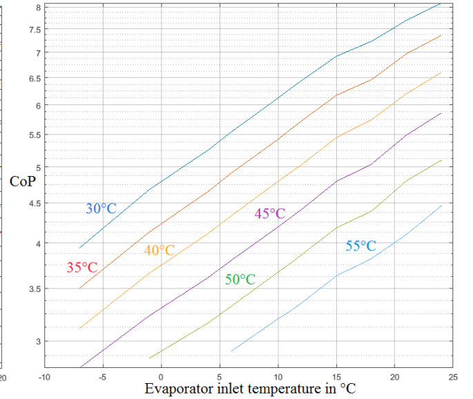
FIGURE. 6 GSHP CoP in different outlet temperature categories
