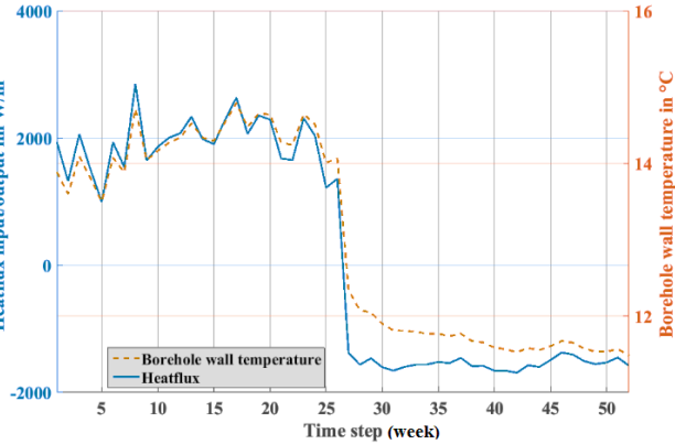
FIGURE. 9 Case 2 borehole wall temperature response to heat flux
