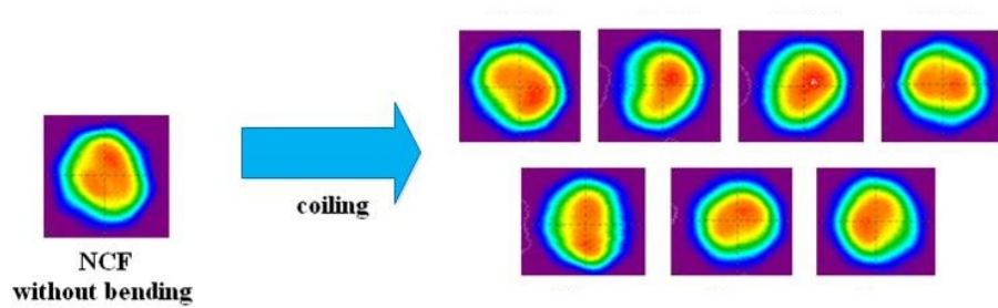
Fig. 4. Different fiber-delivered near-field beam profiles for different diameter fiber coils.
