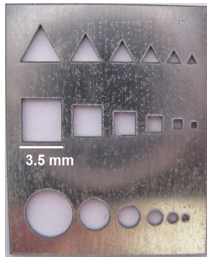
Fig. 12. Example of cutting through of the 0.3 mm thick aluminum sheet with the ns laser.
