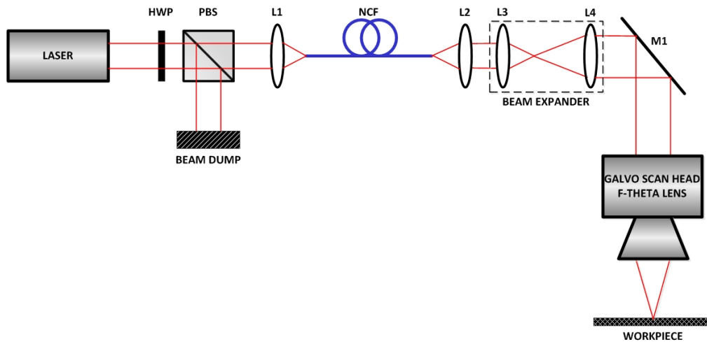
Fig. 11. The experimental setup for ns and ps fiber-based micro-machining. HWP: half-wave plate; PBS: polarizing beam splitter; L: lens; M: mirror.
