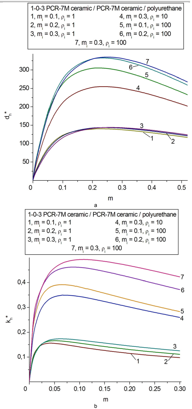
Figure 9. Correlation between the hydrostatic piezoelectric coefficient d_h^* (a, in \text{pC} / \text{N} ) and hydrostatic ECF k_h^* (b) in the 1–0–3 PCR-7M ceramic / polyurethane composite
