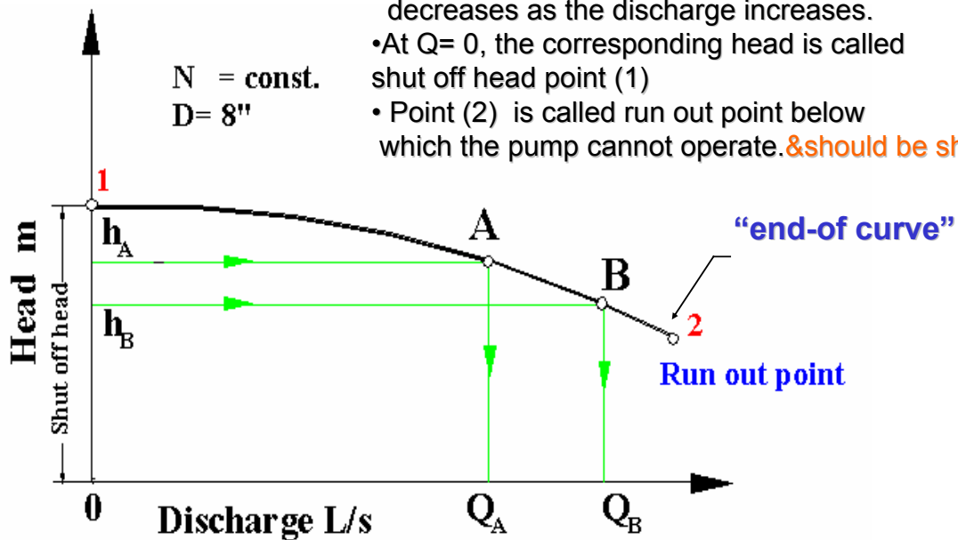
Head capacity curve
