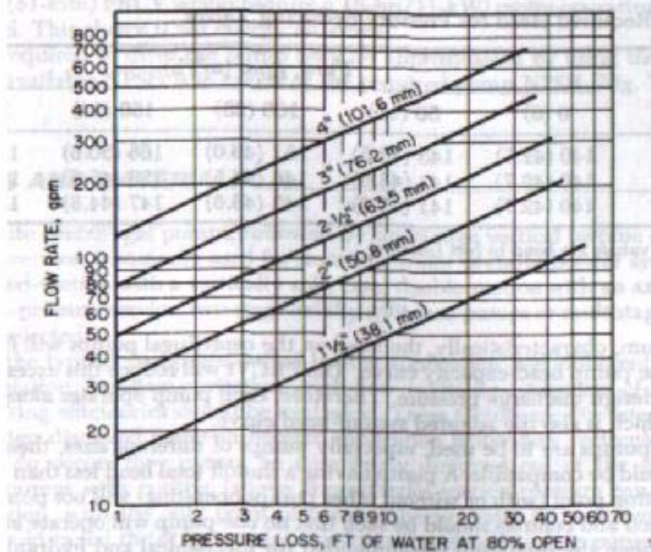
FIG. 6 Typical PRV or PRCV flow chart. (ft \times 0.3048 = m; gpm \times 0.2271 = m 3 /h; in \times 25.4 = mm) (Cla-Val)
