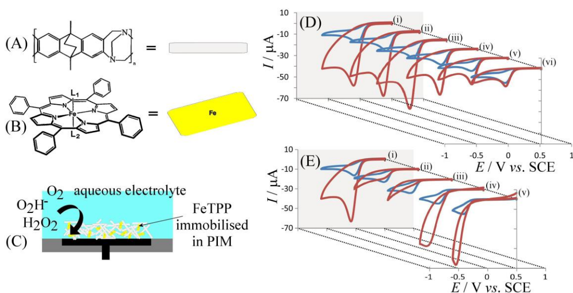
Figure 6. (A) Molecular structure of PIM-EA-TB and (B) of FeTPP. Schematic drawings of (C) FeTPP immobilised into the rigid microporous structure. (D) Cyclic voltammograms (scan rate 20 \text{ mVs}^{-1} ) for the reduction of ambient oxygen (blue) and 4 \text{ mM H}_2\text{O}_2 (red) at electrodes coated with (i) 1:1, (ii) 1:2, (iii) 1:5, (iv) 1:10, (v) 1:20, and (vi) 1:40 weight ratio FeTPP:PIM immersed in aqueous 0.1 \text{ M} phosphate buffer pH 2. (E) Cyclic voltammograms (scan rate 20 \text{ mVs}^{-1} ) for the reduction of ambient oxygen (blue) and 4 \text{ mM H}_2\text{O}_2 (red) at electrodes coated with 1:5 FeTPP:PIM immersed in aqueous 0.1 \text{ M} phosphate buffer at pH (i) 2, (ii) 4, (iii) 7, (iv) 9, and (v) 12 (reprinted with permission [52] ).
