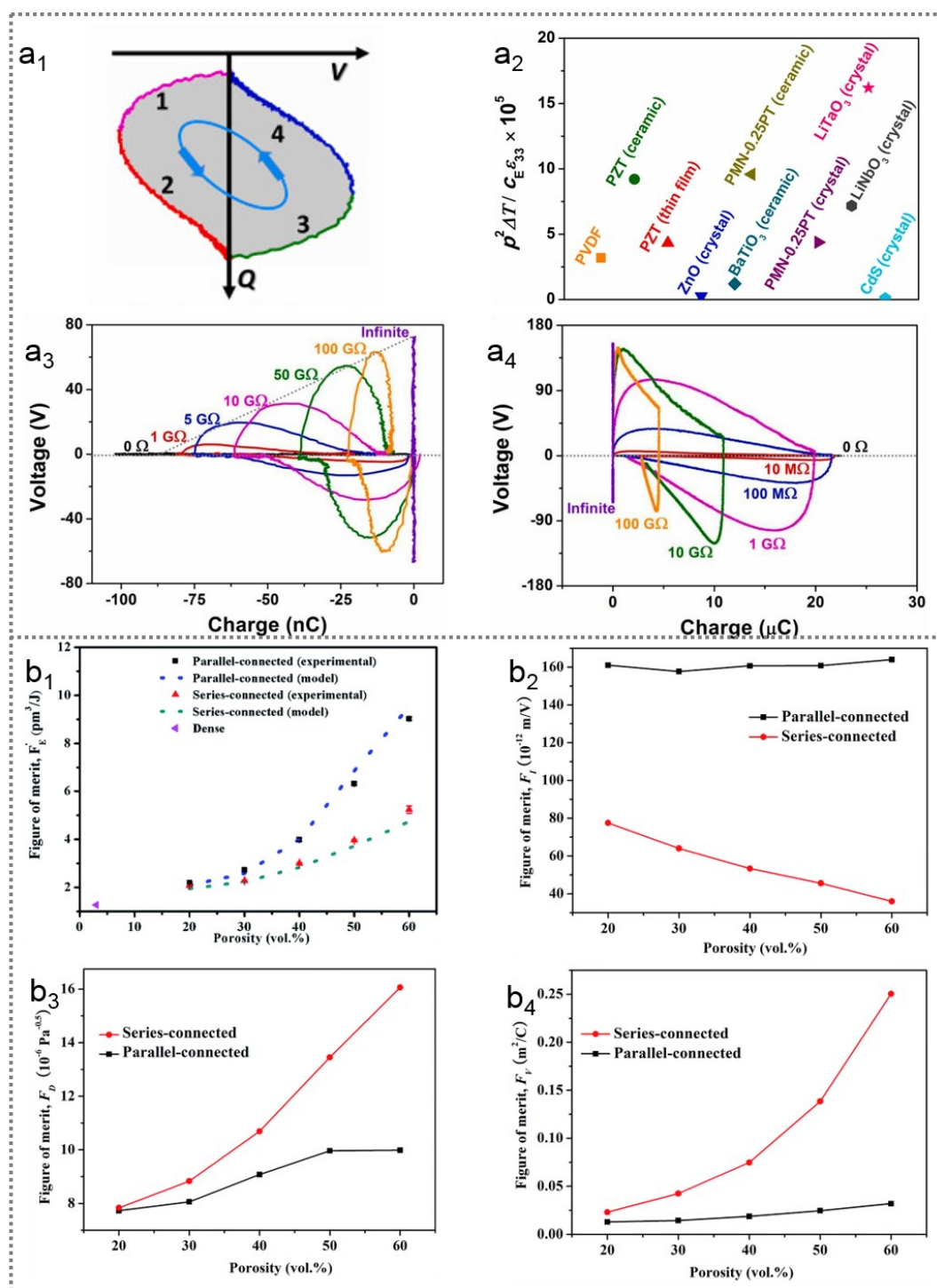
Figure 5. Figures of merits for pyroelectric nanogenerators. a) a 1 ) Charge-voltage (Q-V) cycle of a pyroelectric nanogenerator, a 2 ) Figure-of merit ( FE'' ) for different types of pyroelectric materials, a 3 , a 4 ) Q-V cycles of a 3 ) PVDF device and a 4 ) PZT device under different load resistances. Reproduced with permission. [198] Copyright 2019, Elsevier. b) b 1 ) Porosity dependence of experimental and modelling pyroelectric figure of merit of porous PZT ceramics, b 2 ) Current responsivity F_I , b 3 ) F_D , b 4 ) voltage responsivity F_V . Reproduced with permission. [142] Copyright 2017, Royal Society of Chemistry.
