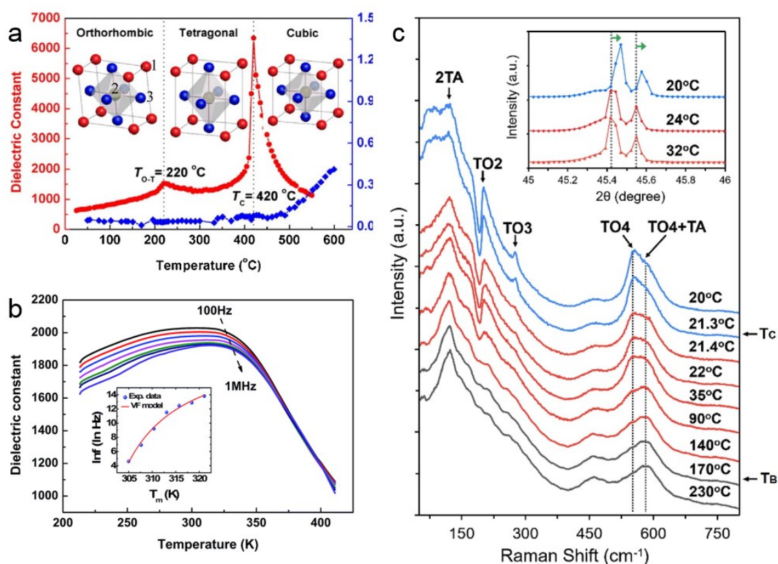
Figure 2. a) Normal ferroelectric phase transition. Temperature-dependent dielectric permittivity and loss of \text{K}_{0.5}\text{Na}_{0.5}\text{NbO}_3 ceramics. Relxor ferroelectric phase transition. Reproduced with permission. [197] Copyright 2013, American Chemical Society. b) Temperature and frequency dependent dielectric constant of the 0.6\text{BaTiO}_3@0.4\text{SrTiO}_3 bulk ceramic. Reproduced with permission. [102] Copyright 2015, The Royal Society of Chemistry. c) The Raman spectra of \text{KTa}_{0.61}\text{Nb}_{0.39}\text{O}_3 at different temperatures. Reproduced with permission. [103] Copyright 2019, Elsevier.
