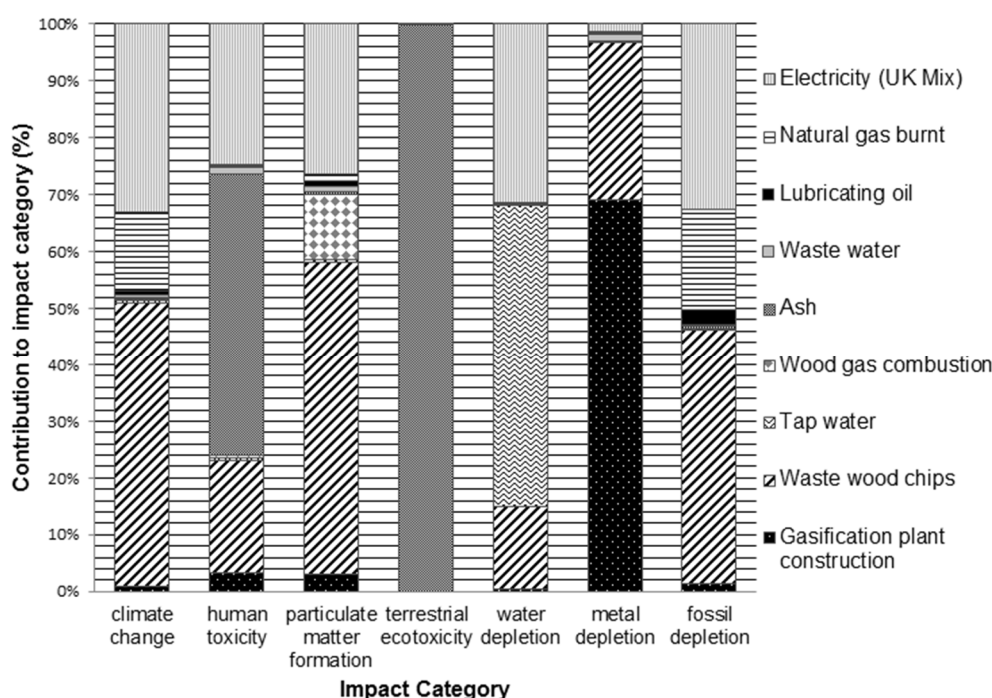
Figure 5: Characterised data for annual biomass gasification plant operation (ReCiPe midpoint [H] v1.01)
