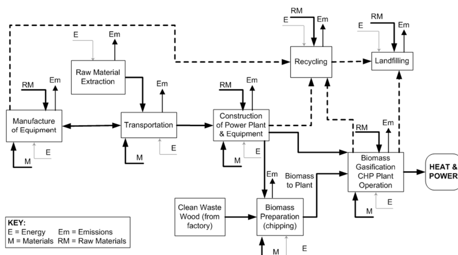
Figure 3: Overview of the system boundary for the biomass gasification plant construction and operation [10].
