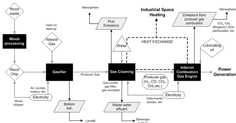
Figure 2: Description of the biomass gasification CHP system with main inputs, processes, outputs and emissions
