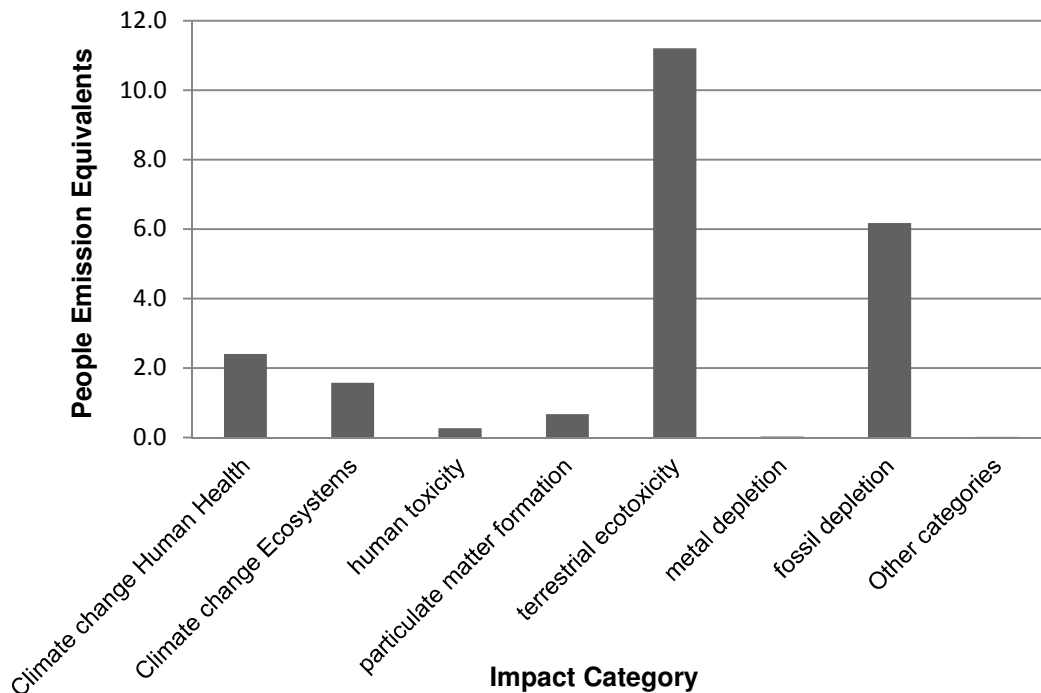
Figure 4: Normalised data for annual biomass gasification plant operation (ReCiPe endpoint [H] v1.01)
