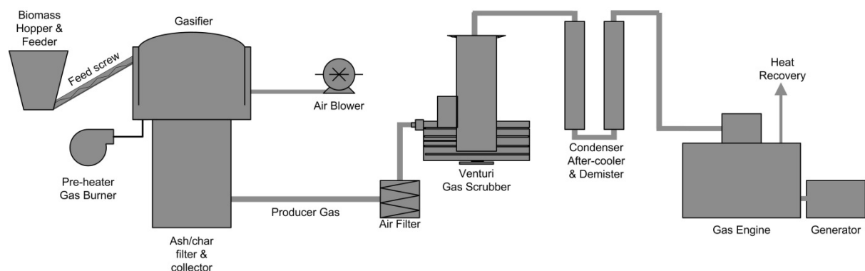
Figure 1: Simplified Schematic of the Gasification Process
