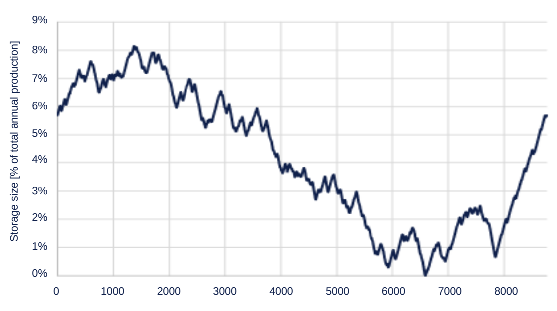
Example of the percentage of hydrogen in storage from wind turbines. Source: DNV.
