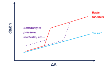
Fatigue crack growth rate
