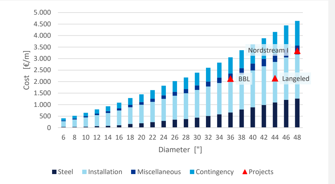
Investment figures for hydrogen pipelines depending on the diameter. Source: DNV reference database.
