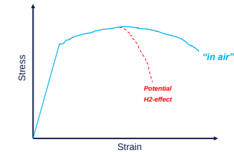
Stress-strain curve
