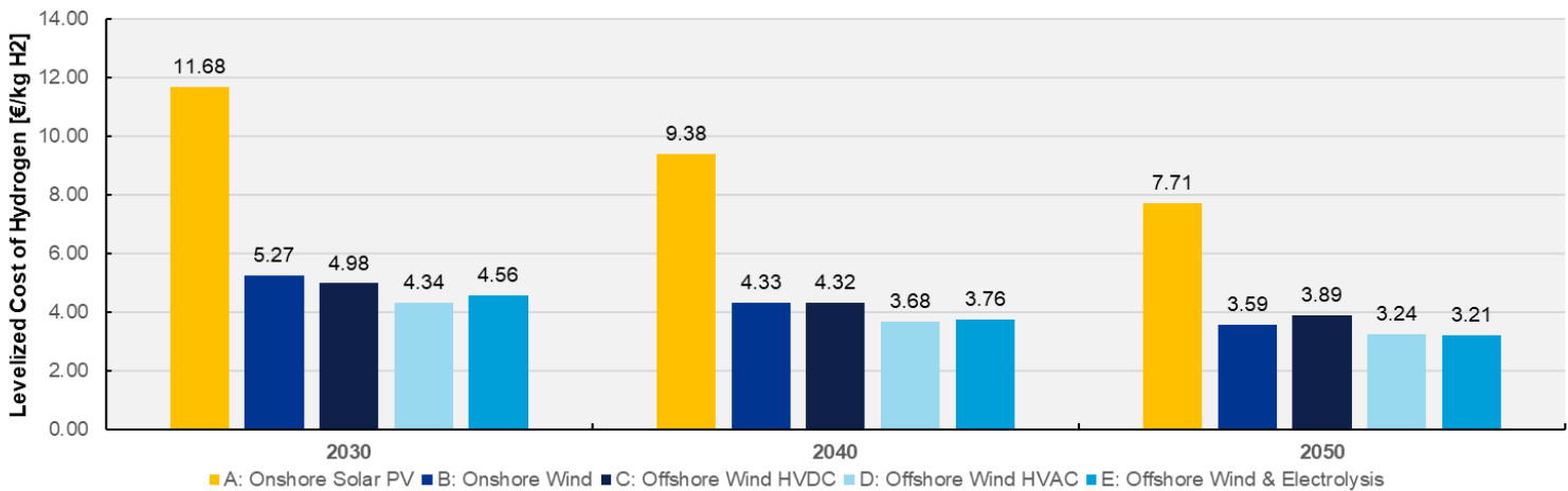
High-level cost calculations for various Northern European hydrogen value chains
