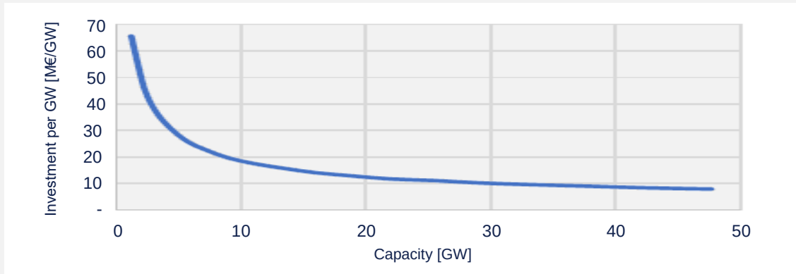
Specific investment cost for a hydrogen pipeline with increasing pipeline capacity (assumed inlet pressure: 100 barg, outlet pressure 30 barg, length 100 km). Source: DNV
