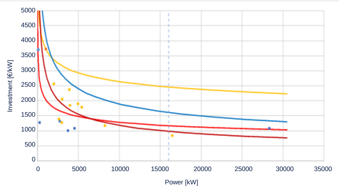
Investment figures for hydrogen compressors. Dots are individual reference prices and lines represent fitted models. Source: DNV reference database.
