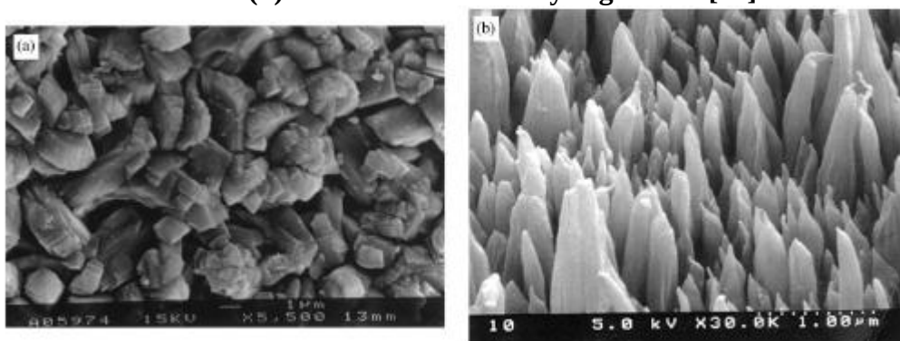
Figure 1 Examples of rough pretreated substrate surfaces. (a) Phosphated steel prepared for rubber bonding [cf. 19] (b) P.T.F.E. irradiated by argon ions [20].
