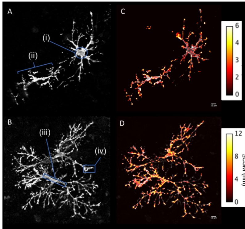
Figure 4. Mouse cortical neurons ('Cell 1', Panel A and 'Cell 2', Panel B) treated with 500 nM A\beta_{15-21} -fluor, analyzed by high resolution fluorescence microscopy. Labels i-iv show specific morphological features, likely corresponding to the cell body (i), dendrite (ii) periaxonal region (iii) and synapses (iv). C and D show the corresponding false color map of \Delta CSM = CSM \lambda_{Ex514nm} - CSM \lambda_{Ex458nm} extracted from emission spectra of each image.
