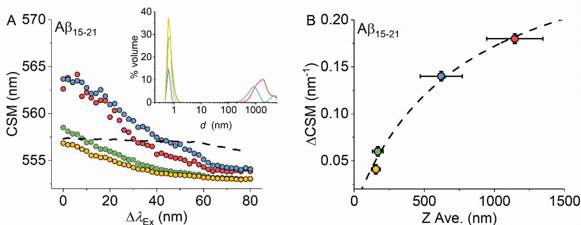
Figure 3. A , Edge-shift measurements demonstrating sensitivity between monomerized and aggregated states (shown as differently colored data points) of fluor- A\beta_{15-21} and coloration is correlated between main panel and inset . The black dashed-line shows the data for fluorescein alone. Inset , DLS data for monomerized and aggregated fluor- A\beta_{15-21} . Coloration corresponds to aggregation state shown in inset . B , Correlation between the change in CSM ( \Delta CSM ) for fluor- A\beta_{15-21} shown in Panel A. The Z-average hydrodynamic diameter from the DLS data shown in Panel A. Coloration is as Panel A.
