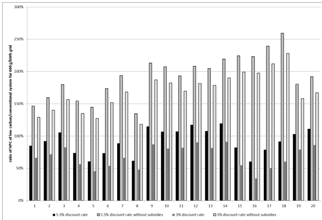
Figure 9 ratio of NPC for low carbon system to standard system with grid intensity of 600g/kWh
