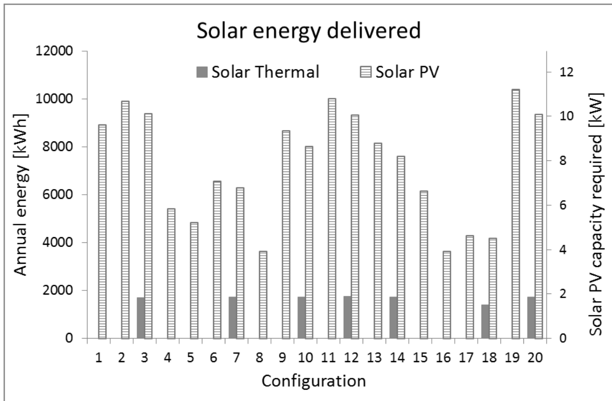
Figure 3 : Solar energy delivered
