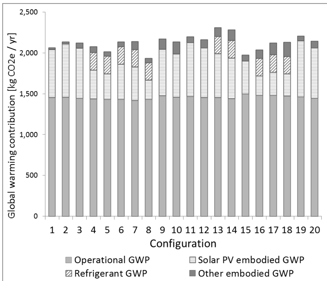
Figure 5 Green house gas emissions for configuration considered
