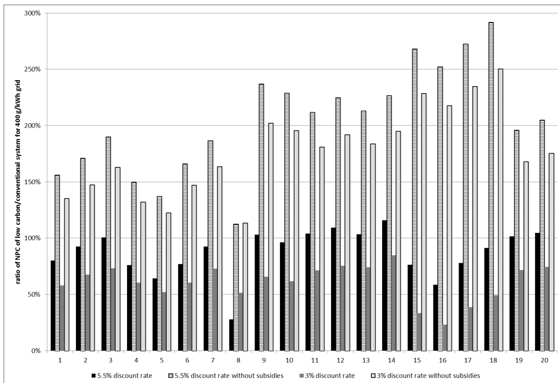
Figure 10 ratio of NPC for low carbon system to standard system with grid intensity of 400g/kWh
