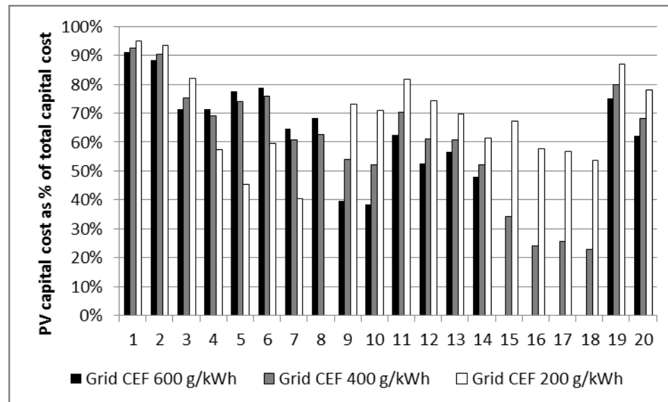
Figure 13 PV costs as % of total capital costs
