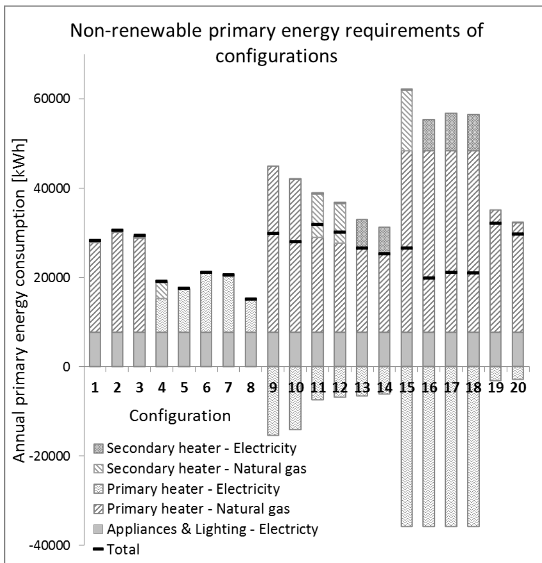
Figure 2: Non-renewable primary energy requirements
