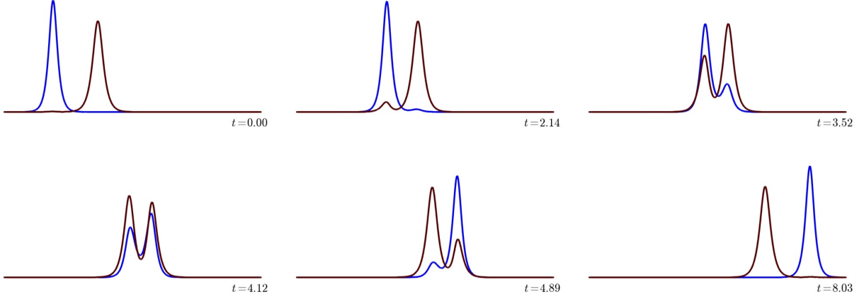
FIGURE 6. Here we show the dynamics of the approximation generated by the conservative discretisation scheme with polynomial degree q = 1 approximating a smooth solution with initial conditions given by (5.5).
