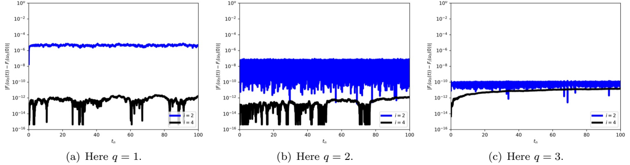
FIGURE 1. Here we examine the conservative discretisation scheme with various polynomial degrees, q , approximating the exact solution (2.21) with initial conditions given by (5.2). We show the deviation in the two invariants F_i , i = 2, 4 , corresponding to momentum and energy. In each test we take a fixed spatial discretisation parameter of h = 0.25 and fixed time step of \tau = 0.001 . Notice that in each case the deviation in energy is smaller than the solver tolerance of 10^{-12} and the deviation in momentum is bounded. In addition, as the degree of approximation is increased the deviation in momentum becomes smaller, in this case by around two orders of magnitude per polynomial order. The simulations are simulated for long time to test conservativity with T = 100 in each case.
