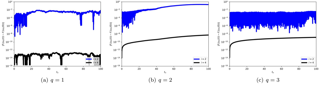
FIGURE 10. Here we examine the conservative discretisation scheme with various polynomial degrees, q , approximating the solution to (2.2) with initial conditions given by (5.8). We show the deviation in the two invariants F_i , i = 2, 4 , corresponding to momentum and energy respectively. In each test we take a fixed spatial discretisation parameter of h = 0.25 and fixed time step of \tau = 0.001 . Notice that in each case the deviation in energy is smaller than the solver tolerance of 10^{-12} and the deviation in momentum is bounded. The simulations are simulated for long time to test conservativity with T = 100 in each case.
