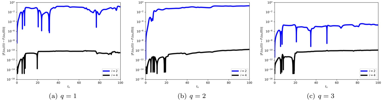
FIGURE 8. Here we examine the conservative discretisation scheme with various polynomial degrees, q , approximating the solution to (2.2) with initial conditions given by (5.7). We show the deviation in the two invariants F_i , i = 2, 4 , corresponding to momentum and energy respectively. In each test we take a fixed spatial discretisation parameter of h = 0.25 and fixed time step of \tau = 0.001 . Notice that in each case the deviation in energy is smaller than the solver tolerance of 10^{-12} and the deviation in momentum is bounded. The simulations are simulated for long time to test conservativity with T = 100 in each case.
