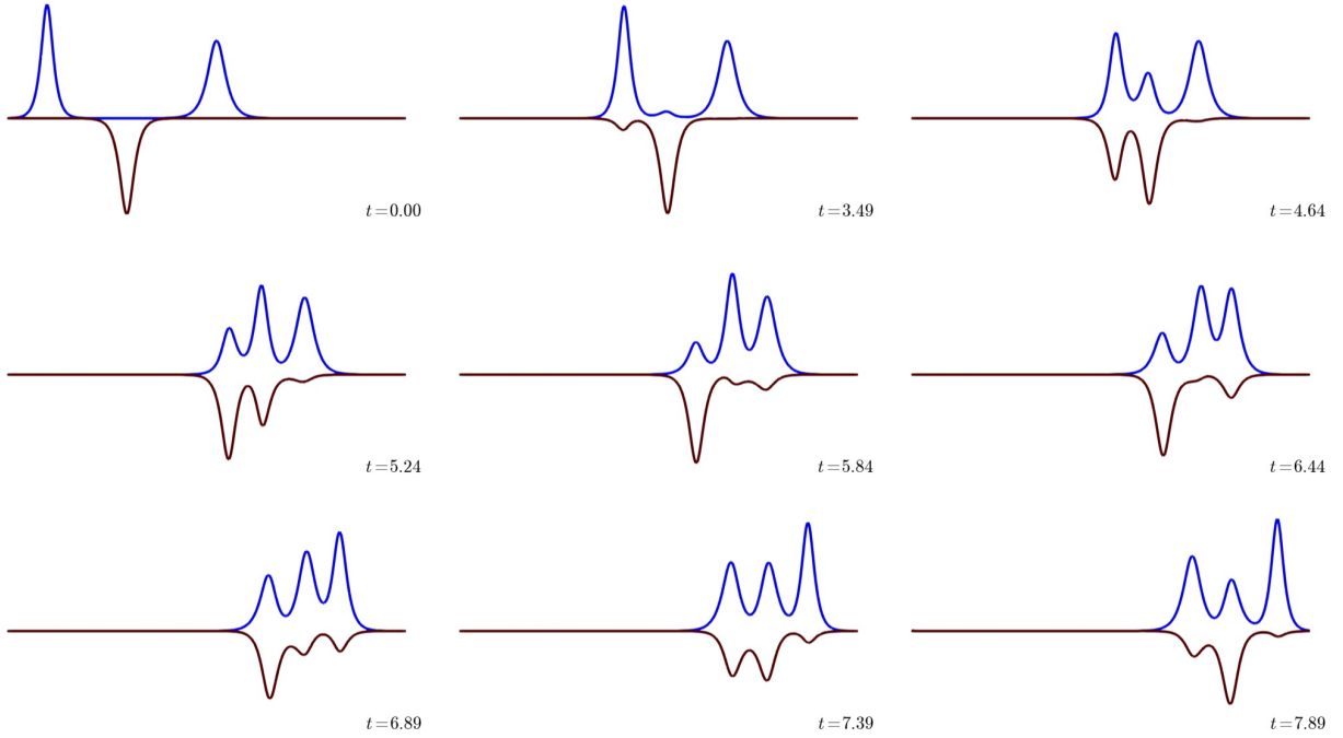
FIGURE 7. Here we show the dynamics of the approximation generated by the conservative discretisation scheme with polynomial degree q = 1 approximating a smooth solution with initial conditions given by (5.6).
