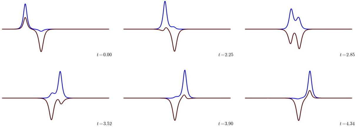
FIGURE 5. Here we show the dynamics of the approximation generated by the conservative discretisation scheme with polynomial degree q = 1 approximating a smooth solution with initial conditions given by (5.4).
