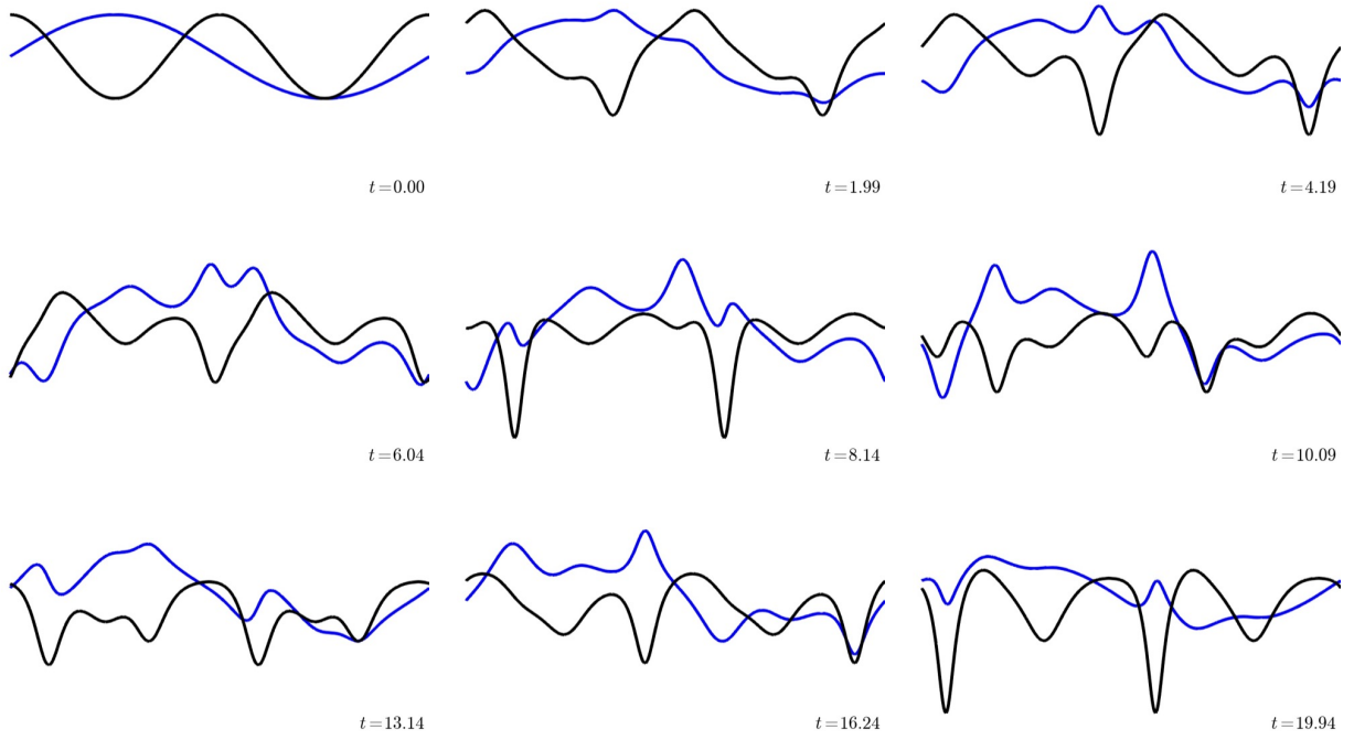
FIGURE 9. Here we show the dynamics of the approximation generated by the conservative discretisation scheme with polynomial degree q = 1 approximating the solution to (2.2) with initial conditions given by (5.8). Notice that initially, dispersive waves emanate from the discontinuity.
