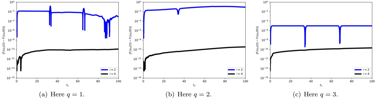
FIGURE 3. Here we examine the conservative discretisation scheme with various polynomial degrees, q , approximating the exact solution (2.22) with initial conditions given by (5.3). We show the deviation in the two invariants F_i , i = 2, 4 , corresponding to momentum and energy respectively. In each test we take a fixed spatial discretisation parameter of h = 0.25 and fixed time step of \tau = 0.001 . Notice that in each case the deviation in energy is smaller than the solver tolerance of 10^{-12} and the deviation in momentum is bounded. The simulations are simulated for long time to test conservativity with T = 100 in each case.
