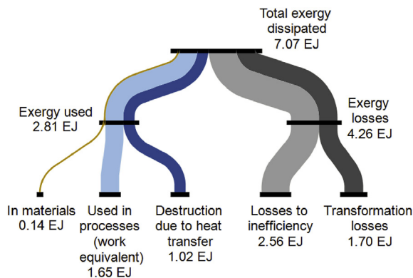
Fig. 2. Categorization of industrial exergy use (figures relate to UK industry, 2007).
