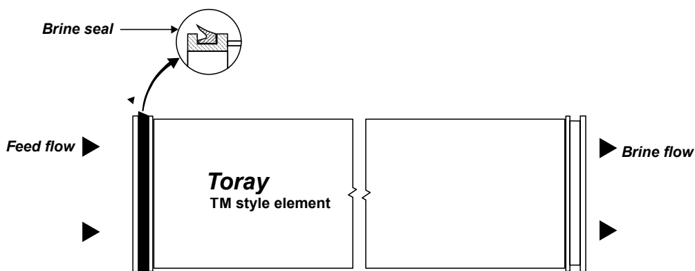
Figure TMM-200-4: Orientation of brine seal
