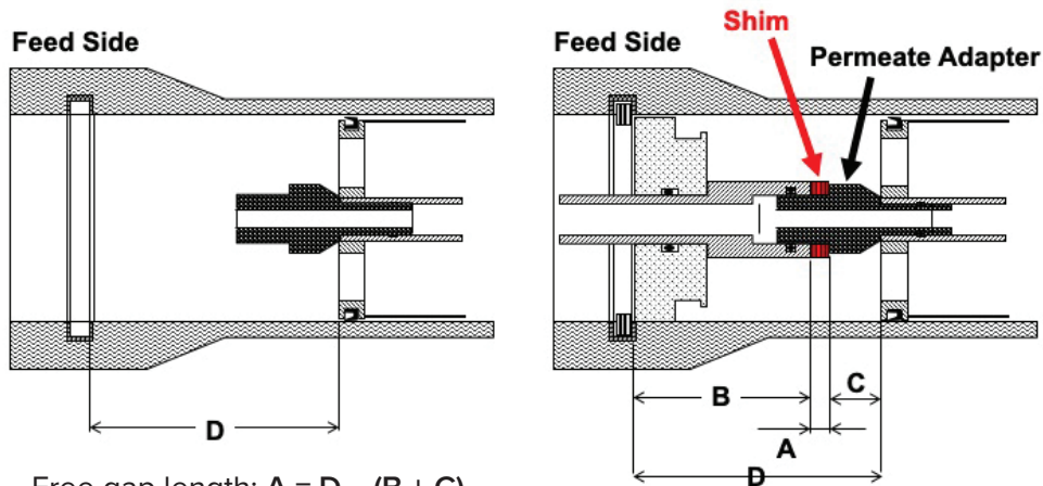
Figure TMM-200-9: Shimming procedure
