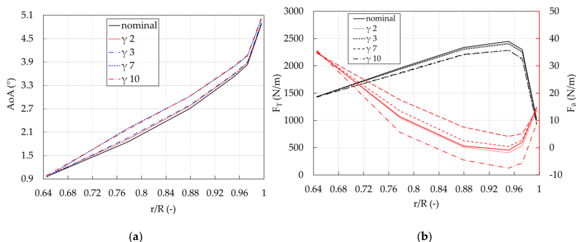
Figure 10. Relevant turbine figures: (a) Angle of attack along the outer part of the blade and (b) thrust ( F_t ) and tangential ( F_s ) for the outer part of the blade at 4 m/s mean wind speed.
