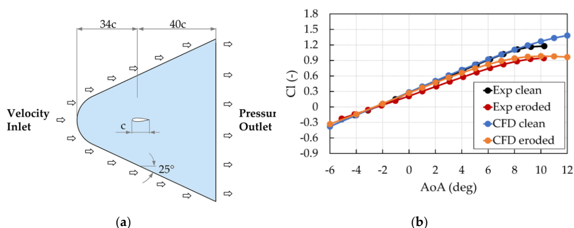
Figure 4. CFD validation. (a) Illustration of the adopted computational domain; (b) validation of the numerical setup in respect to data from [5] at Re=1.5 \times 10^6 .
