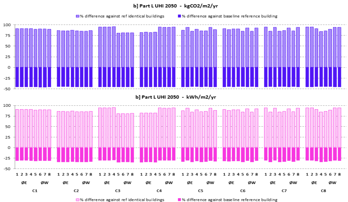
Figure 8. as figure 7 for low levels of internal gains b] (47 kWh/m 2 /yr).
