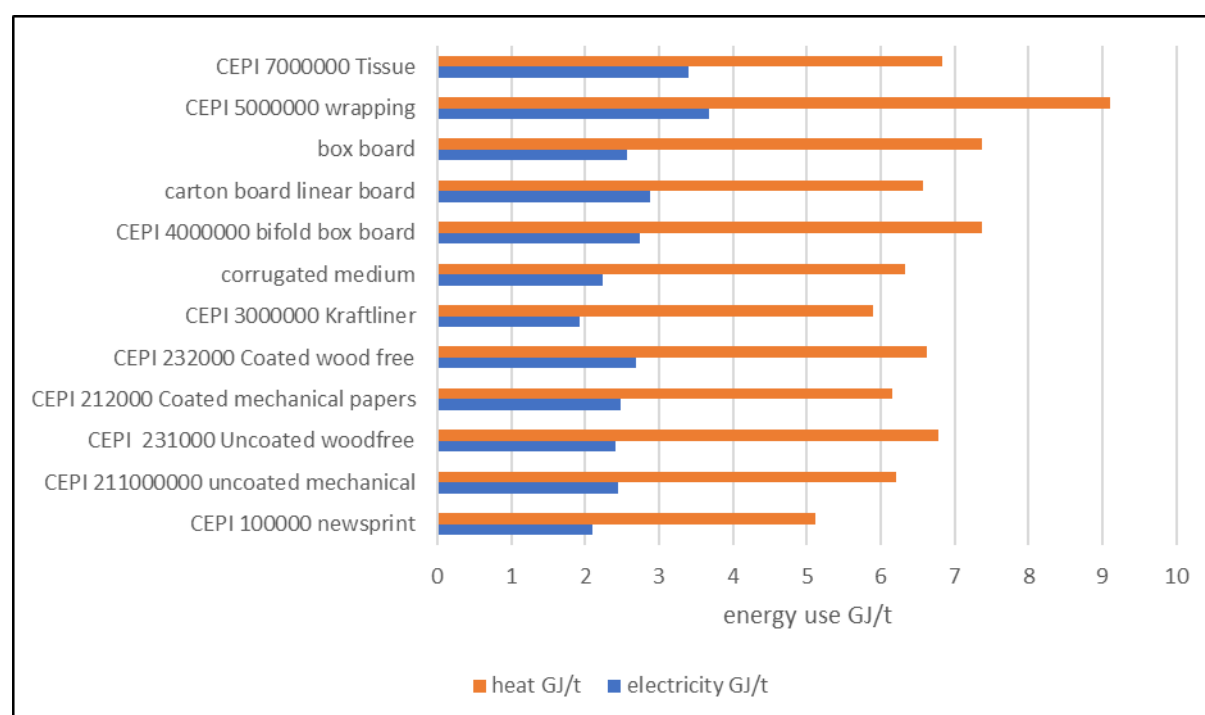
Fig.4. Process energy requirements for different grades of product produced by non-integrated mills.
