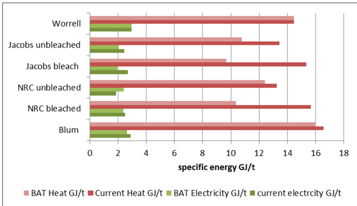
Fig. 6. Comparisons of current and BAT values for Kraft pulping
