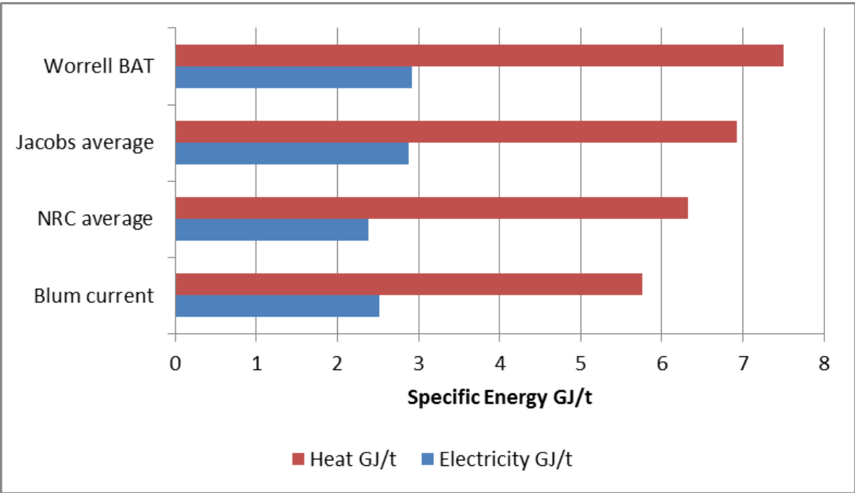
Fig 1. Specific energy requirement for non-integrated wood-free coated paper
