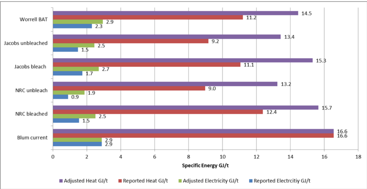
Fig. 2. Specific energy requirement in Kraft pulping mills
