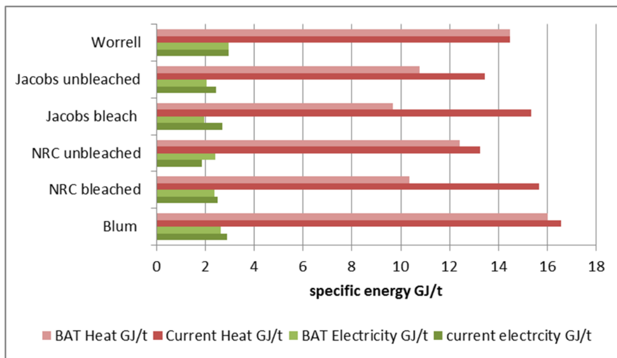
Fig. 7. Comparisons of current and BAT values for non-integrated wood-free coated paper mills
