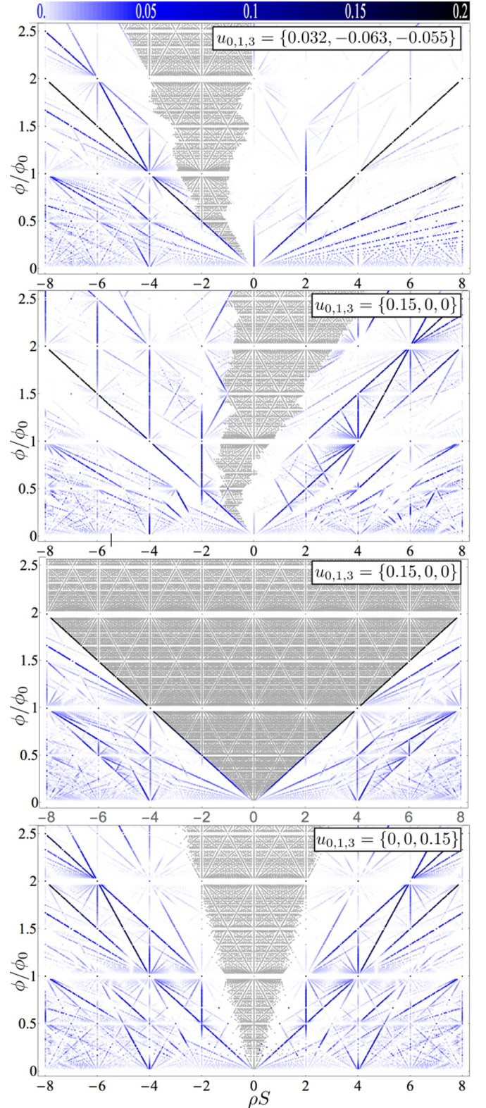
FIG. 4. The evolution of energy gaps in the magnetic miniband spectrum as a function of density and magnetic flux, calculated for the same parameters as Fig. 1. Larger gaps are shown using a darker color, white represents a vanishing gap, and gray represents the particular gapless states associated with the zero-energy LL.
