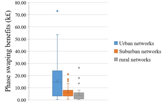
Fig. 8 Practical benefits from phase swapping
