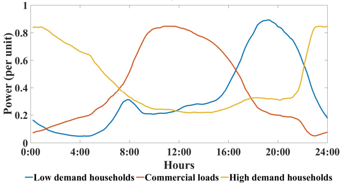
Fig. 6 Average weekday profiles of constituent loads
