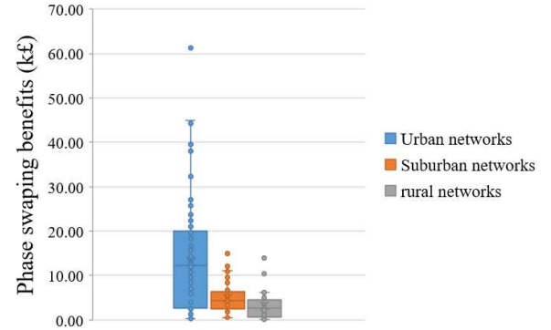
Fig. 5 Practical benefits from phase swapping
