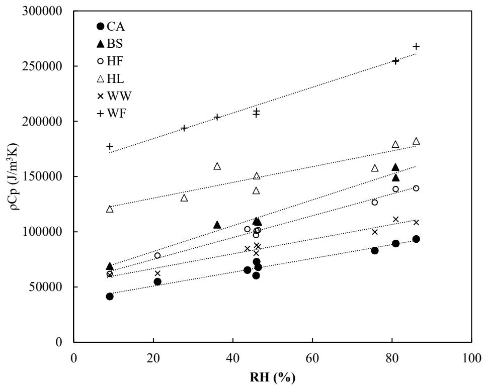
Figure 2. Variation of the product \rho C_p with relative humidity for the six samples. Experimental results are linearly fitted.
