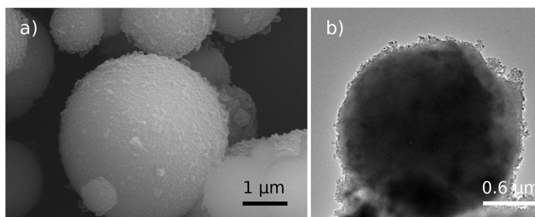
Figure 1 FESEM (a) and TEM (b) micrographs of the \text{Ti}_{\text{sph}} as-prepared powder.
