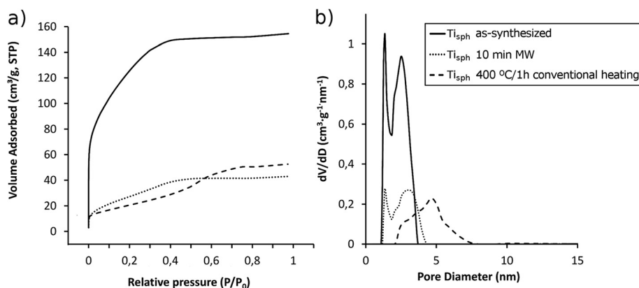
Figure 4 Nitrogen adsorption-desorption BET isotherms (a) and pore size distribution curves (b).
