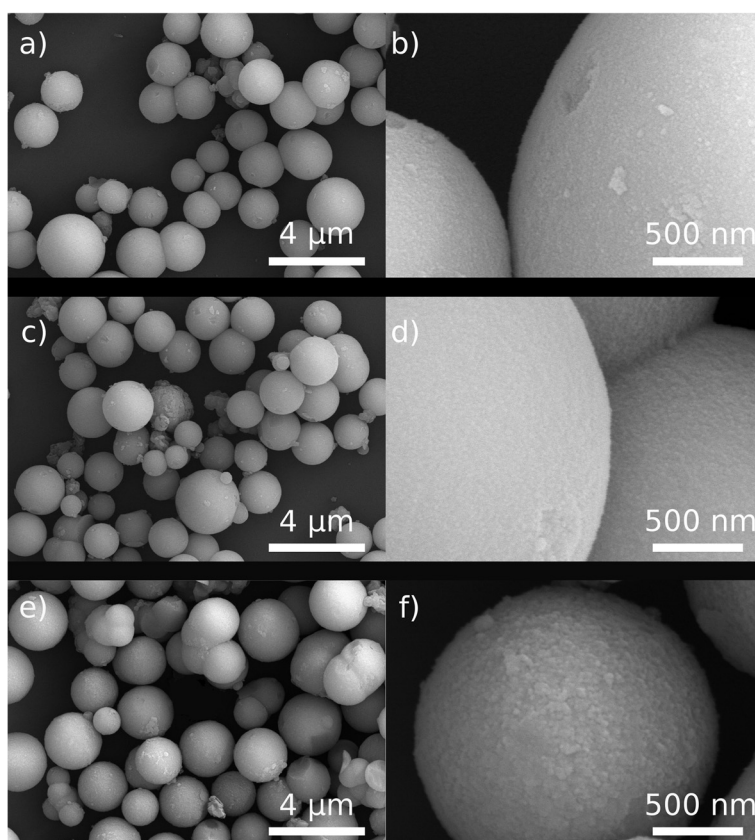
Figure 3 FESEM micrographs of the \text{Ti}_{\text{sph}} powder. After being exposed to different thermal treatments, 7 min under MW radiation (a, b), 15 min under MW radiation (c, d) and 1 h of conventional electric heating at 400°C (e, f).
