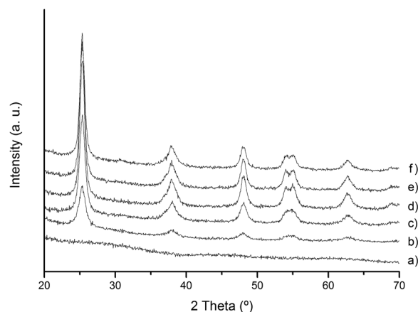
Figure 2 X-ray diffractograms. Of as-synthesized \text{Ti}_{\text{sph}} powder (curve a) and after 7 min (curve b), 10 min (curve c), 15 min (curve d) and 30 min (curve e) of MW treatment. XRD of the same powder treated at 400°C/1 h in a conventional electric furnace (f). All peaks corresponding to \text{TiO}_2 anatase (JCPDS file no. 21-1272).
