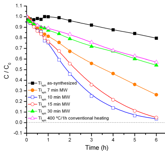
Figure 5 Evolution of methyl orange concentration during the photocatalytic test.
