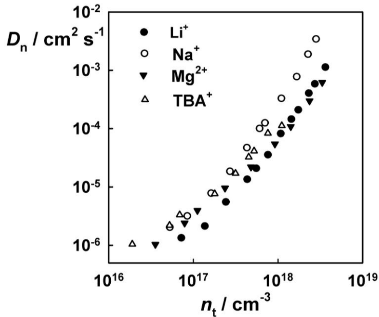
Figure 6. Effective electron diffusion coefficients measured for DSCs with different cations as a function of concentration of trapped electrons. Note that the plots should coincide if the trap distribution is independent of the cations.
