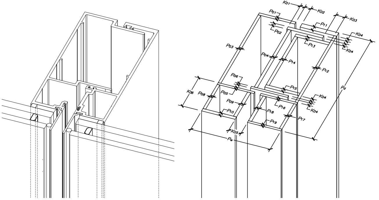
Figure 2: The male and female extrusions (Left), together, form a unitized curtain wall’s split mullion. In the idealized model of the mullion extrusions (Right), the P series of dimensions can be modified parametrically. Other input parameters control whether the elements labelled P_{04} , P_{09} , and P_{18} , as well as the group of elements labelled P_{13} , P_{14} , and P_{15} , are included in the model.
