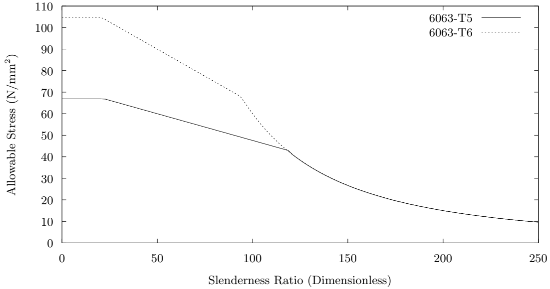
Figure 18: Maximum allowable bending stress, determined by the method set out in the Aluminum Design Manual [21], plotted with respect to slenderness.
