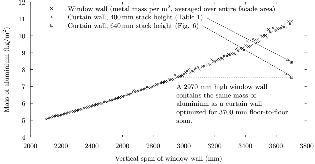
Figure 14: Relationship between mass of aluminium and height of window wall. The mass of metal in this study’s reference curtain wall system (Figure 4) is shown for comparison. Also shown is the mass of metal in a modified version of the reference wall, in which the mullion’s support bracket is positioned at the optimal distance from the top of the panel.
