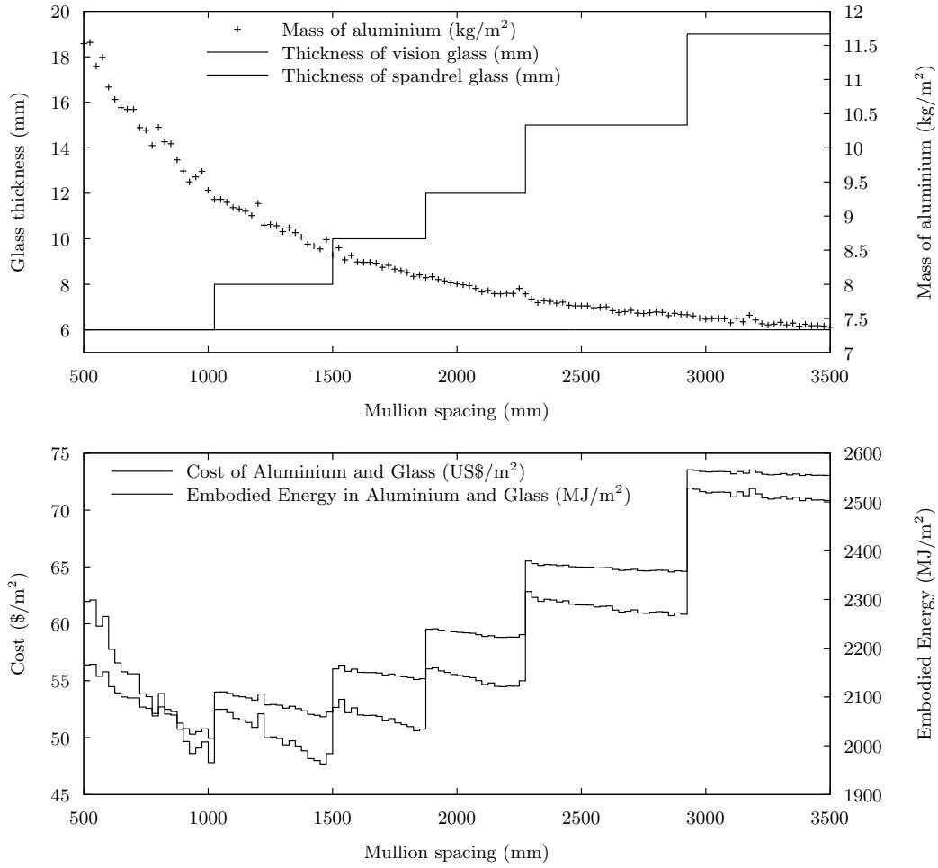
Figure 10: The upper graph shows how the mass of aluminium in an optimized curtain wall, and the thickness of its vision and spandrel glass, change with the horizontal spacing between mullions. The lower graph shows the approximate combined cost, and the approximate combined embodied energy, of the aluminium and glass.
