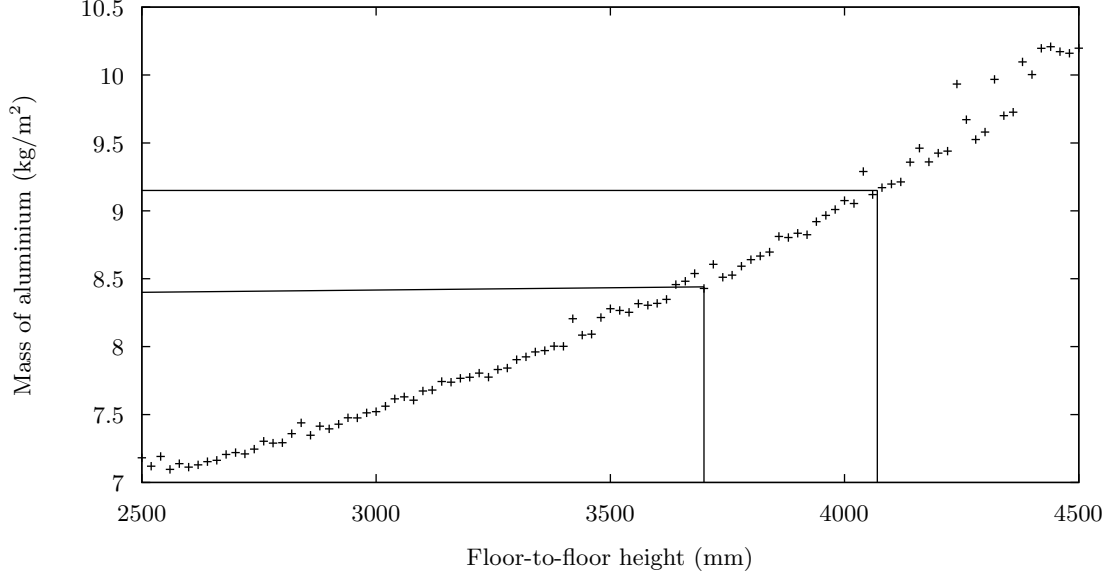
Figure 5: Influence of floor-to-floor height upon the mass of metal per unit area of optimized curtain wall.
