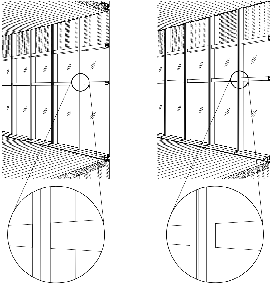
Figure 16: Two unitized curtain walls viewed from the interior side. In one (left), mullions and transoms are of uniform size, in the other (right) transoms are recessed. Aesthetically, the difference between the two designs is minor. Suspended ceilings, spandrel insulation and fire barriers have been omitted from the drawing for clarity.
