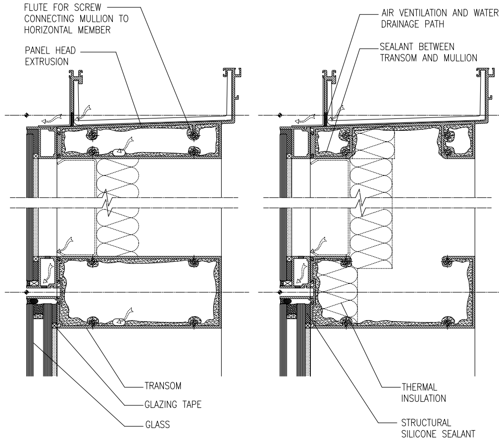
Figure 19: The unitized curtain wall head and transom members on the left are conventional, boxed designs. Those on the right are open sections, requiring less metal.
