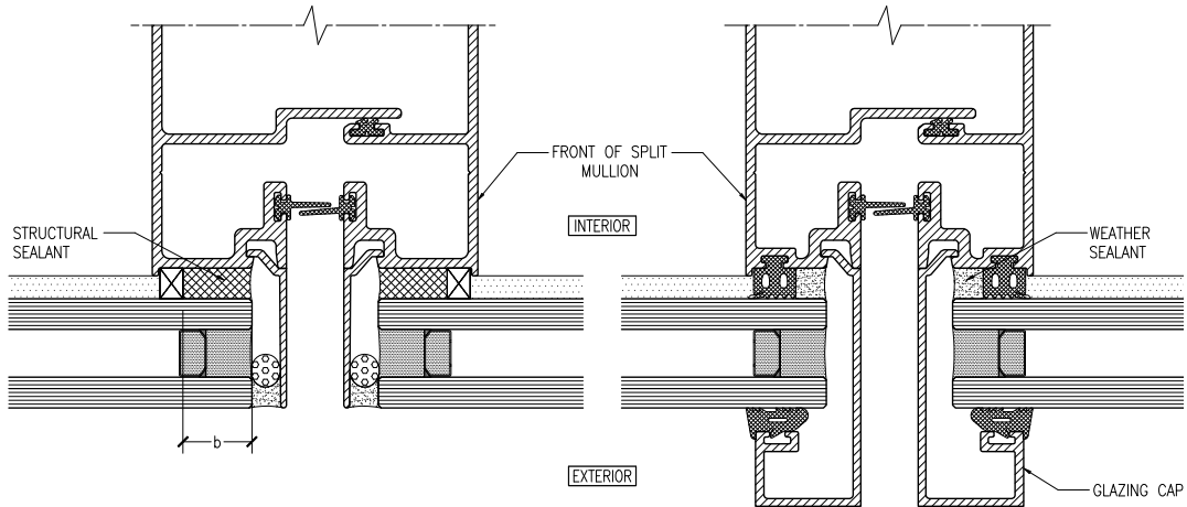
Figure 17: A split mullion with seamless, structural silicone glazing (left), and with capped glazing (right).
