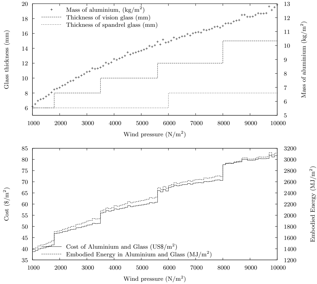
Figure 11: Upper graph shows the effect that variation in design wind load has upon mass of aluminium and thickness of glass in an optimized curtain wall system. Lower graph shows the effect upon and material cost and embodied energy.
