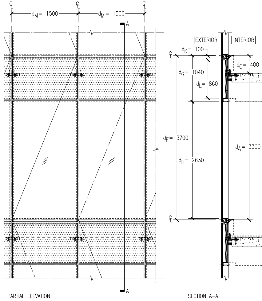
Figure 4: Dimensioned elevation and section views showing the layout of the normative reference curtain wall considered in the numerical optimization studies. The vertical distance between the fulcrum of the bracket and the fulcrum of the stack joint, d_C , is the “stack-height”.
