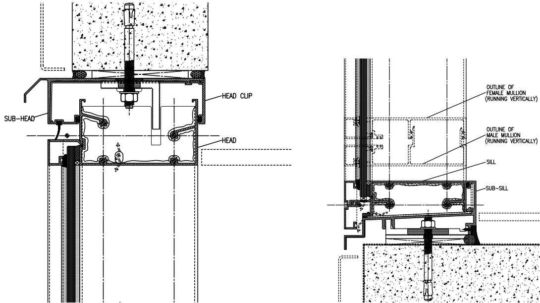
Figure 13: Cross-sectional form of horizontal members in a window wall: the sub-head and head (left), and the sill and sub-sill (right). An outline of the vertical mullion is shown above the sill.
