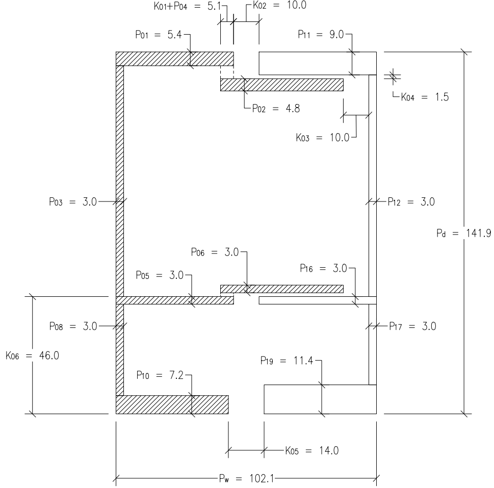
Figure 3: Shapes of the mullion profiles optimized to meet the performance criteria set out in Table 1, and the facade layout geometry shown in Figure 4. Dimensions are in millimeters.
