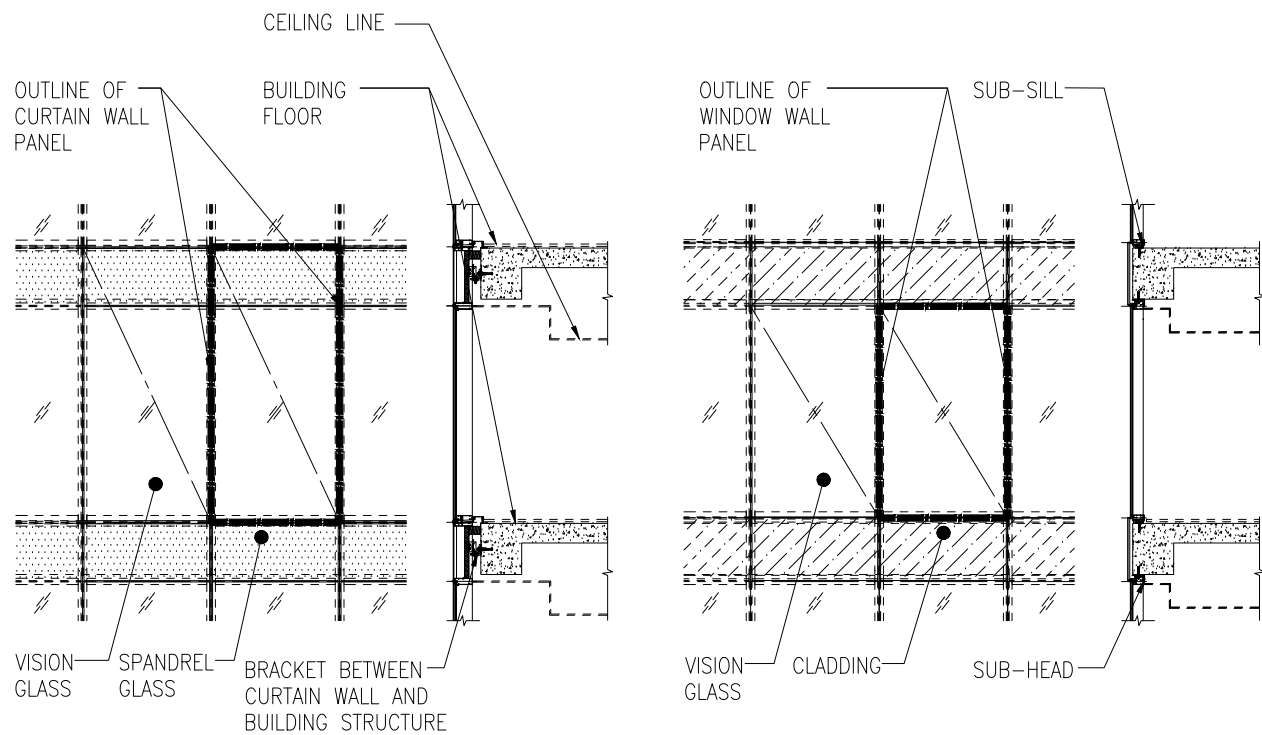
Figure 12: Elevation and section views of a curtain wall (left), and a window wall (right). In the elevation views, panel sizes are indicated with a heavy, broken line.
