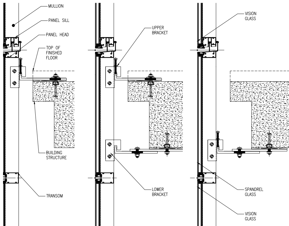
Figure 15: A top-of-slab mullion bracket (left), double bracket (centre) and underside bracket (right).
