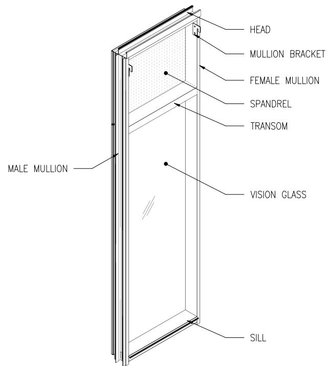
Figure 1: Parts of a unitized curtain wall panel for a flat facade, viewed from the side facing the interior of the building. For clarity, cosmetic trims, insulation, and barriers preventing the spread of fire and smoke, are omitted from this diagram.
