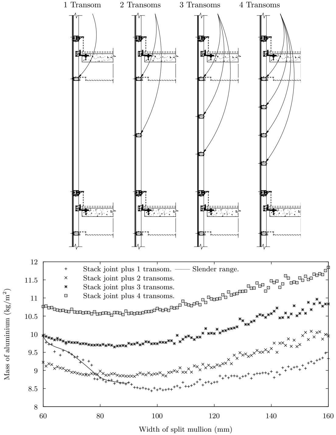
Figure 7: Plot (bottom) shows variation in mass of aluminium with mullion width, for four different curtain wall panel configurations (above). Other than the number of their transoms, panels are the same as those shown in Figure 4. The solid line on the graph is a moving mean mass of metal for panels with one transom, in which the mullion is slender and lateral torsional buckling is the governing structural design consideration. At high slenderness ratios, the mullion cross-sections are inefficient: if mullion width is narrower than 80 mm then a panel with two transoms requires less aluminium than in a panel with one transom.
