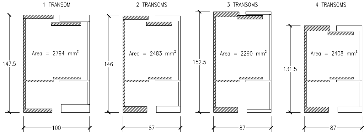
Figure 8: Mullions optimized for four different curtain wall panels – those shown in the upper diagram of Figure 7 – each with a different number of transoms. Dimensions are in millimeters. The slight gaps in between rectangular elements in the male profile’s flanges and, in the case of the three-transom mullion, the small area of overlap between adjacent elements, are consequences of the geometric simplifications made during the design of the parametric model.
