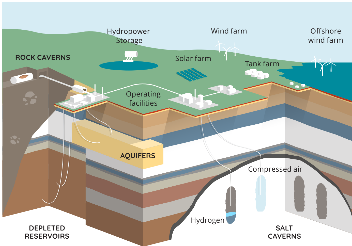
Hydrogen storage in salt caverns [34].
