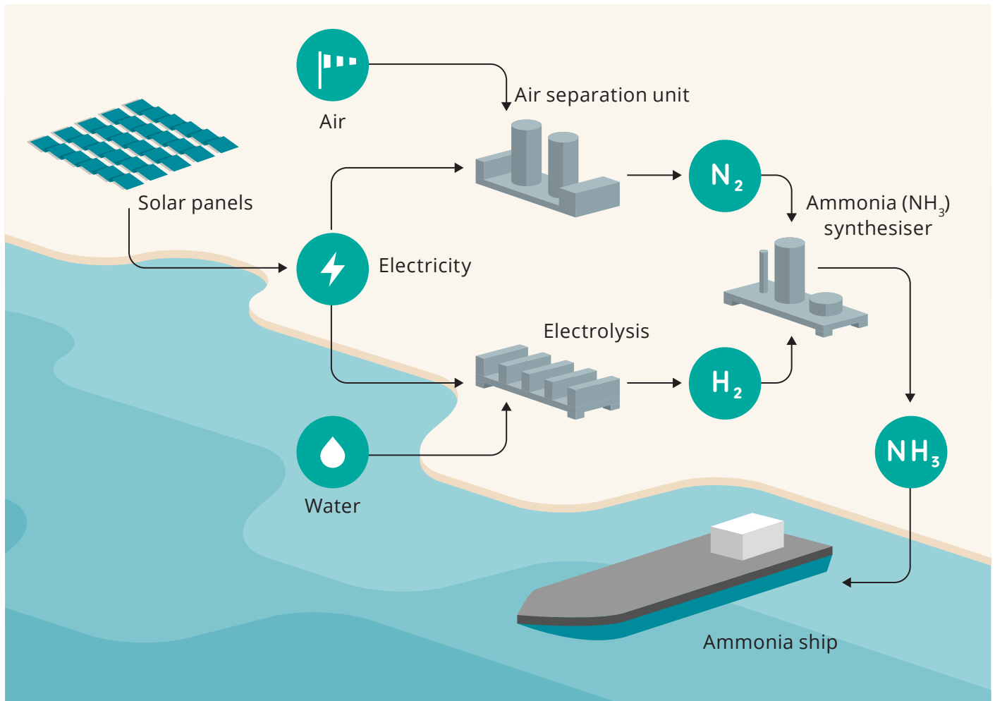
Solar-hydrogen-ammonia cycle [30].
