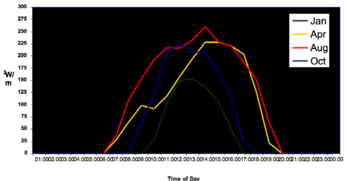
Figure 2.11 – Hourly Average Solar Radiation – Dublin ( \text{W/m}^2 )
