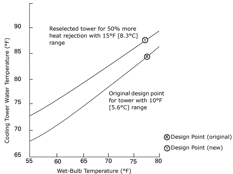
Figure 22. Cooling tower re-selection with different chiller capacities
