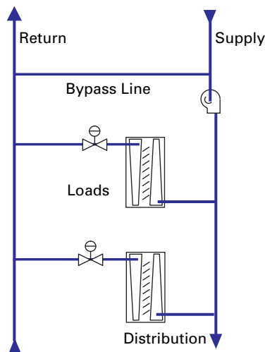
Figure 30. Distribution loop
