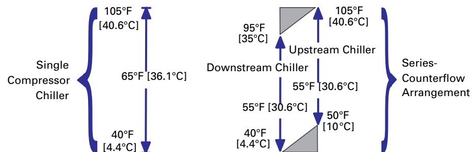
Figure 49. Equal lift concept
