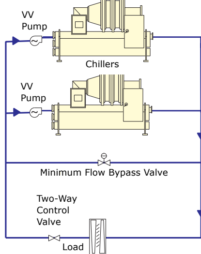
Figure 14. Variable-primary system
