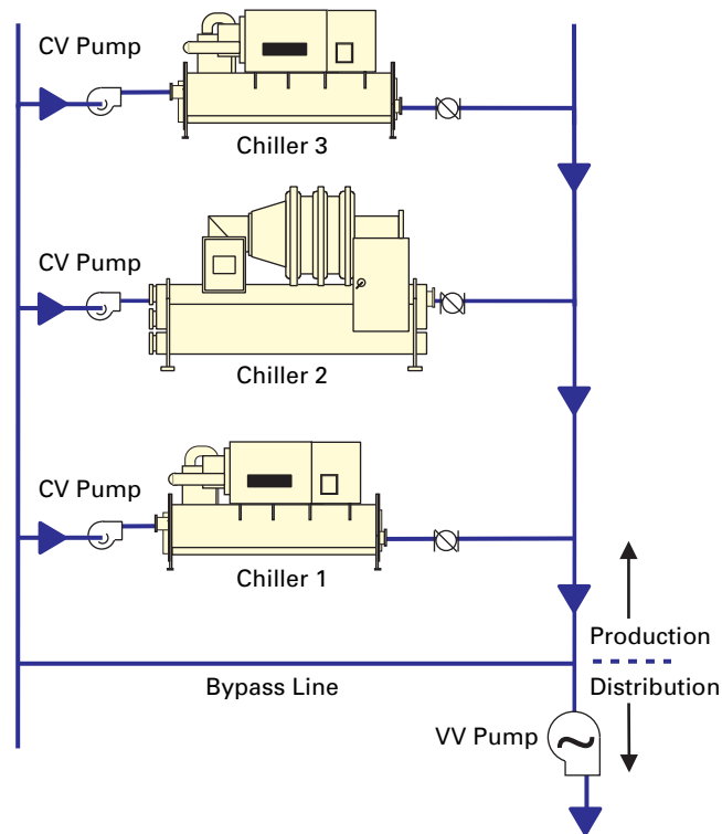
Figure 28. Decoupled arrangement
