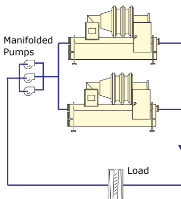
Figure 10. Manifolded pumps
